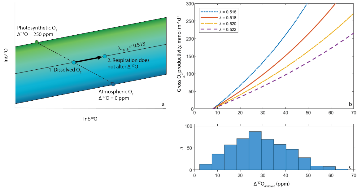
Figure 1: (a) Schematic (after Juranek and Quay) 21 showing how dissolved O 2 Δ 17 O can be a mixture of endmember atmospheric and photosynthetic O 2 compositions, and respiration fractionation that assumes \lambda_{17/18} will preserve Δ 17 O. (b) Calculated GOP plotted against Δ 17 O value for different \lambda values using the method of Prokopenko et al. 22 and photosynthetic O 2 from average marine phytoplankton according to Luz and Barkan 61 assuming \delta^{18}\text{O}_{\text{O}_2} = 0.73\text{‰} , k = 3 \text{ m d}^{-1} , and [\text{O}_2]_{\text{eq}} = 230 \text{ mol m}^{-3} . (c) Histogram of Δ 17 O data from Reuer et al. 49
