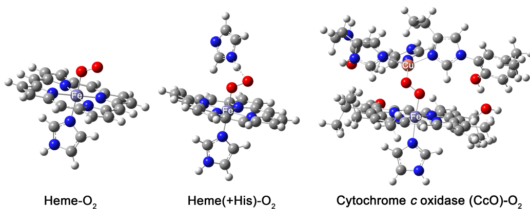
Figure 3. Oxyheme models used in this study. White atoms are hydrogen, grey atoms are carbon, blue atoms are nitrogen, and red atoms are oxygen. Transition-metal atoms (Fe, in lavender, and Cu, in orange) are labeled.
