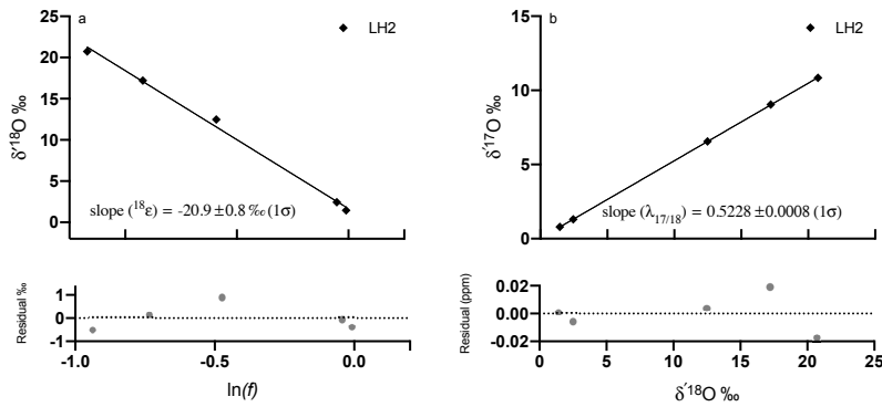
Figure 6. LH2 data are shown as a representative example of the evolution of \delta^{18}\text{O} vs. the natural log of the fraction of \text{O}_2 remaining (a). The linear regression slope of this line is {}^{18}\epsilon . Panel (b) shows the co-variation in \delta^{17}\text{O} vs \delta^{18}\text{O} , and the linear regression slope of this line is \lambda_{17/18} . Residuals for these regressions are shown in the bottom of each panel.
