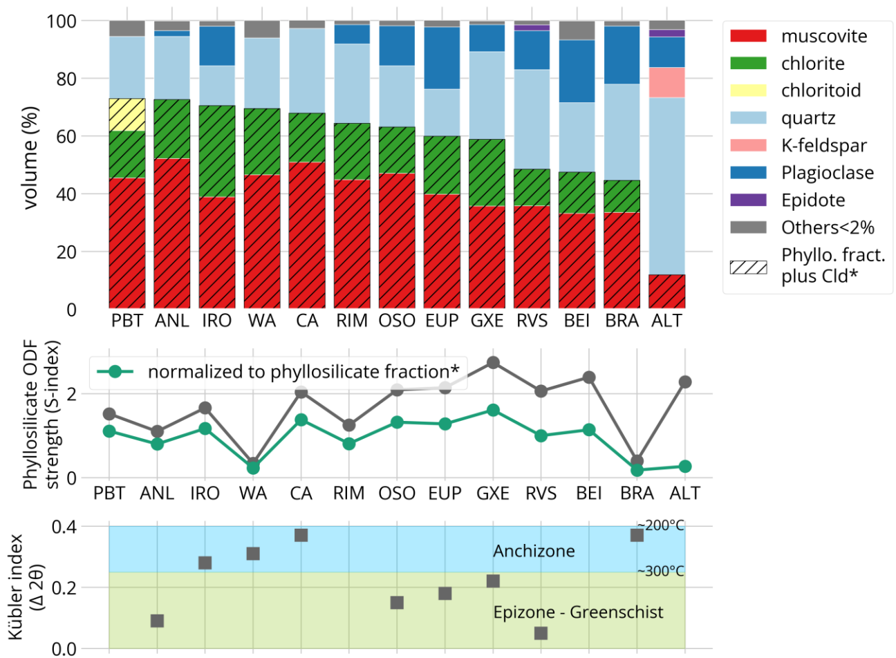
Figure 1. Mineral composition, phyllosilicate preferred orientation, and degree of metamorphism. (a) Volumetric contribution of the major mineral phases estimated using large-coverage EDS chemical maps. The hatched area represents the volumetric contribution of the phyllosilicates excepting in sample PBT where chloritoid (11.1 %) is also included (see section 3.2 for details). Sample ALT is a micaceous quartzite with 11.9 % of micas. The remaining samples are single-foliated slates with phyllosilicate content varying between 72.6 and 44.6 %. Only mineral phases above 2 % are considered for computing seismic properties. A table with volume fraction values is provided in the Supplementary Material as Table S4. (b) Phyllosilicate CPO intensity, measured by the S-index (orientation entropy in Euler space), both raw and normalised to the total phyllosilicate fraction (Table S5). (c) The degree of metamorphism for most of the slates using the Kübler index (illite crystallinity) (Table 1).
