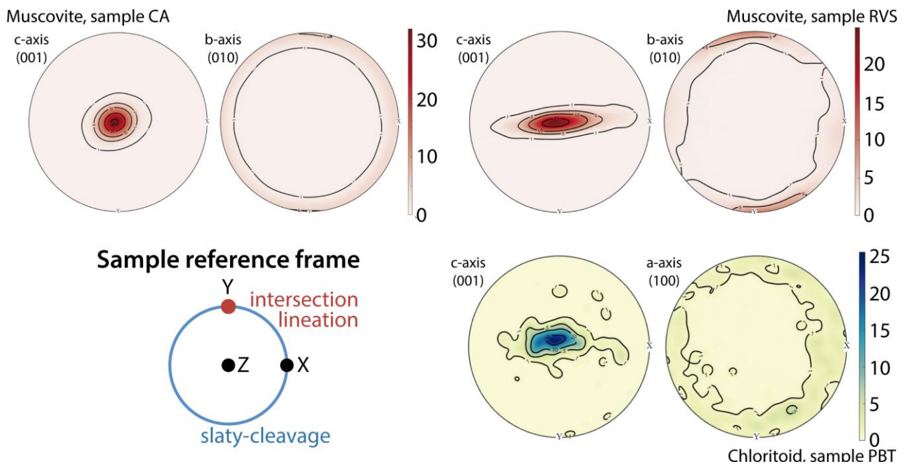
Figure 2. Typical CPO patterns in the studied samples. Upper row: Typical phyllosilicate (muscovite and chlorite) CPOs in slates. On the left, the c-axis forms a point maximum normal to the foliation, and the b- and a-axes are oriented randomly within the foliation (samples ALT, ANL, BEI, BRA, CA, EUP, GXE, OSO, WA). On the right, the c-axis forms a semi-girdle with a point maximum normal to the foliation and spreads perpendicular to the intersection lineation. The a- and b-axes are oriented with the foliation, showing a complete girdle with a maximum parallel to the intersection lineation (samples RVS, PBT, RIM). Bottom row: On the left is the reference frame of the sample with respect to the pole figure. On the right, the chloritoid CPO pattern in the PBT sample showing a similarity with the phyllosilicate CPO patterns with the c-axis arranged normal to the foliation and the a- and b-axes oriented randomly within the foliation. Upper hemisphere equal-area projections, contours in multiples of a uniform distribution. All CPO pole figures are provided in the Supplementary Material.
