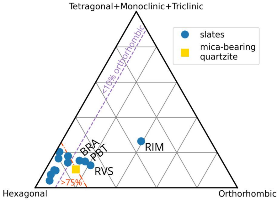
Figure 7. Decomposition analysis of the calculated elastic tensors (geometric mean) illustrating the proportion of hexagonal to orthorhombic to lower symmetry components for all the samples. The purple dashed line indicates the <10 % orthorhombic symmetry threshold, while the orange dash-dotted line indicates the >75 % hexagonal symmetry threshold. Slates outside these thresholds are labelled.
