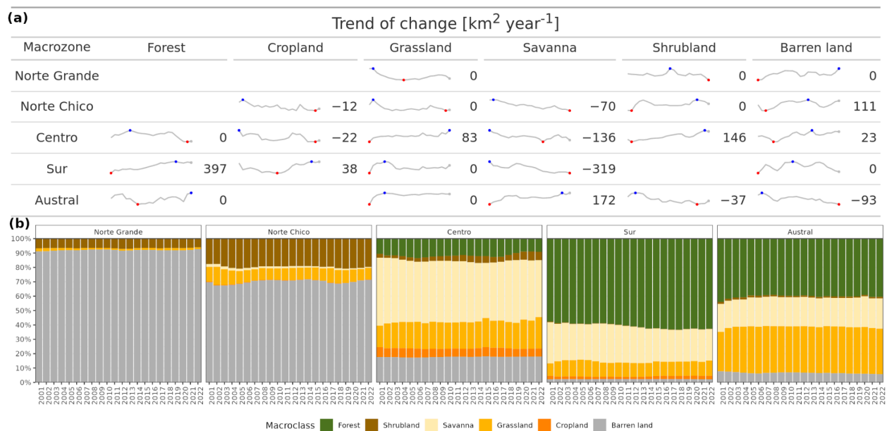
Figure 3. Land cover is shifting dynamically across continental Chile. Temporal trends in absolute (a) and relative (b) land cover across continental Chile for 2001-2022. Temporal change in land cover for each class was estimated with Sen's slope; zero values indicate no change, while red and blue points indicate maximum and minimum values, respectively. Land cover classes with no values did not have statistically significant changes in area over the study period. Relative land cover change was estimated within each study region.
