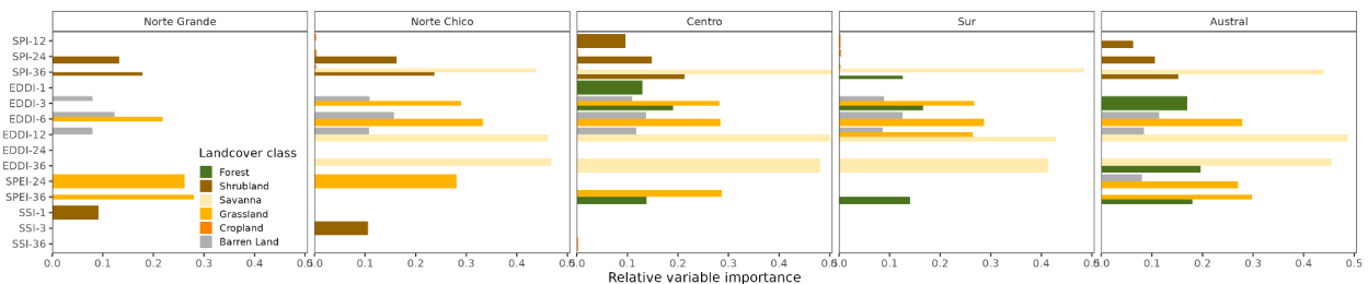
Figure 6. Shifts in water supply and demand drive land cover change across multiple time scales. Variable importance of multi-scalar drought indices for explaining land cover change in five study regions across continental Chile. Variable importance was estimated with Random Forest models fitted for each combination of study region and land cover type. SPI is the Standardized Precipitation index, SPEI is the Standardized Precipitation Evapotranspiration Index, SSI is the Standardized Soil Moisture Index, and EDDI is the Evaporative Demand Drought Index. The numbers next to the drought index correspond to the time scales in months (1- 36).
