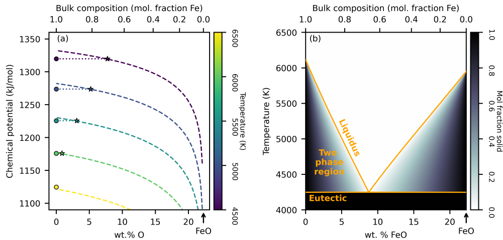
Figure 2. Equilibrium properties of the Fe-FeO system computed from [39] at 330 GPa. (a) The chemical potential of liquid FeO mixtures (dashed lines) and the pure solid Fe chemical potential (circles) coloured by temperature. Dotted tie lines connect solid Fe with the equilibrium liquid mixture for temperatures within the two phase region. At 6500 K solid Fe is unstable compared to a pure Fe liquid. (b) Calculated phase diagram where phase boundaries (liquidus and eutectic) are shown (orange lines) and the solid Fe – liquid FeO two-phase region relevant to our slurry model is labeled. The equilibrium solid fraction is indicated by the shading.
