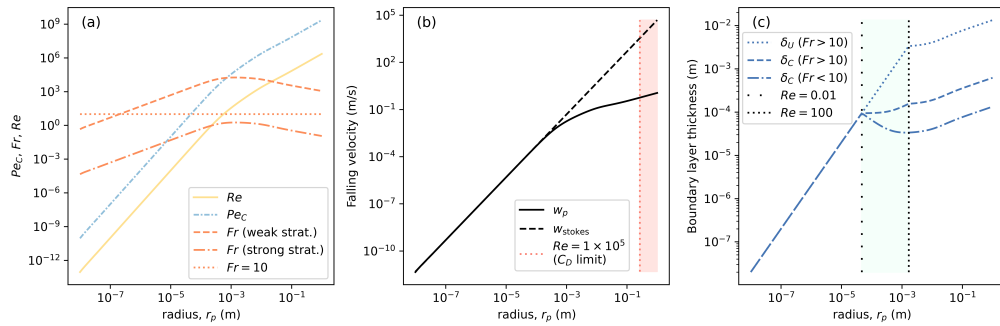
Figure 3. Dynamical regime, falling velocity and boundary layer thickness for a iron particle falling through a stratified liquid with parameters relevant to the F-layer ( \rho^S = 12700 \text{ kg m}^{-3} , \rho^L = 12100 \text{ kg m}^{-3} , g = 4.4 \text{ m s}^{-2} , D^L = 1 \times 10^{-9} \text{ m}^2 \text{ s}^{-1} and \nu^L = 1 \times 10^{-6} \text{ m}^2 \text{ s}^{-1} ). (a) Re (yellow) and Pe_C (blue) and Fr (orange, dashed for N_{BW} = 10^{-3} \text{ Hz} and dash-dots for N_{BW} = 10 \text{ Hz} ) are calculated self consistently and determine the dynamical regime, with Fr = 10 indicated. (b) Falling velocity (solid line) and Stokes velocity (dashed line) showing the divergence at larger particle radii. The vertical line and pink shading corresponds to Re \geq 3 \times 10^5 , the upper bound on the empirical scaling for the drag coefficient. (c) Momentum (dotted line) and chemical (dashed for N_{BW} = 10^{-3} and dash-dots for N_{BW} = 10 \text{ Hz} ) boundary layer thickness. Vertical dotted lines showing the intermediate and large Re regime transitions.
