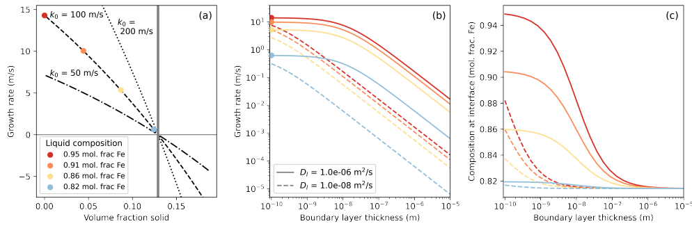
Figure 4. Calculated particle growth rate dr_p/dt for bulk composition X^{\text{tot}} = 5 mol. % O, T = 5000 K and P = 330 GPa. (a) shows dr_p/dt as a function of solid fraction \phi , neglecting boundary layer effects, using Equation 3.8. Vertical grey line denotes the equilibrium solid fraction at the chosen P - T - X^{\text{tot}} . Coloured symbols denote the liquid composition calculated from Equation 2.2 for the given \phi and X^{\text{tot}} . (b) and (c) show dr_p/dt and X(r_p) as a function of fixed boundary layer thickness using the four liquid compositions marked in (a) calculated with Equation 3.10. Two values of the oxygen diffusivity are shown in solid and dashed lines. All coloured cases have k_0 set to 100 m/s.
