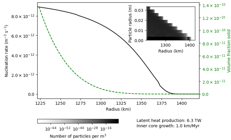
Figure 7. Key results from a slurry model of the F-layer with temperature and compositional profiles as shown in 1(c), D^L = 1 \times 10^{-9} \text{ m}^2 \text{ s}^{-1} , \nu^L = 2 \times 10^{-6} \text{ m}^2/\text{s} (corresponding to the light blue square in in Figure 5) and I_0 = 1 \times 10^{-11} \text{ s}^{-1} \text{ m}^{-3} . The main panel shows the calculated nucleation rate (black) and volume fraction solid (green), which both increase downwards as the under-cooling increases. Nucleation starts close to R = 1375 \text{ km} where the temperature profile drops sufficiently below the liquidus (see Figure 1), but the very low undercooling results in such small nucleation and growth rates that the volume fraction solid remains effectively zero until R = 1275 \text{ km} where the under-cooling becomes much more significant. The inset histogram of the number density of particles of different sizes as a function of depth reveals that once particles start to grow they grow steadily with the largest particles found just above the ICB. However, small particles that have not yet grown enough to fall quickly continue to dominate the particle size distribution throughout the layer.
