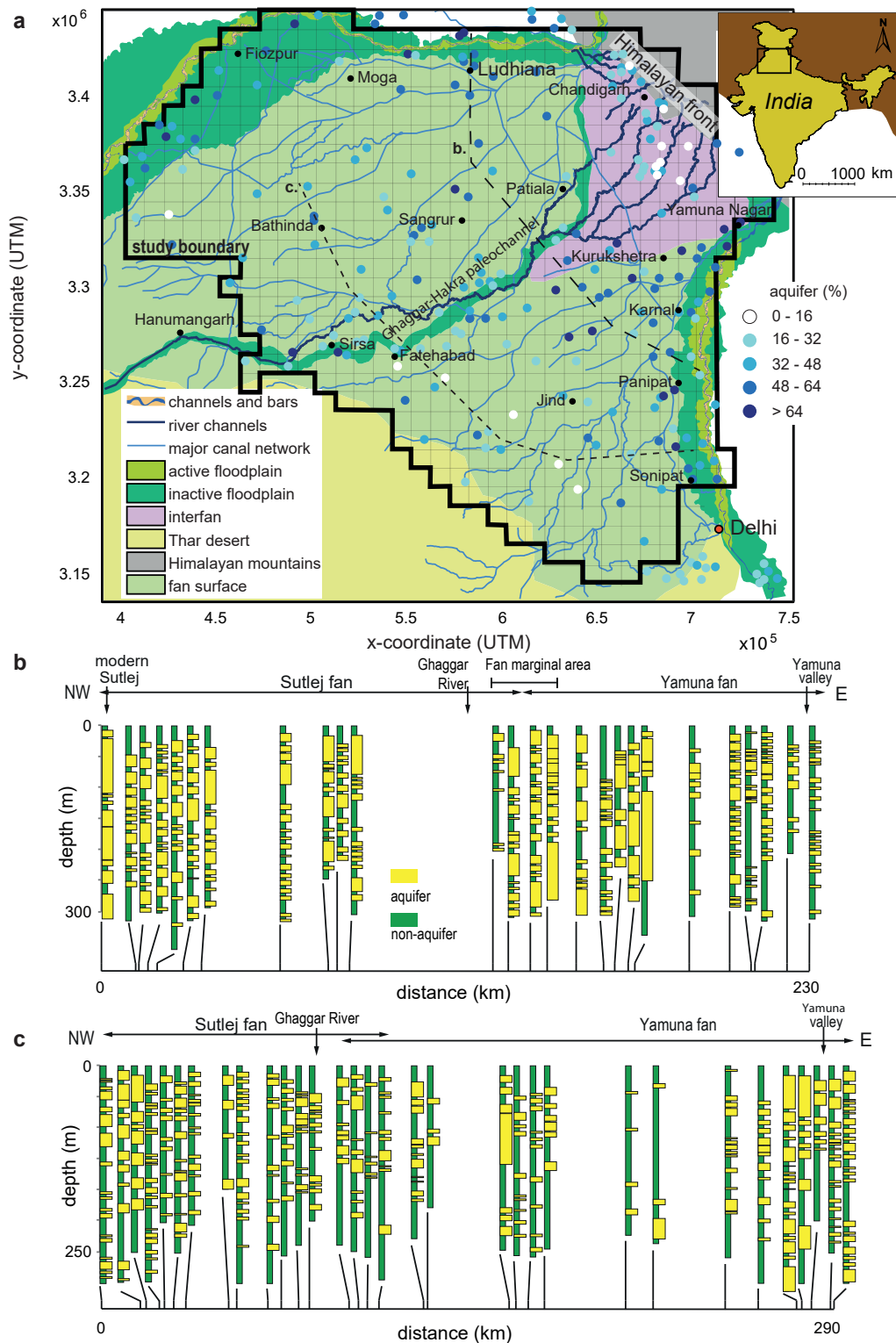
Figure 1: a) Geomorphological map and the subsurface aquifer percentage of the study area in northwestern India, modified after Van Dijk et al. (2016a). The study area covers the Sulej and Yamuna fans (light green) and the interfan area between them (pink). Dark green areas show the incised valleys of the modern Sulej and Yamuna rivers and the Ghaggar-Hakra paleochannel (Singh et al., 2017). Light blue lines show major canals. Dots show bulk aquifer percentage in the upper 200 m of the subsurface, based on CGWB aquifer-thickness logs (see Van Dijk et al. (2016a) for description). Long-dashed line shows the medial transect in panel (b), while the short-dashed line shows the distal transect in panel (c). The study area is outlined by the thick black line and divided into 10 x 10 km grid cells. b) Medial transect illustrating aquifer (yellow) and non-aquifer (green) units in the subsurface. Note abundant stacked aquifer bodies. c) Distal transect showing the lower abundance of aquifer bodies compared to the medial part of the fan. Transects in panels (b) and (c) modified from Van Dijk et al. (2016a).
