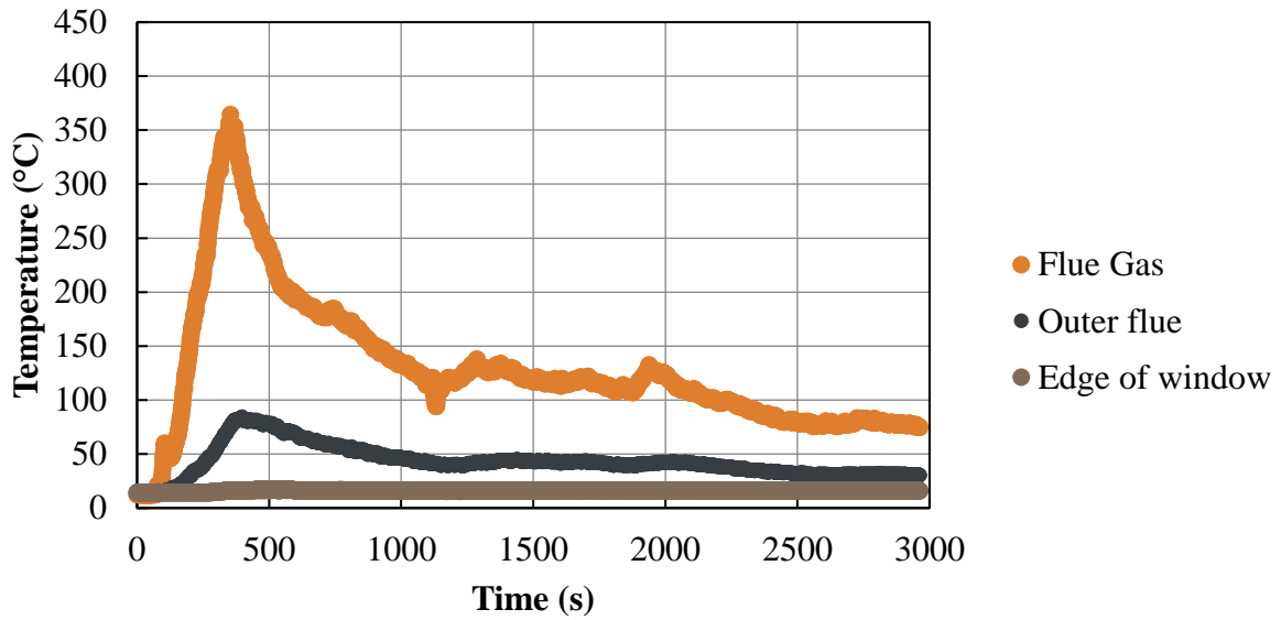
Figure 5. Temperature readings during test 2 (burning with the door open and the door opening covered).
