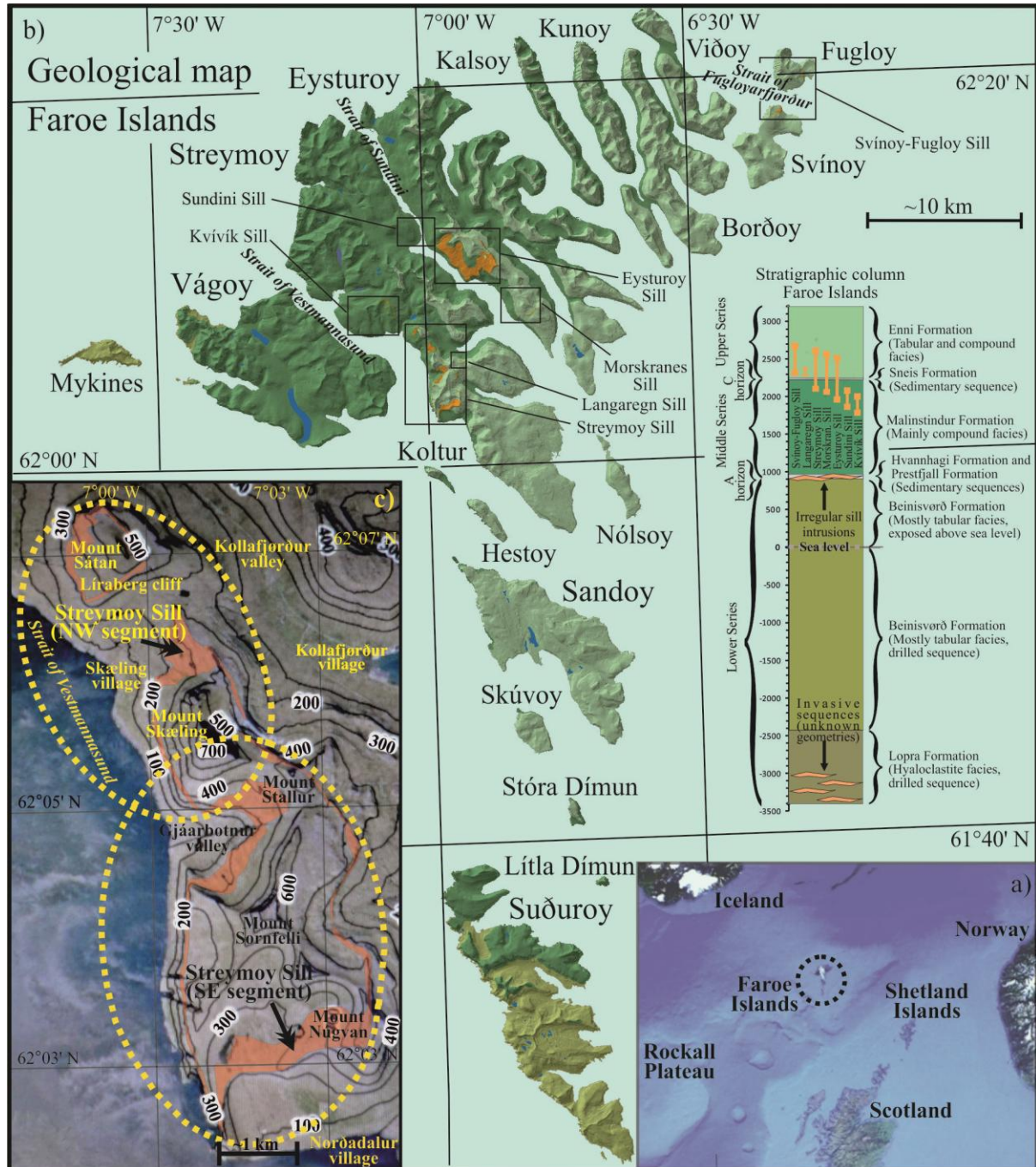
Figure 1. Modified from Hansen et al. (2019). a) Map of the North Atlantic area showing the relative location of the Faroe Islands. Basic image from Google Earth. b) Geological map of the Faroe Islands. Older nomenclature is indicated to the right of the stratigraphic column and a more recent nomenclature is shown to the left. Vertical extents of sills are indicated by orange bars in stratigraphic column. Topographic and other map data originate from Munin.Fo, Faroe Islands. c) The map shows the two segments making up the Strey moy Sill, where sill outcrops are indicated in orange colour. Numbers on topographic contours indicate metres. Basic image from Kortal.Fo, Faroe Islands.
