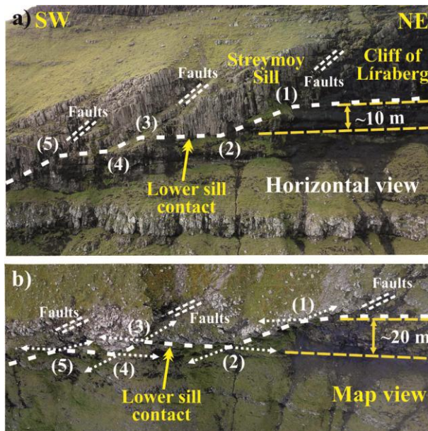
Figure 7. Part of the Streymoy Sill, NW segment, cropping out at the cliff of Líraberg (see also Fig. 4a). Lower sill contacts are indicated with white dashed lines. High-resolution drone-based images building up these two main composite images were provided by Magnus Pauli Joensen, Faroe Islands. Estimated initial magma propagation/climbing directions in this area are indicated in Fig. 4a. a) Image, taken horizontally roughly orthogonal to the cliff face, showing apparent ramp – flat geometries at the lower sill contact. Intersections between ramps and flats are numbered. b) Same as in a), but taken vertically downwards (map view). Extrapolated directions of individual numbered basal sill sections are indicated with small white dotted arrows.
