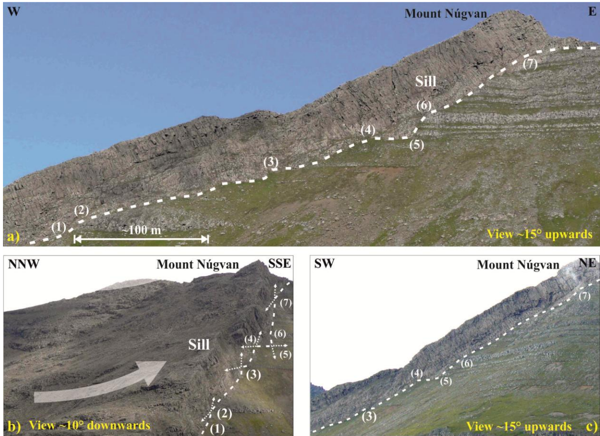
Figure 6. Part of the Strey moy Sill, SE segment, which crops out at Mount Nógvan (see also Fig. 3a). Lower sill contacts are indicated with dashed white lines. a) Image, taken roughly orthogonal to the cliff face, but at a slight upwards angle and showing apparent irregular (ramp – flat) geometry at lower sill contact. Most intersections are numbered. b) Same as in a), but taken slightly downwards and at a narrow lateral angle with the cliff face. Large white arrow indicates the most probable propagation direction of initial sill magmas. Extrapolated directions of individual sill base sections are indicated with small white dotted arrows. c) Same as in a) and b), but taken at a slight upwards angle and a lateral angle of around 30° with the cliff face.
