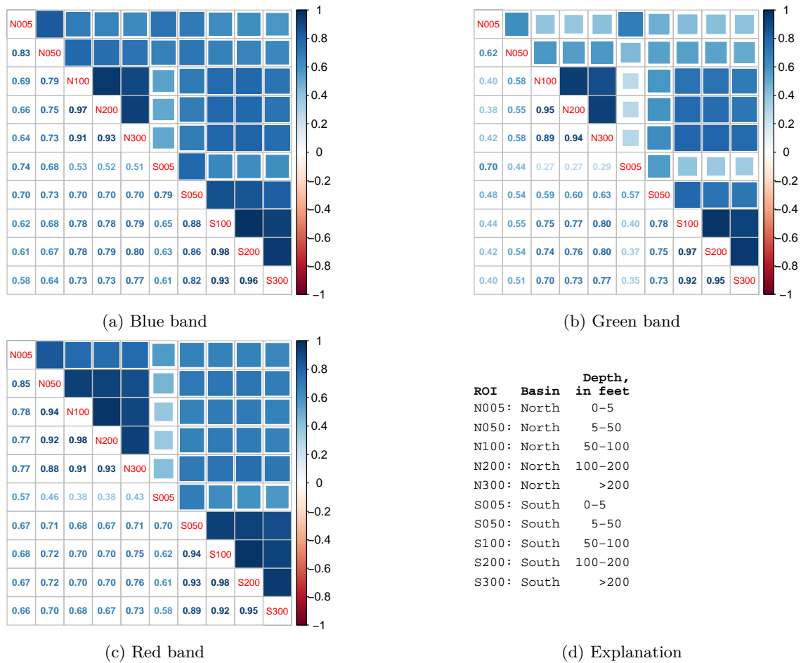
Figure 19. Spatial Correlation of generalized additive modelling errors by basin and water-depth interval for Torch Lake, Michigan
