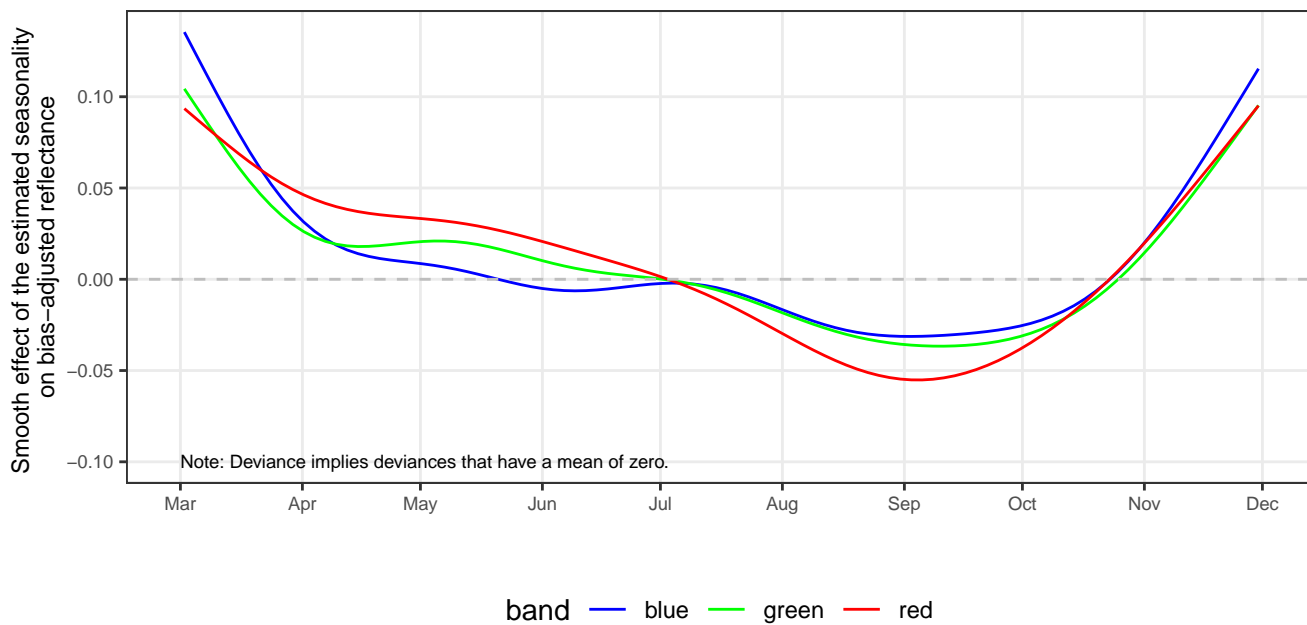
Figure 17. Seasonality of Grand Traverse Bay surface reflectances by band color
