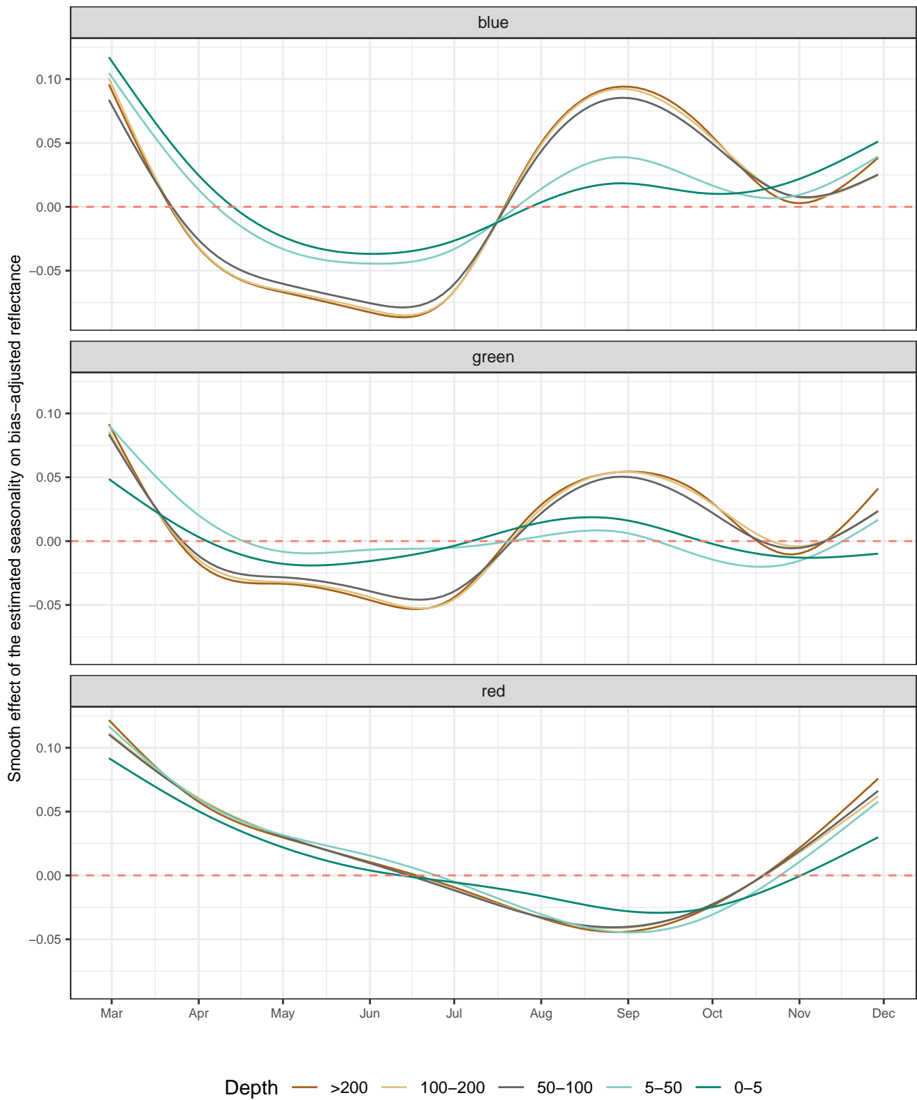
Figure 9. Seasonal components of generalized additive model of visible light in the blue, green, and red bands from Torch Lake in Antrim County, Michigan
