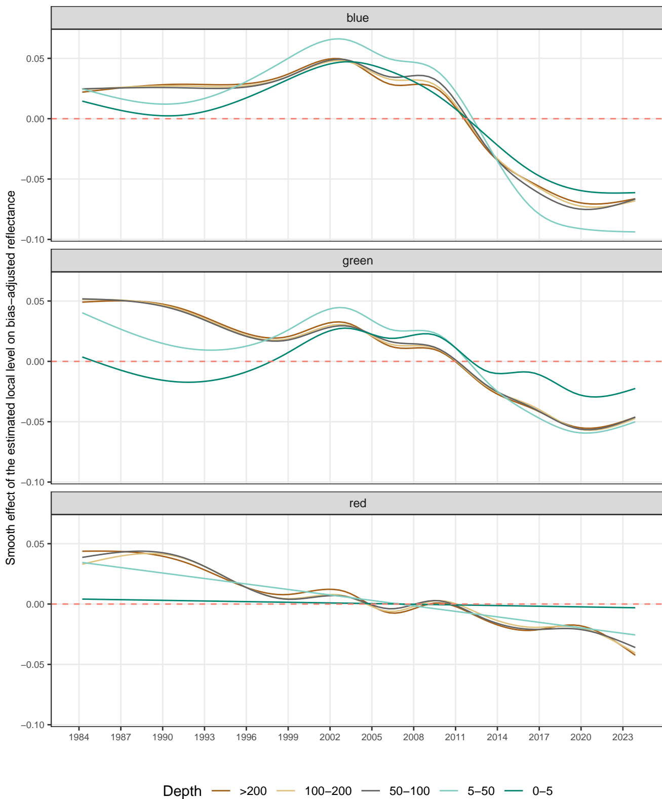
Figure 11. Local level deviances from zero mean in blue, green, and red bands of visible light during open-water periods from 1984 through 2023 on Torch Lake in Antrim County, Michigan
