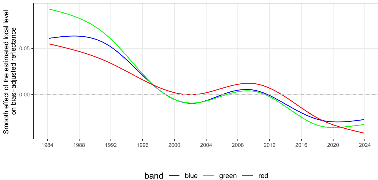
Figure 18. Local levels of Grand Traverse Bay surface reflectances by band color
