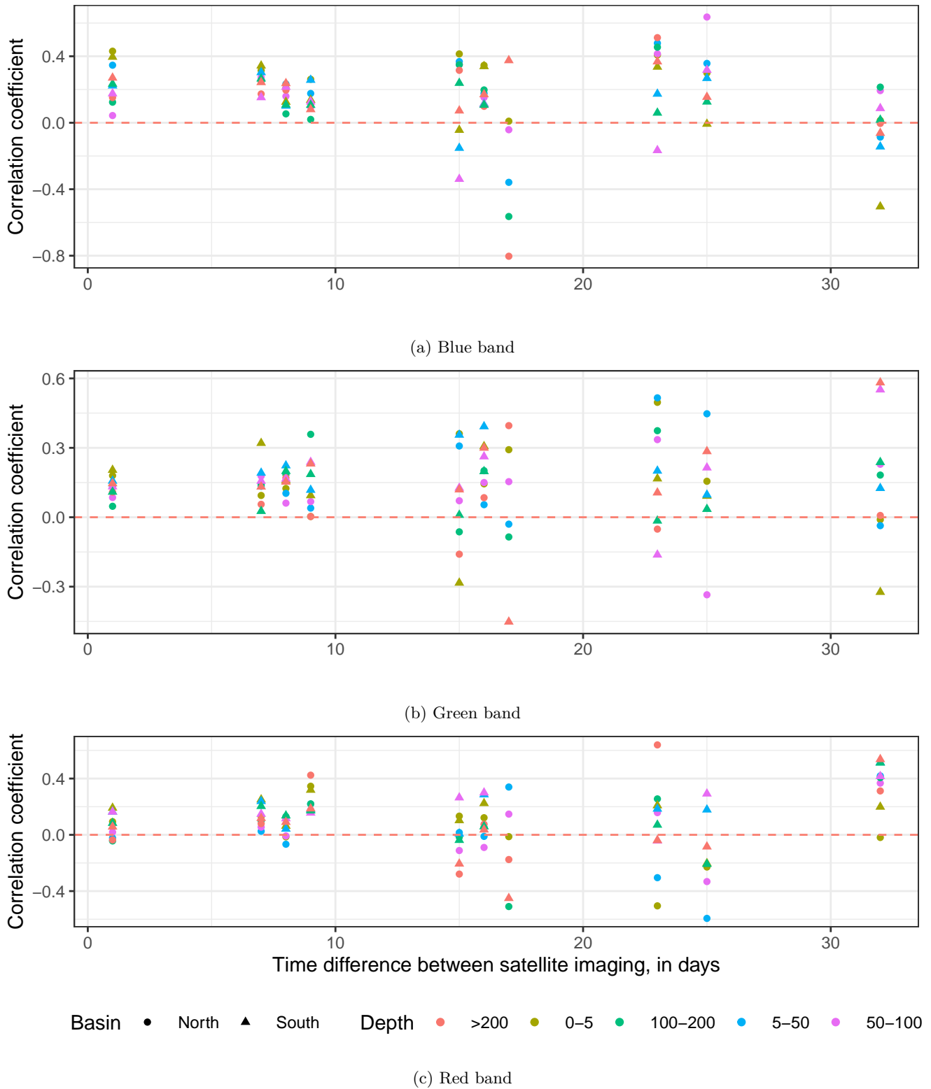
Figure 20. Autocorrelation functions of generalized additive modelling errors by basin and water-depth interval for Torch Lake, Michigan
