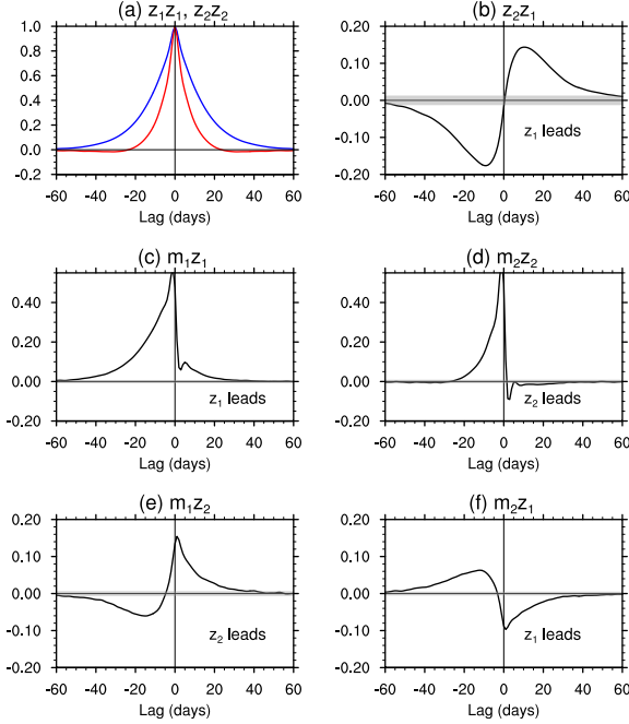
FIG. 10. Lagged-correlation analysis of synthetic data with cross-EOF feedback. (a) Auto-correlation of z_1 (blue) and z_2 (red), (b) cross-correlation z_1z_2 , (c) cross-correlation m_1z_1 , (d) cross-correlation m_2z_2 , (e) cross-correlation m_1z_2 , and (f) cross-correlation m_2z_1 . The e -folding decorrelation time scales of z_1 and z_2 are 13.9 and 6.5 days, respectively. The regions outside the gray shading indicate 95% significance level according to the test of Bartlett (Appendix A).
