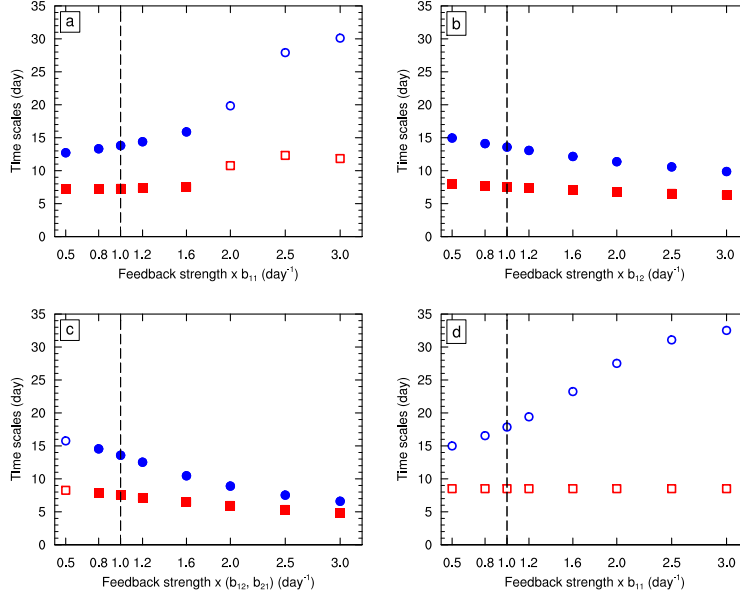
FIG. 12. The computed e -folding decorrelation time scale (day) of z_1 (blue circles) and z_2 (red squares) as a function of feedback strengths (day ^{-1} ). The impact of varying (a) b_{11} , (b) b_{12} , and (c) b_{12} and b_{21} on the decorrelation time scale (the y-axis) while all other b_{jk} are kept the same. The x-axis shows the value of varied b_{jk} as fraction of the value in EXP2 (Table 3); the vertical dashed line indicates the control values. (d) The impact of varying b_{11} in EXP1 (Table 3). The filled indicates that the parameters satisfy the condition for propagating regimes, i.e., existence of decaying-oscillatory solutions (Eq. (20)).
