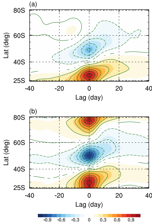
FIG. 6. One-point lag-correlation maps of the vertically averaged zonal-mean zonal wind anomalies from year-round ERA-Interim data integrated across the depth of the troposphere (1000-100 hPa) ( \bar{u} ) in the Southern Hemisphere. (a) Total anomaly fields and (b) reconstructed from projections onto the two leading EOFs of \bar{u} . The base latitude is at 30°S and the contour interval is 0.1. Regions enclosed by contour lines denote values significant at the 95% level according to the t -test.
