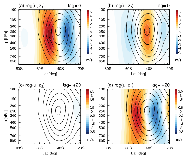
FIG. 3. Anomalous zonal-mean zonal wind ( \bar{u} ) regressed onto z_1 and z_2 in the GCM setup with non-propagating regime: (a, b) simultaneous, (c) z_2 leads by 20 days, and (d) z_1 leads by 20 days. The contours are the climatological zonal-mean zonal wind with interval of 5 \text{ ms}^{-1} .
