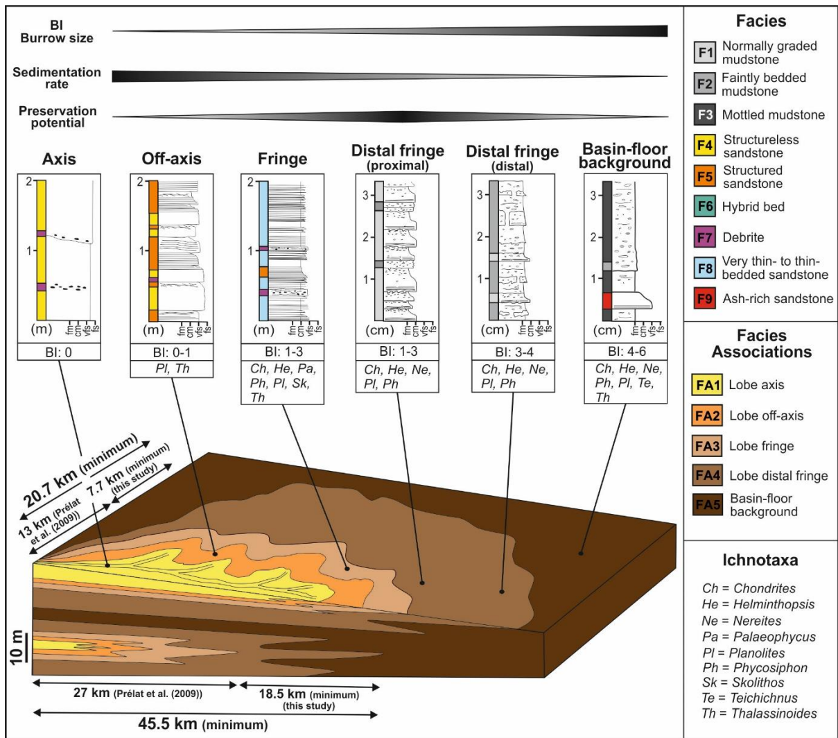
Figure 14: Depositional model of deep-water basin-floor lobes based on the description and interpretation of the Skoorsteenberg Formation. Representative sedimentological logs for each sub-environment are shown, along with facies, facies associations, ichnotaxa and bioturbation index (BI). Note the different vertical scales of the sedimentological logs between the sandstone-prone and mudstone-prone part of the model. Bioturbation index scale from Taylor and Goldring (1993).
