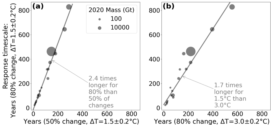
Fig. S 9. Response timescale in years after simulation start for different timescale definitions. Time when 80% of the committed mass loss has occurred at \Delta T=1.5^{\circ}\text{C} compared to (a) the estimates for 50% losses (Fig. S 11 vs. Fig. S 15) and (b) the estimates at \Delta T=3.0^{\circ}\text{C} . Each dot represents one of the 19 RGI regions. The size of the dots scales with the respective 2020 glacier mass.
