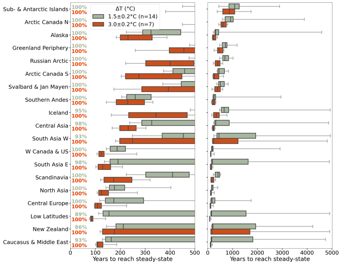
Fig. S 8. Years to reach steady state. For each region, percentiles (5 th , 25 th , median, 75 th , 95 th ) are calculated over the individual “year estimates” of the glacier models and climate scenarios (see Methods). In the left panel, the percentage of experiments (glacier model and climate scenario combinations) reaching steady state is highlighted (considering all climate scenarios, i.e. also those with little changes). Due to the 101-year rolling average, the steady state can be reached earlier than estimated under very fast-responding climate scenarios, regions and glacier models. n in legend refers to the number of climate scenarios.
