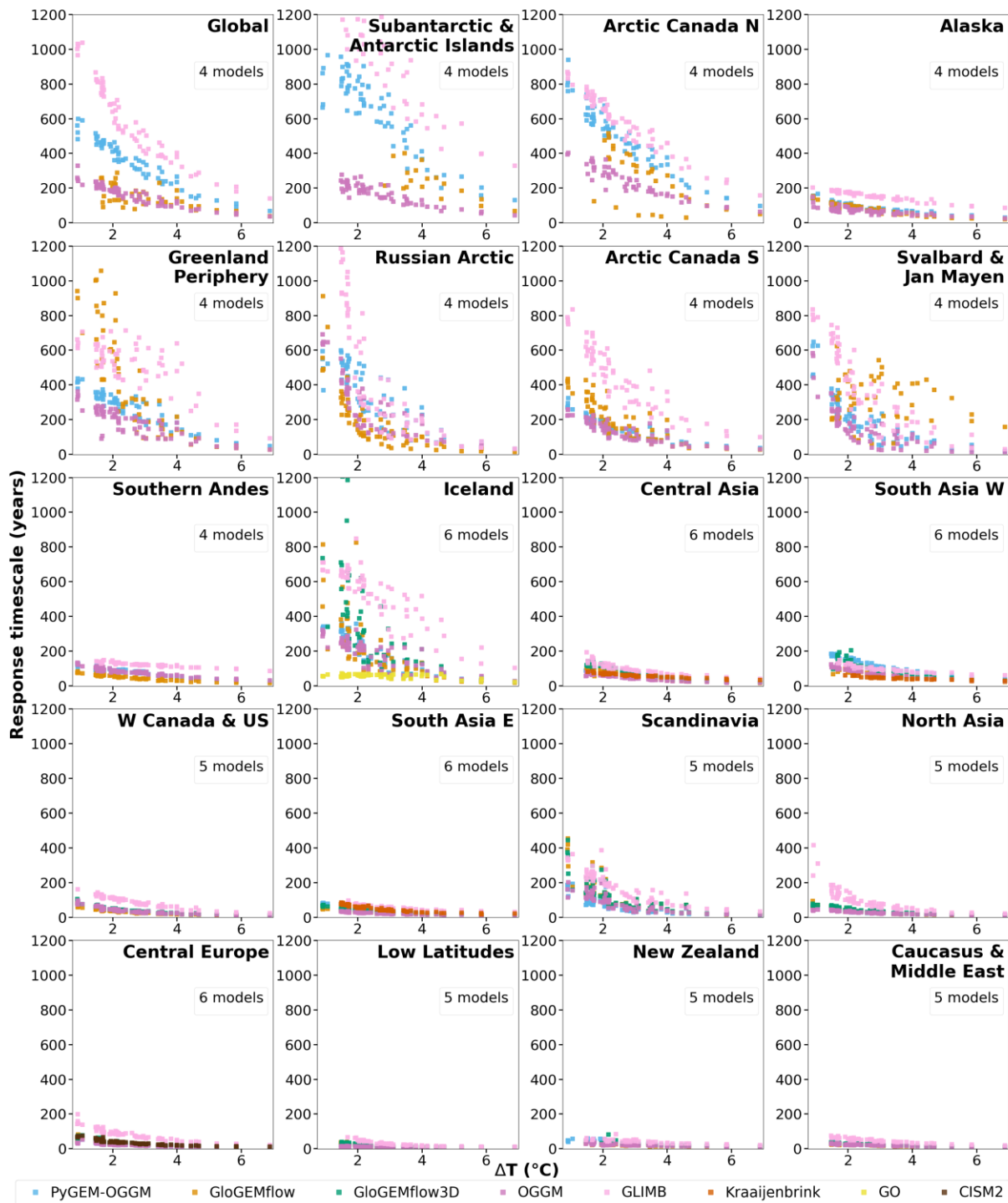
Fig. S 11. Response timescale in years from the simulation start when 80% of the committed mass loss between 2020 and steady state has occurred. Years are estimated from 21-year mass averages. Results are shown for glacier models and climate scenarios with \Delta T \geq 0.8^{\circ}\text{C} and at least 25% of committed mass change (see Methods). Fig. S 15 shows response timescale when 50% of the committed mass change occurs.
