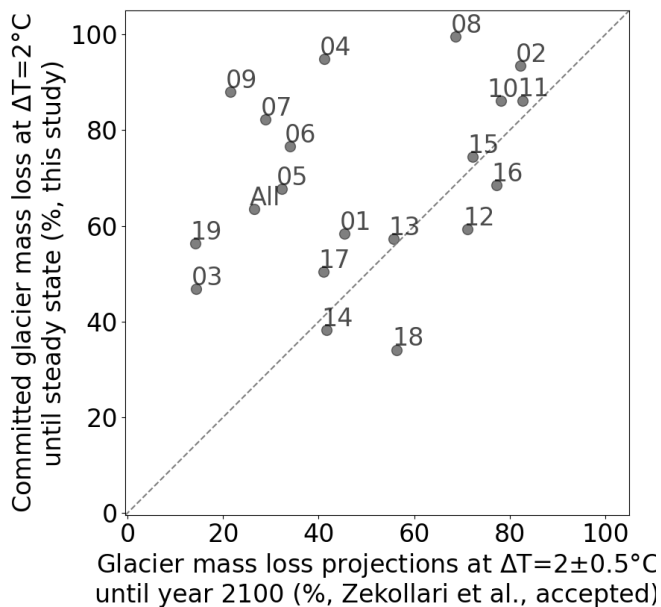
Fig. S 10. Committed glacier mass loss (in %, relative to 2020) from equilibration experiments (this study) versus mass losses by 2100 relative to 2015 derived from transient climate projections (11). For the equilibration experiments in this study, results are shown for \Delta T = 2^{\circ}\text{C} (median LOWESS fit). The 21 st century glacier projections are from Zekollari et al. (11), representing the median of three global glacier models (PyGEM-OGGM, OGGM, GloGEM) and of 17 climate model and SSP combinations of CMIP6 within the \Delta T = 2^{\circ}\text{C}\pm 0.5^{\circ}\text{C} range. “All” indicates the global losses, while the numbers refer to the RGI region numbers (refer to Table S 3 for naming).
