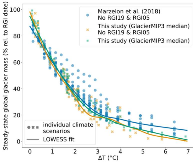
Fig. S 7. Sensitivity of committed global glacier mass loss to global mean warming levels above pre-industrial, compared to Marzeion et al. (13). For direct comparison, estimates are shown relative to the simulation start (RGI date) instead of 2020 as in the main text. In Marzeion et al. (13), about 60% of the global glacier mass is simulated, excluding Subantarctic & Antarctic Islands (RGI19) and the Greenland Periphery (RGI05).
