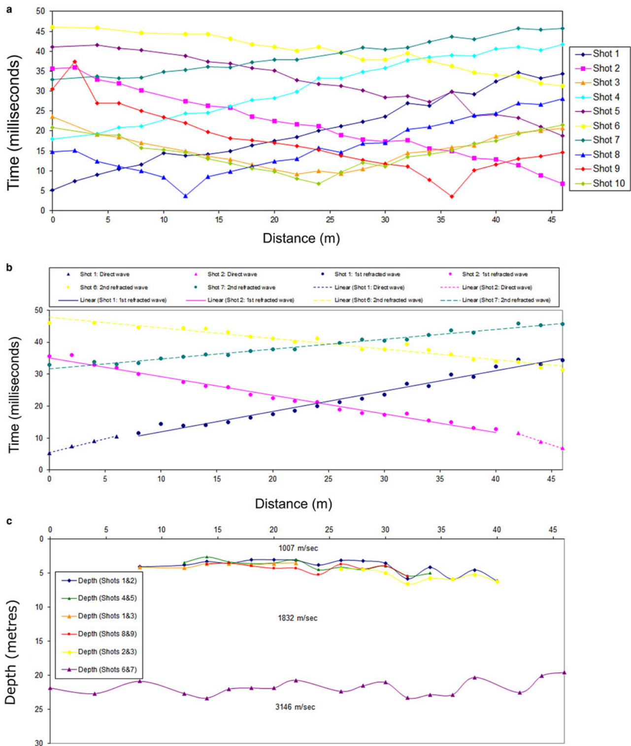
Fig. 5. Seismic refraction measurements, 'Pingo' 3, Rhos Llawr Cwrt, Cletwr Fawr. The seismic refraction profile ran perpendicular to Cletwr ERT 2, intersecting it at the location of borehole 1; (a) seismic refraction traveltimes graph; (b) traveltimes graph of selected seismic refraction shots, demonstrating the direct, first refracted and second refracted waves observed; (c) Seismic refractor depths and morphology, derived using the Common Receiver Point method.
