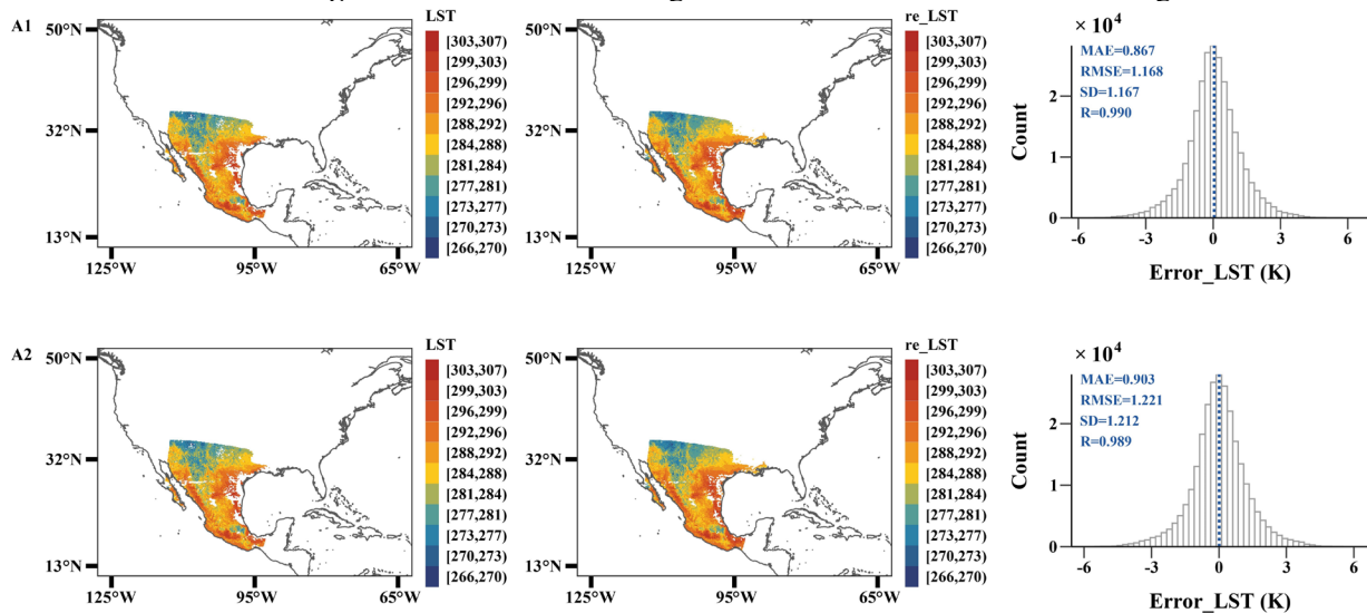
Extended Data Fig. 2. Error Distribution Diagram of LST and WVC Inversion Using Simulation Data
