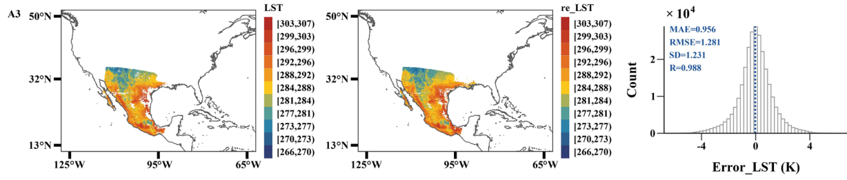
Extended Data Fig. 3. Cross-validation of MODIS LST products and MODIS retrieval LST result (2022.4.18) for band combination: (1) 5BT_to_LST (27, 28, 29, 31, 32) ; (2) 4BT_to_LST (28, 29, 31, 32) ; (3) 4BT_to_LST (27, 28, 31, 32) . Histograms illustrate the statistical difference (MODIS LST product data minus MODIS retrieval LST data), in which the dashed blue lines represent the MAE.
