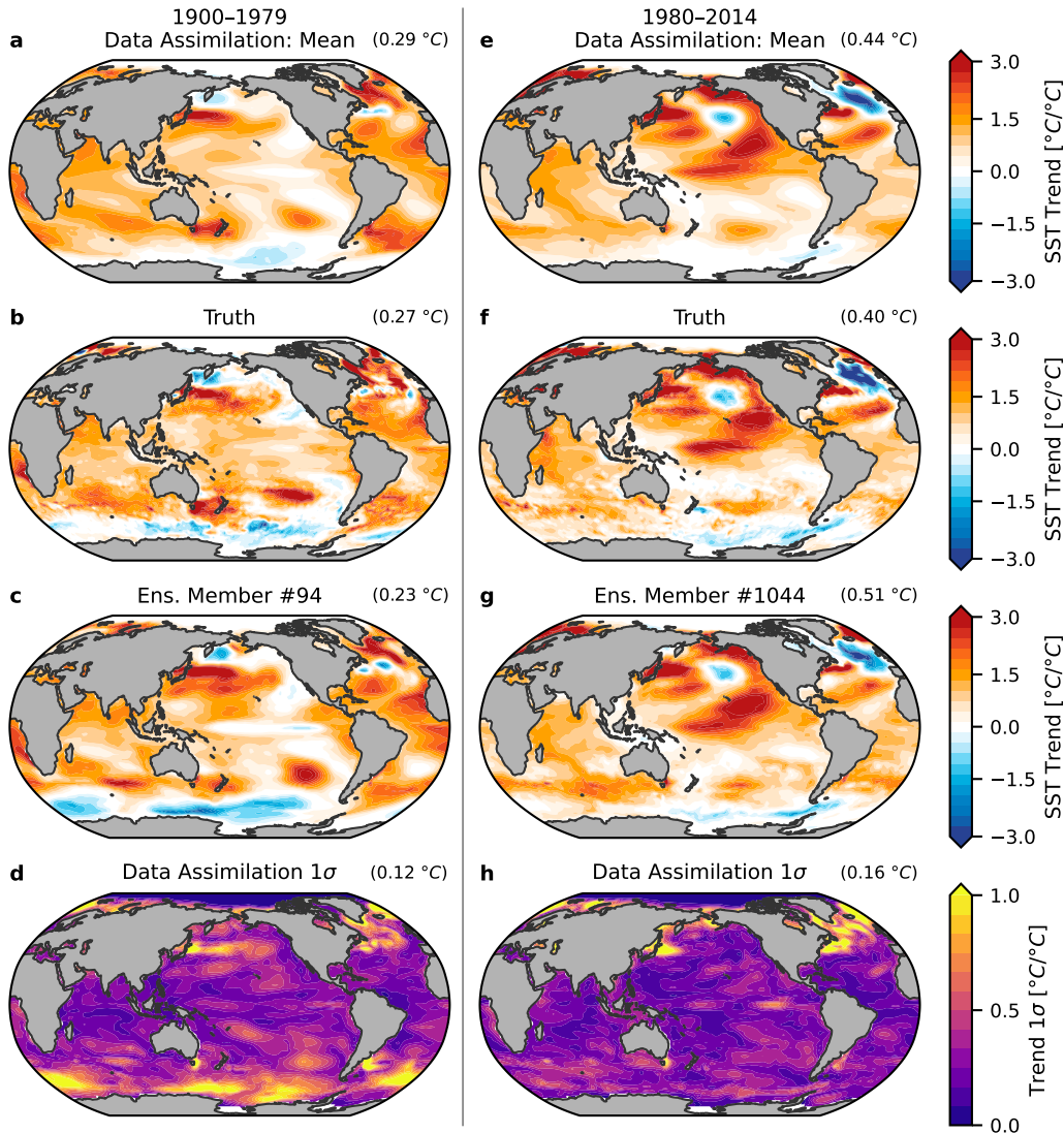
FIG. 3. Validation by pseudo-reconstruction: SST trends. (a) Normalized 1900–1979 ensemble mean of trends from data assimilation; local trends are divided by the global-mean trend to show SST patterns; upper-right indicates the global-mean trend before normalization, scaled by the number of years to show trend in ^{\circ}\text{C} per 80 years. (b) Repeats panel a but showing true trends in the pseudo-reconstruction’s target model, MPI-ESM1-2-HR’s historical simulation. (c) Repeats panel a but shows an individual member from ensemble data assimilation. (d) Uncertainty in results from data assimilation, calculated as the sample standard deviation ( 1\sigma ) across 1600 ensemble members’ normalized trends; values greater than 1.0 indicate that local 1\sigma is greater than the global-mean trend; upper-right shows the global-mean of the 1\sigma in local trends before normalization. (e–f) Repeats panels a–d for 1980–2014.
