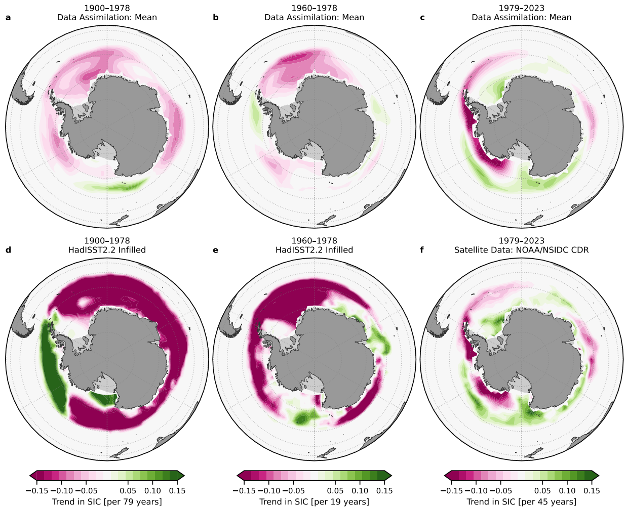
Fig. 9. Historical trends in Antarctic sea-ice concentration (SIC). (a–c) Ensemble mean of trends from data assimilation, scaled by the number of years in each time period to show trends in SIC per N years. (d–f) Repeats panels a–c but showing comparison datasets, with infilled HadISST2.2 in panels d–e and NOAA/NSIDC CDR from satellite data in panel f. Note that SIC is bounded from 0 to 1.
