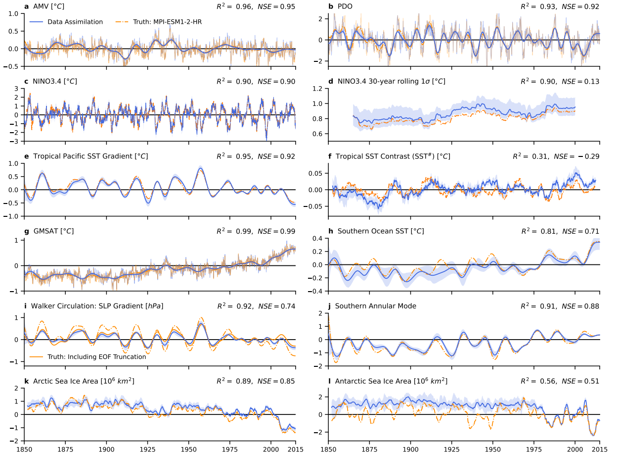
FIG. 2. Validation by pseudo-reconstruction: timeseries. (Orange) True values from the target model, the 1850–2014 historical simulation from MPI-ESM1-2-HR. (Blue) Result from data assimilation, showing mean of 1600 ensemble members; shading denotes ensemble 17 th and 83 rd percentiles, i.e., likely range. (a) Atlantic Multidecadal Variability with 10-yr low-pass filter and monthly values as thin lines. (b) Pacific Decadal Oscillation with 6-yr low-pass filter and monthly values as thin lines. (c) Monthly Nino3.4 with 30-yr running mean removed. (d) Rolling 30-yr standard deviation of Nino3.4 in panel c. (e) Zonal gradient of tropical Pacific SST with 10-yr low-pass filter. (f) Tropical SST contrast, SST # , 5-yr running mean. (g) Global-mean near-surface air temperature (GMSAT) with 10-yr low-pass filter and monthly values in thin lines. (h) Zonal mean of Southern Ocean SST (50°–70°S) with 10-yr low-pass filter. (i) Walker circulation, i.e., zonal SLP gradient across tropical Pacific, with 10-yr low-pass filter. (j) Southern Annular Mode with 10-yr low-pass filter. (k) Total area of Arctic sea ice with 24-month running mean. (l) Total area of Antarctic sea ice, with 24-month running mean. Calculation of metrics is described in Methods Section 2d.
