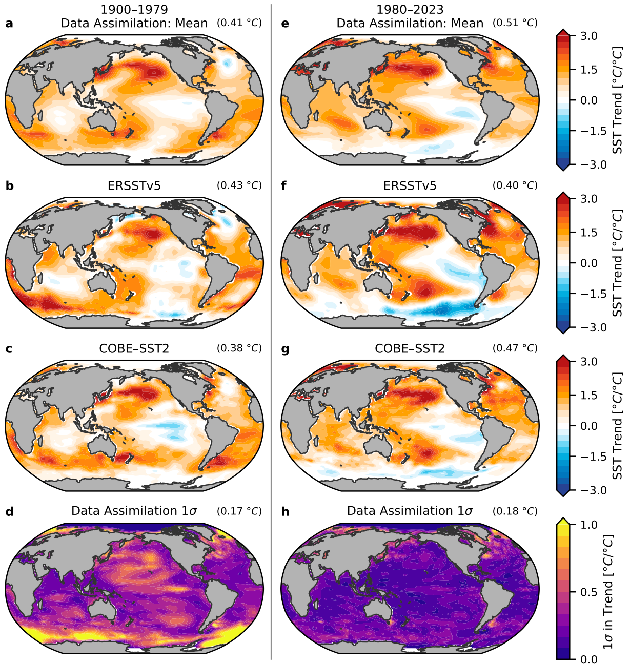
FIG. 6. Historical patterns of SST trends. (a) Normalized 1900–1979 ensemble mean of trends from data assimilation; local trends are divided by the global-mean trend to show SST patterns; upper-right value is the global-mean trend before normalization, scaled by the number of years to show trend in ^{\circ}\text{C} per 80 years. (b) Repeats panel a but showing comparison data from NOAA ERSSTv5 and (c) COBE-SST2. (d) Uncertainty in results from data assimilation, calculated as the sample standard deviation ( 1\sigma ) across 1600 ensemble members' normalized trends; values greater than 1.0 indicate that local 1\sigma is greater than the global-mean trend; upper-right value is the global-mean of the 1\sigma in local trends before normalization. (e–f) Repeats panels a–d for 1980–2023.
