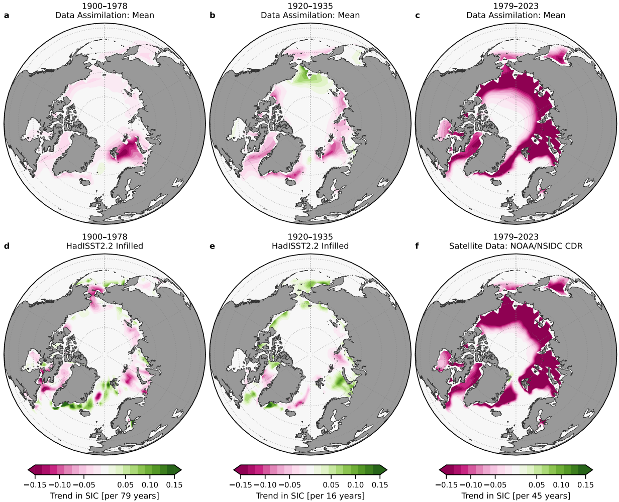
FIG. 8. Historical trends in Arctic sea-ice concentration (SIC). (a–c) Ensemble mean of trends from data assimilation, scaled by the number of years in each time period to show trends in SIC per N years. (d–f) Repeats panels a–c but showing comparison datasets, with infilled HadISST2.2 in panels d–e and NOAA/NSIDC CDR from satellite data in panel f. Note that SIC is bounded from 0 to 1.
