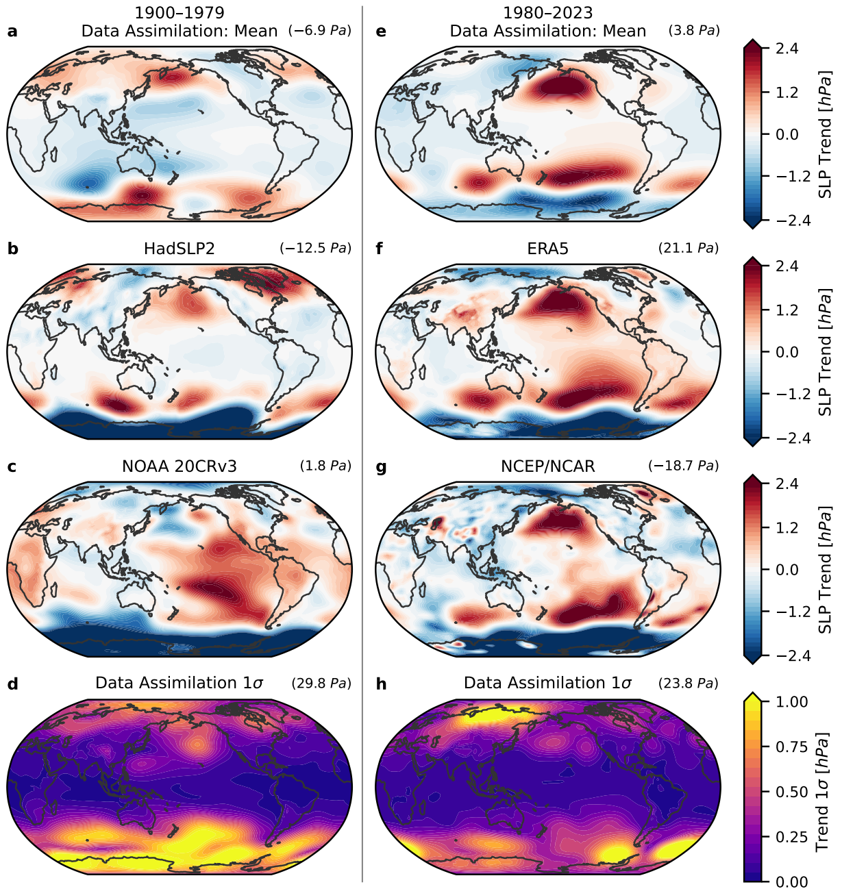
FIG. 7. Historical trends in sea-level pressure (SLP). (a) 1900–1979 ensemble mean of trends from data assimilation, scaled by the number of years to show trends in hPa per 80 years; upper-right indicates the global-mean trend in Pa per 80 years. (b) Repeats panel a but showing comparison datasets HadSLP2 and (c) NOAA 20CRv3. (d) Uncertainty in results from data assimilation, calculated as the sample standard deviation ( 1\sigma ) across local trends from 1600 ensemble members; upper-right shows the global mean of the 1\sigma in local trends. (e–f) Repeats panels a–d for 1980–2023, with comparison reanalyses from (f) ERA5 and (g) NCEP/NCAR.
