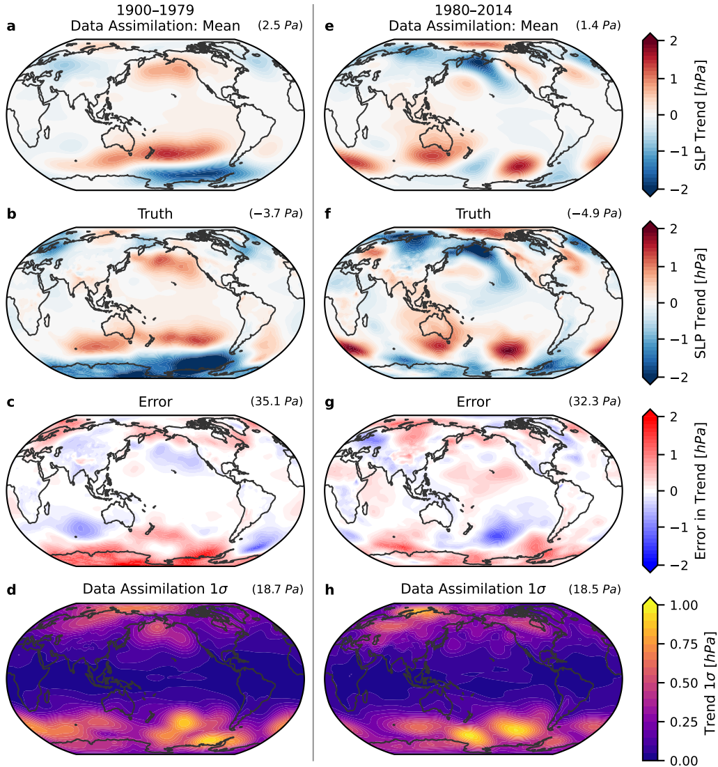
FIG. 4. Validation by pseudo-reconstruction: trends in sea-level pressure (SLP). (a) 1900–1979 ensemble mean of trends from data assimilation, scaled by the number of years to show trends in hPa per 80 years; upper-right indicates the global-mean trend in Pa per 80 years. (b) Repeats panel a but showing true trends in the pseudo-reconstruction’s target model, MPI-ESM1-2-HR’s historical simulation. (c) Error, shown as mean reconstruction minus truth; RMSE shown in upper right. (d) Uncertainty in results from data assimilation, calculated as the sample standard deviation ( 1\sigma ) across trends from 1600 ensemble members; upper-right shows the global mean of the 1\sigma in local trends. (e–f) Repeats panels a–d for 1980–2014.
