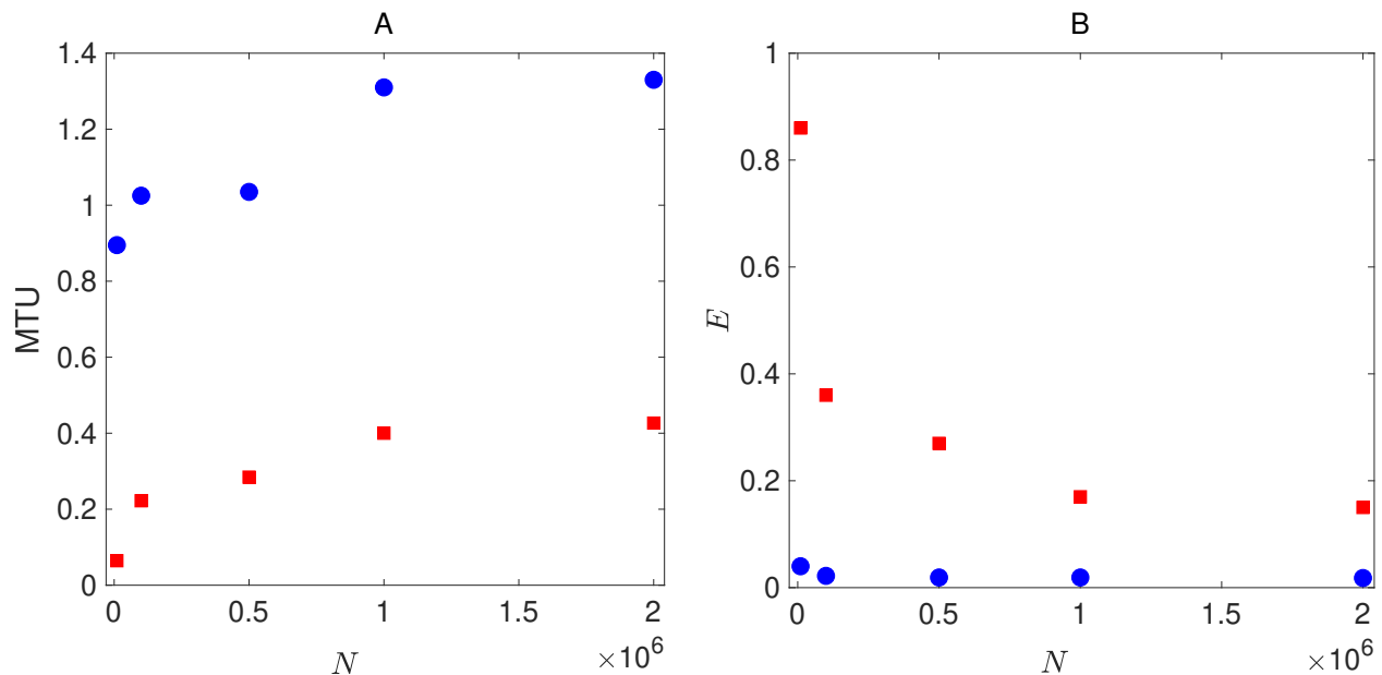
Figure 7: Comparison of the short-term prediction quality for RC-ESN (blue circles) and ANN (red squares) as the size of the training set N is changed from N = 10^4 to N = 2 \times 10^6 . (A) Prediction horizon (when e(t) reaches 0.3). (B) Average error E (see Eq. (10)). For RC-ESN, algorithm T_2 , D = 5000 , and \rho = 0.1 are used.
