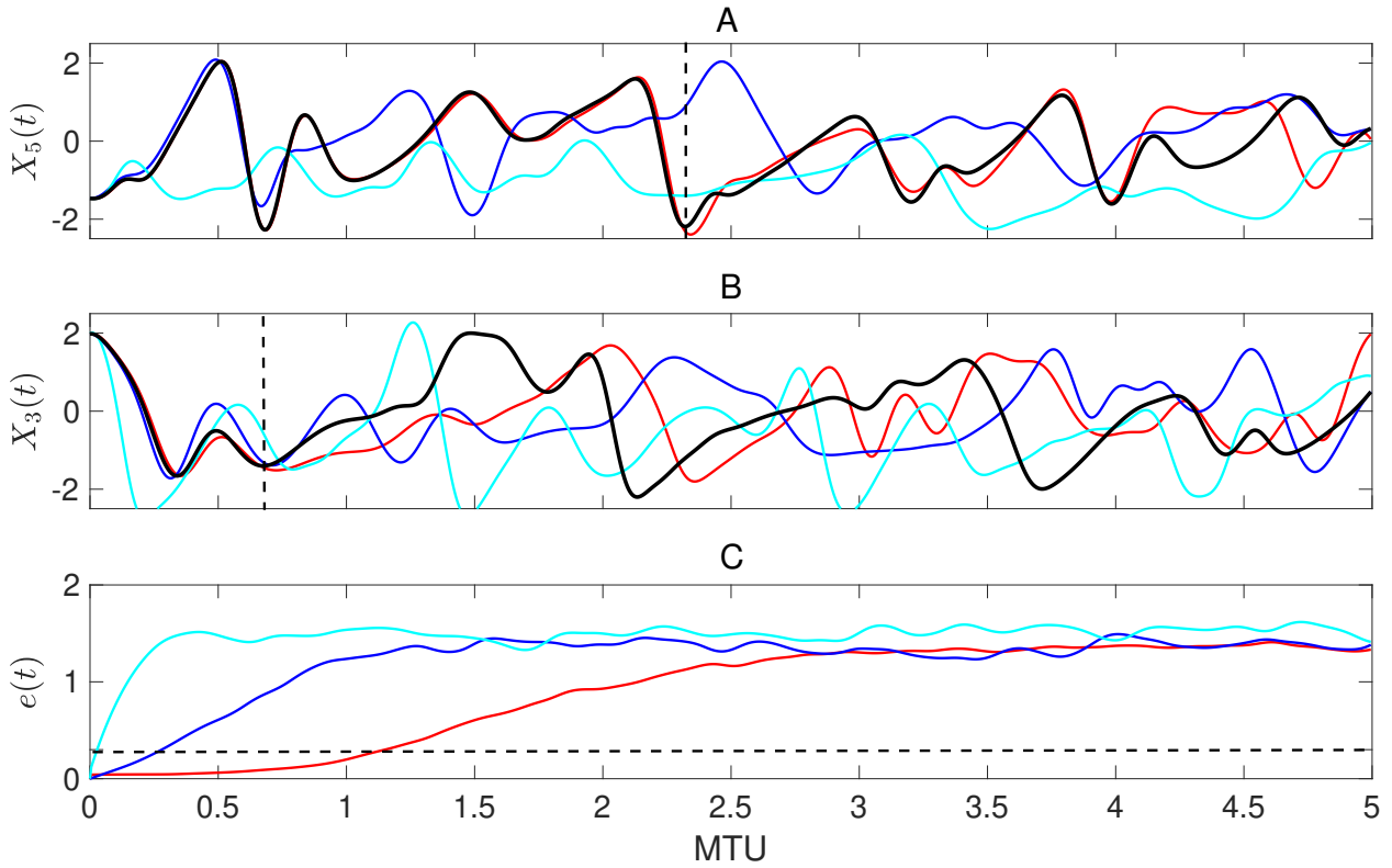
Figure 5: Comparison of the short-term forecast skills among the three deep learning methods. The lines show truth (black), RC-ESN (red), ANN (blue), and RNN-LSTM (cyan). (A) and (B) show examples (differing in initial condition) for which RC-ESN yields the longest and shortest prediction horizons, respectively. Vertical dashed lines approximately show the prediction horizon of RC-ESN. (C) Relative L_2 error averaged over 100 randomly chosen initial conditions e(t) (see Eq. (9)). The dashed horizontal line marks e = 0.3 . Time is in MTU, where 1 \text{ MTU} = 200\Delta t \approx 4.5/\lambda_{max} . Training size is N = 500000 . For RC-ESN, algorithm T_2 , D = 5000 , and \rho = 0.1 are used. This value of \rho is found to give the best results. The effects of other transformation algorithms and larger N and D are discussed later.
