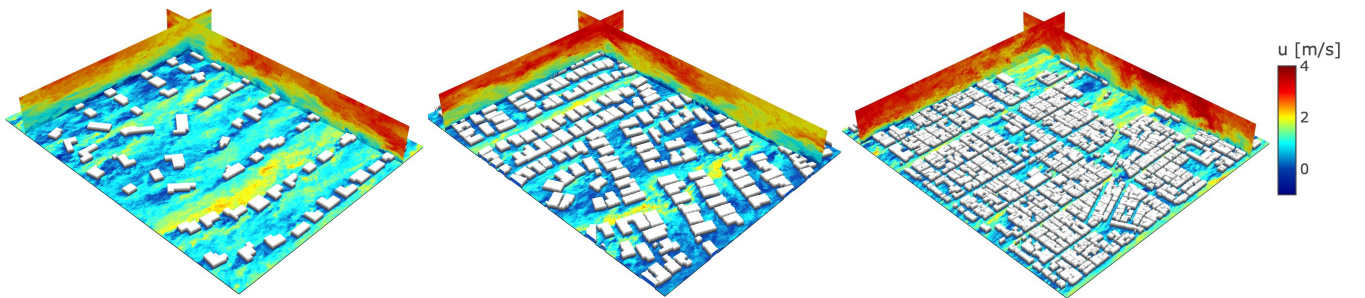
Figure 6. Three examples of instantaneous wind field over realistic neighborhoods from Northfield Township, United States ( \lambda_p = 0.131 ) Melbourne, Australia ( \lambda_p = 0.342 ), and Tokyo, Japan ( \lambda_p = 0.590 ) respectively. The horizontal plane is sampled at the pedestrian height ( z = 1.75\text{m} ). Two vertical cross-sections at positions x = y = 55\text{m} are also shown. Full animations are available in the supplementary material.
