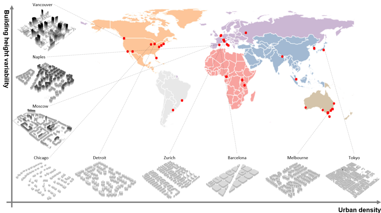
Figure 3. Geographic representation of realistic neighborhoods selected for LES simulations. We consider both uniform and variable height scenarios, to ensure that we cover both horizontal and vertical heterogeneities that enable comparison with idealized cases (Lu et al., 2023b).
