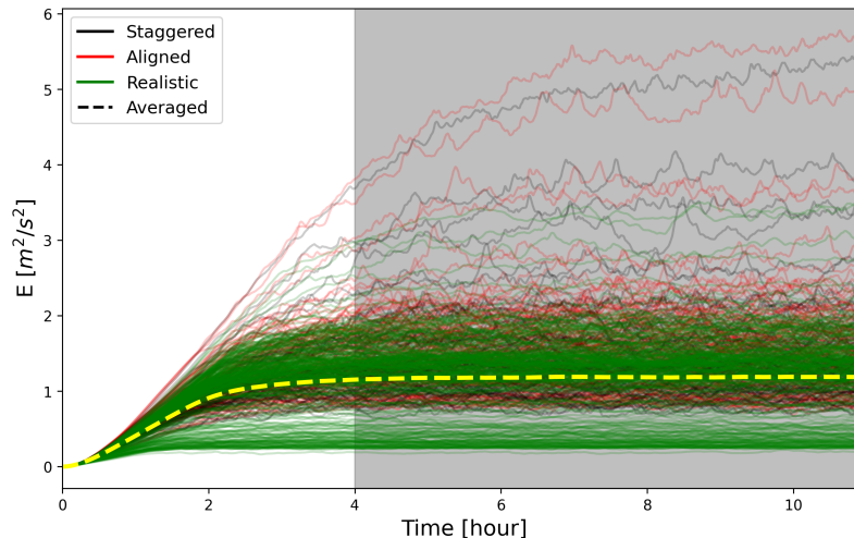
Figure 4. Time-series of total kinetic energy (KE) indicating the quasi-steady state and time-averaging window from 4th to 11th hour. The color of the lines reflect the urban geometry configuration, where black, red, and green lines (with transparency to distinguish different cases) represent staggered, aligned, and realistic, respectively. The yellow dotted line represents 538-cases-averaged time series.
