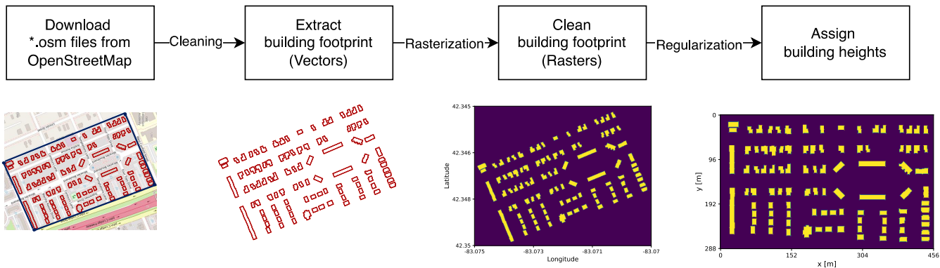
Figure 2. Schematic diagram of downloading, rasterization, and regularization of building footprint using OSM2LES to prepare urban topography for LES simulation.
