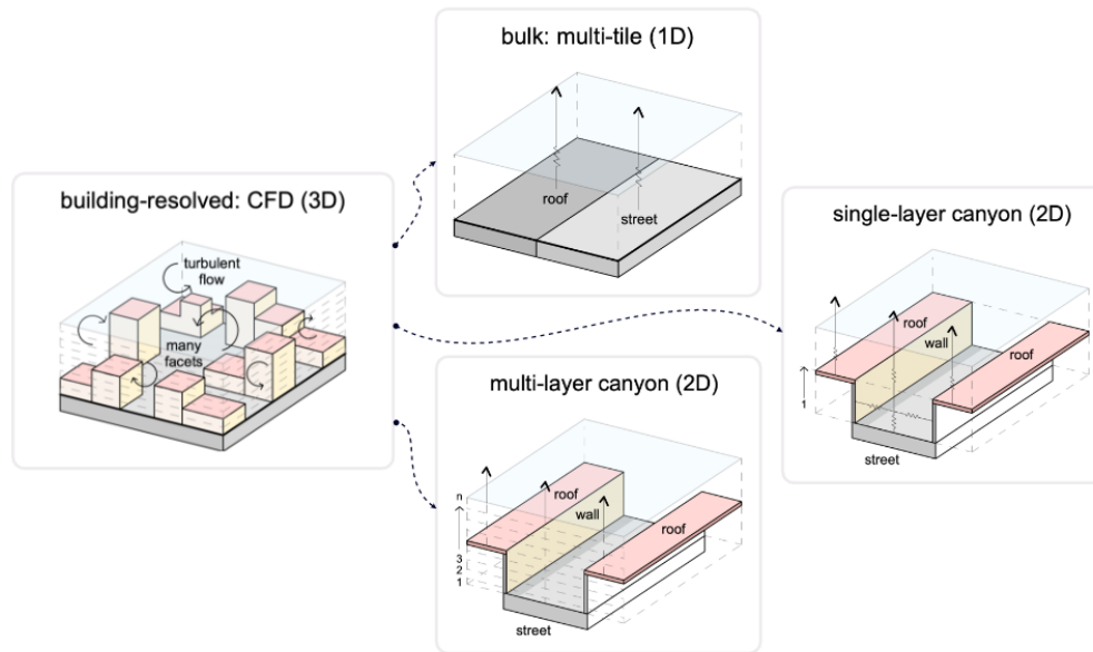
Figure 10. 3D LES dataset informing a suite of other urban canopy models, ranging from simplified tiled models to single-layer and multi-layer urban canopy models that are used offline to assess urban climate or integrated into regional models.
