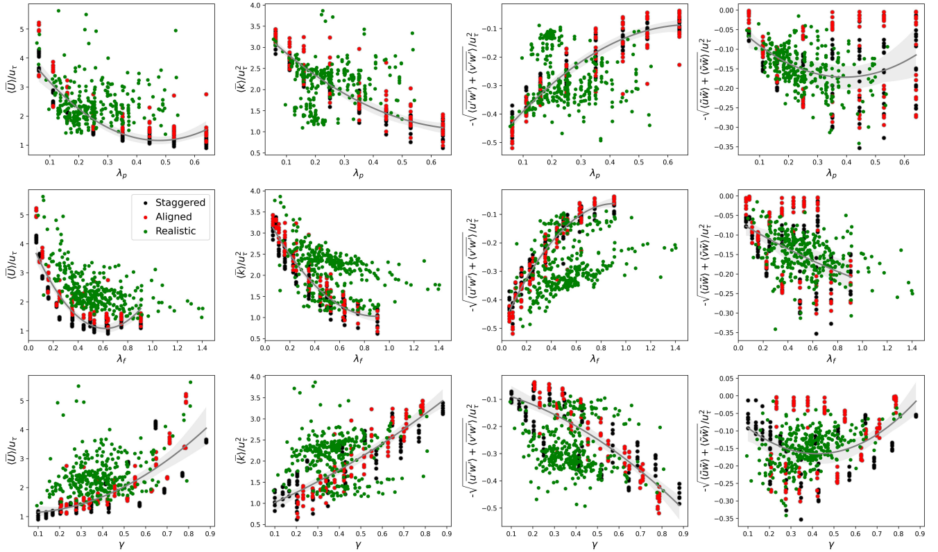
Figure 7. Scatterplots of canopy-averaged flow statistics in UrbanTALES against plan and frontal area density and street connectivity ((Lu et al., 2023b)). The y-axis represent in four columns represent normalized mean wind speed ( \langle \bar{U} \rangle / u_\tau ), TKE ( \langle \bar{k} \rangle / u_\tau^2 ), Reynolds stress ( -\sqrt{\langle u'w' \rangle + \langle v'w' \rangle} / u_\tau^2 ), and dispersive fluxes ( -\sqrt{\langle \tilde{u}\tilde{w} \rangle + \langle \tilde{v}\tilde{w} \rangle} / u_\tau^2 ), respectively. We used colors to distinguish aligned (red), staggered (black), and realistic (green) urban geometrical configurations. In each subplot, a gray line shows the fitting for a semi-logarithmic regression over only idealized urban configurations.
