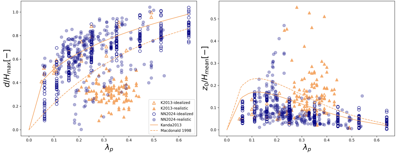
Figure 8. Scatterplots of urban roughness flow parameters (roughness length ( z_0 ) and displacement height ( d )) in UrbanTALES against plan area density \lambda_p . We used colors and marks to distinguish data points from Kanda et al. (2013a) (sandybrown with hollow and solid triangles for idealized and realistic configuration) and from UrbanTALES (navyblue with hollow and solid circles for idealized and realistic configuration). In each subplot, the solid and dashed lines is showing the regression formula from Kanda et al. (2013a) and Macdonald et al. (1998), respectively.
