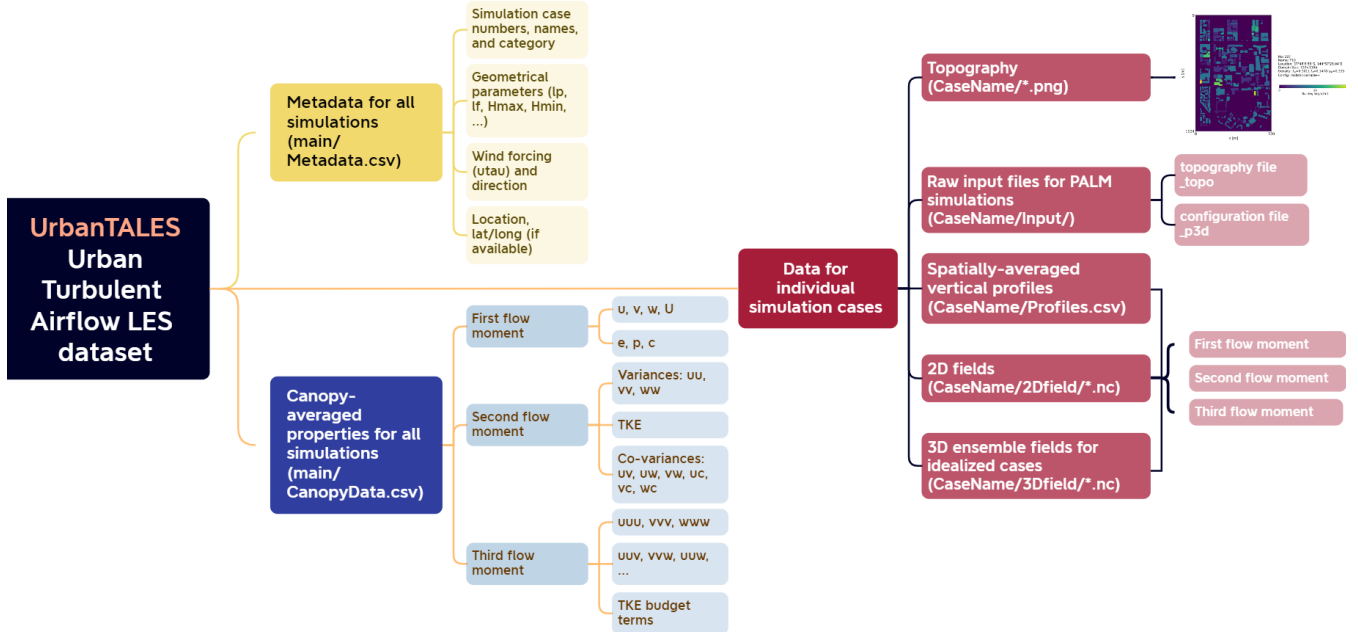
Figure 5. Overview of the UrbanTALES dataset file structure. The metadata datasheet and canopy-averaged flow statistics are provided at the whole dataset level. The topography information (including visualized urban geometry along with some geometrical details), PALM input, vertical profiles, pedestrian-level flow field, and ensemble 3D field are provided at individual case level.
