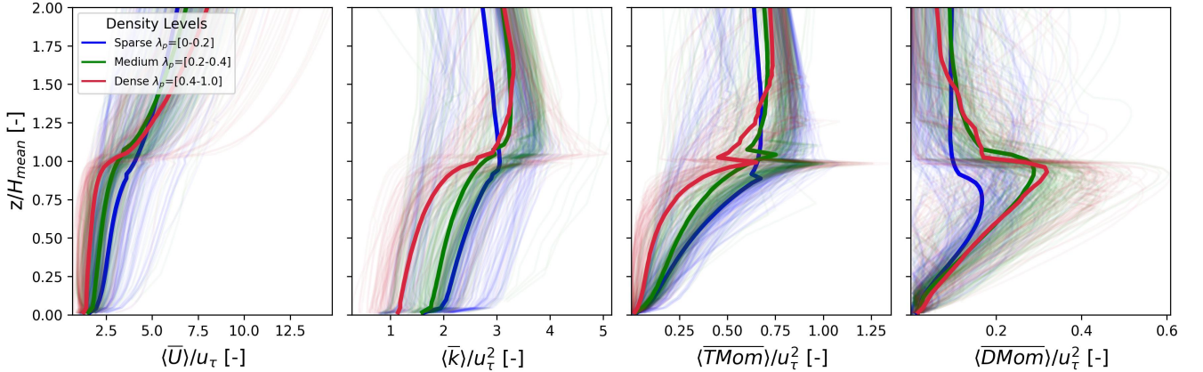
Figure 9. Vertical profiles up to 2H_{\text{mean}} of wind speed U = \sqrt{u^2 + v^2} , turbulent kinetic energy \bar{k} = \frac{1}{2}(\overline{u'u'} + \overline{v'v'} + \overline{w'w'}) , and total turbulent and dispersive momentum flux \overline{\text{TMom}} = \sqrt{\overline{u'w'^2} + \overline{v'w'^2}} \overline{\text{DMom}} = \sqrt{\overline{u\tilde{w}^2} + \overline{v\tilde{w}^2}} normalized by friction velocity, respectively. We separated UrbanTALES into three categories - sparse (cyan), medium (orange), and dense (red) urban configurations based on the plane area density \lambda_p , which is shown for individual cases in the background with high transparency. The category-averaged vertical profiles are shown in solid lines with the same coloring.
