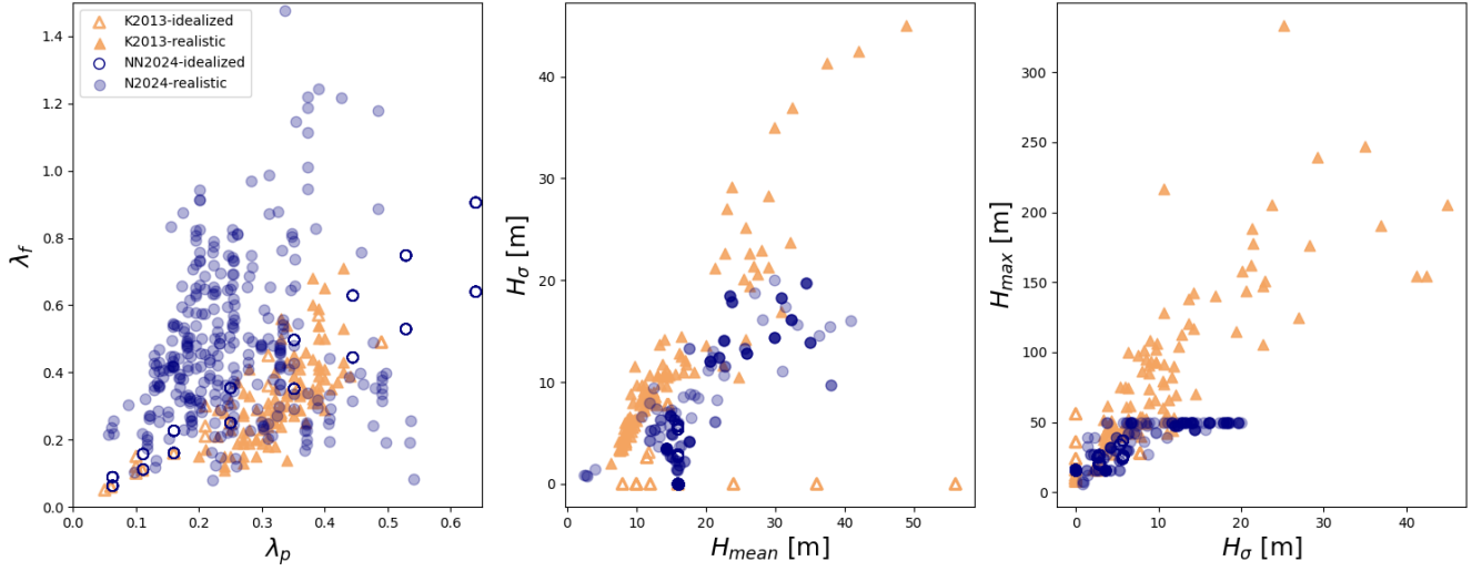
Figure 1. Distribution of urban geometrical parameters in UrbanTALES compared with LES simulations of Kanda et al. (2013a), \lambda_p and \lambda_f represent plan and frontal area density, H_\sigma , H_{mean} , and H_{max} represent standard deviation of building height distribution and mean and maximum of building height.
