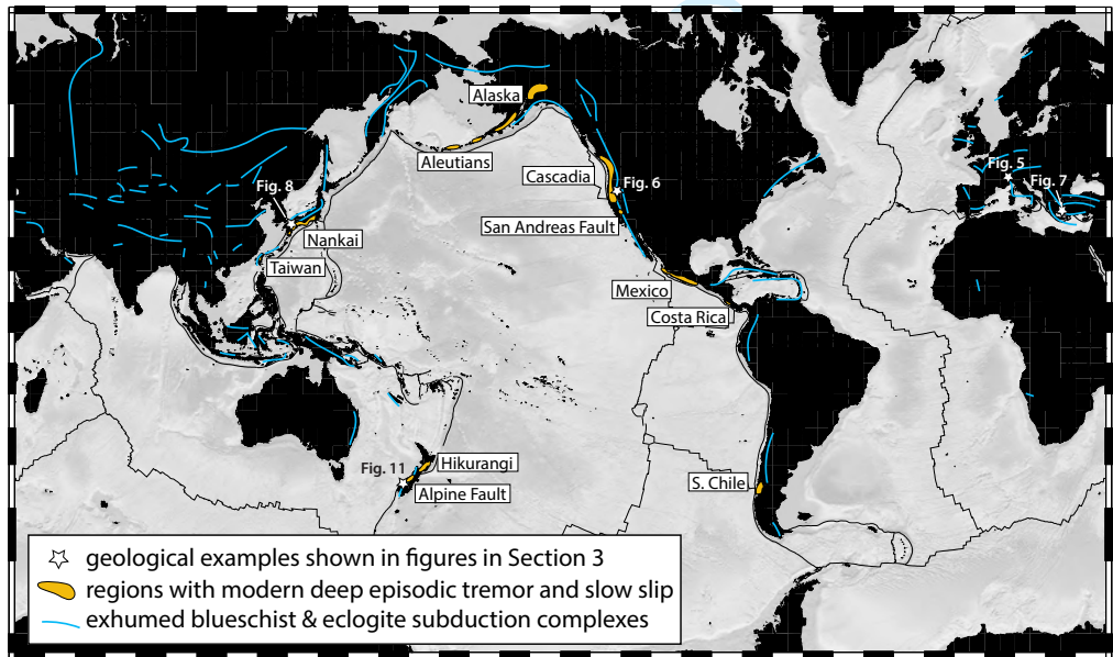
Figure 1. Global distribution of regions with modern deep episodic tremor and slow slip along with exhumed blueschist and eclogite facies subduction complexes.
