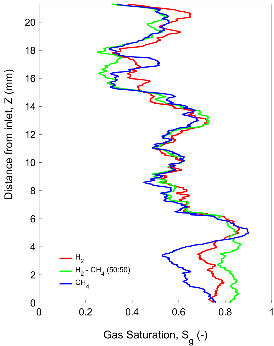
Figure S5: 1-D slice-averaged of gas saturation after imbibition for Exp 3 : \langle b \rangle = 450 \mu\text{m} .
