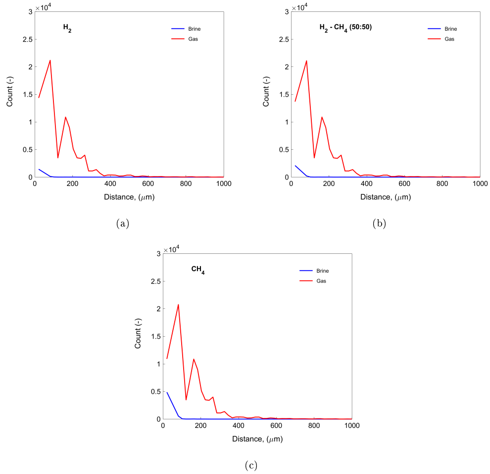
Figure S3: Fluid phase occupancy in Exp 3, D = 25 \text{ mm} , \langle b \rangle = 450 \text{ }\mu\text{m} (a) \text{H}_2 (b) \text{H}_2 - \text{CH}_4 (50 : 50) (c) \text{CH}_4 . The distance is calculated as twice the maximum distance from the center of the aperture to the nearest wall of the fracture.
