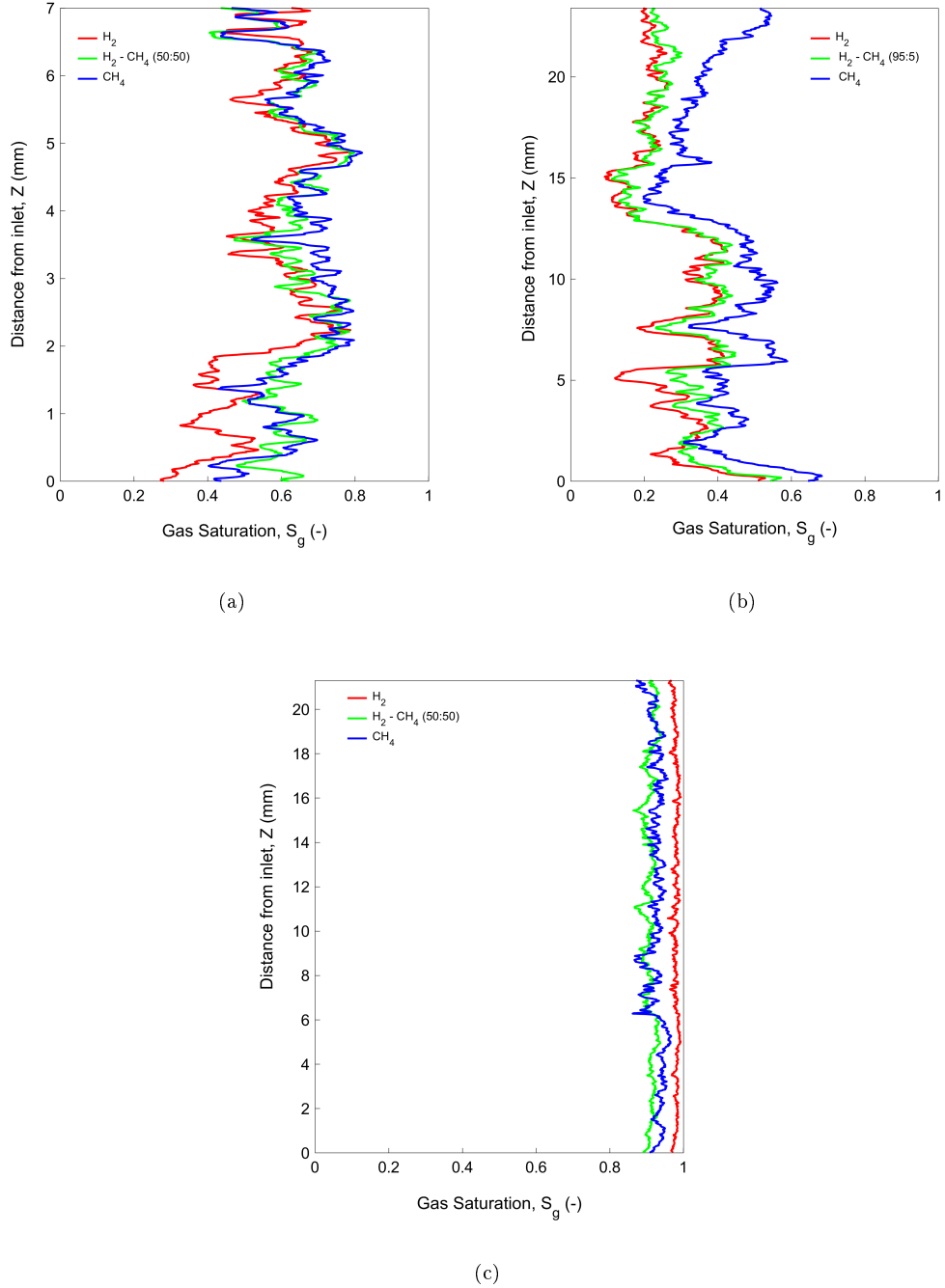
Figure 6: 1-D slice-average gas saturation after drainage along the length of rock core for different gases. (a) Exp 1, D = 6 mm, \langle b \rangle = 130 \mu\text{m} (b) Exp 2, D = 25 mm, \langle b \rangle = 255 \mu\text{m} (c) Exp 3, D = 25 mm, \langle b \rangle = 450 \mu\text{m} .
