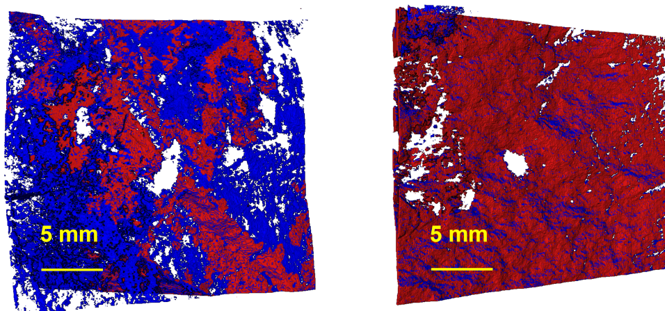
Figure S4: (3-D volume rendering of \text{CH}_4 - brine distribution after drainage (a) Exp 2: \langle b \rangle = 255 \mu\text{m} . (b) Exp 3: \langle b \rangle = 450 \mu\text{m} . The red color denotes gas and blue color denotes brine phase.
