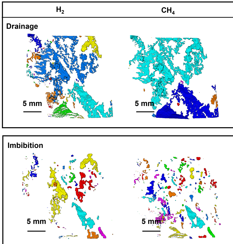
Figure 7: Trapped gas phase for H 2 and CH 4 Exp 2; \langle b \rangle = 255 \mu\text{m} . Each color represents a connected gas ganglia of different size. (Top) after drainage (Bottom) after imbibition
