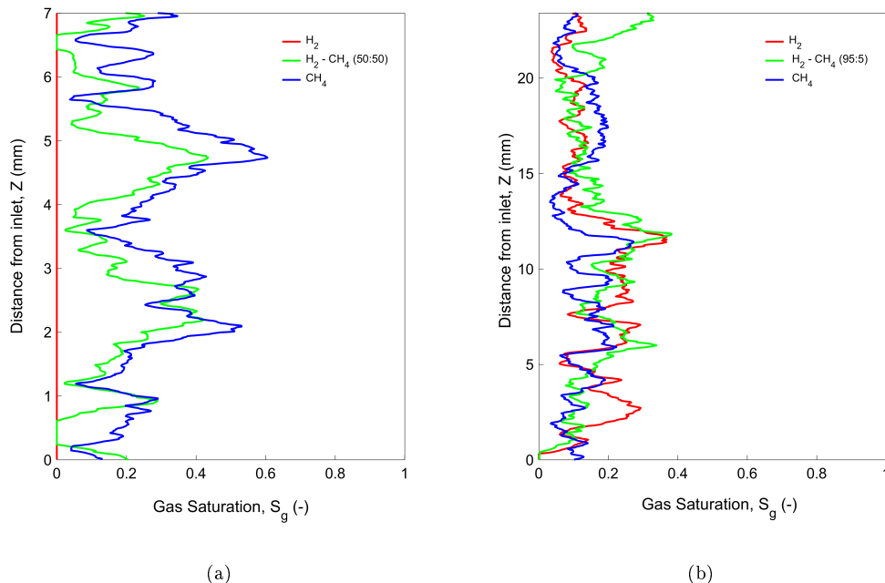
Figure 11: 1-D slice-average gas saturation after imbibition. (a) Exp 1 : \langle b \rangle = 130 \mu\text{m} (b) Exp 2 : \langle b \rangle = 255 \mu\text{m} .
