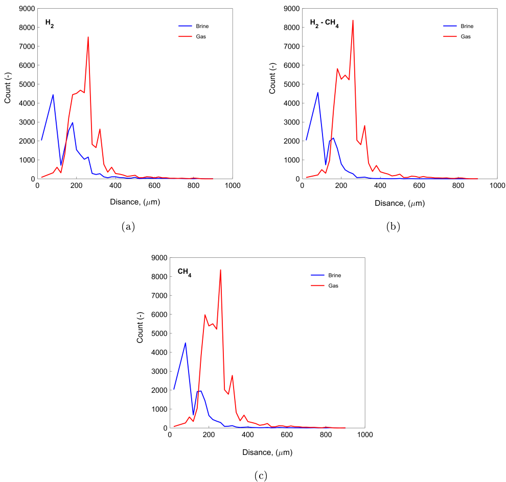
Figure 5: Fluid phase occupancy in Exp 1, D = 6 \text{ mm} , \langle b \rangle = 130 \text{ }\mu\text{m} (a) \text{H}_2 (b) \text{H}_2 - \text{CH}_4 (50:50) (c) \text{CH}_4 . The distance is calculated as twice the maximum distance from the center of the aperture to the nearest wall of the fracture.
