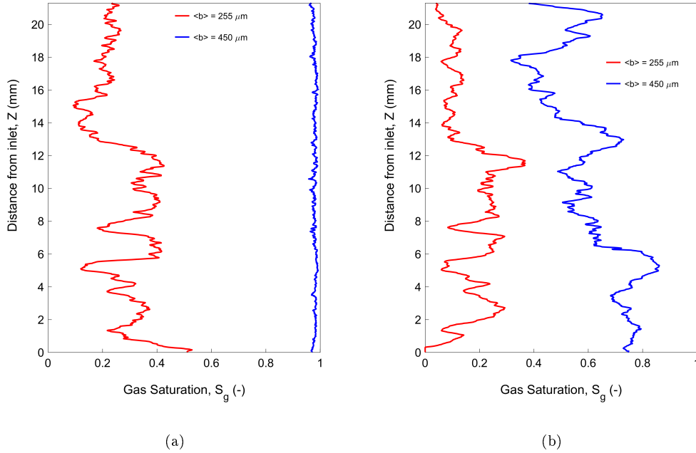
Figure 9: 1-D slice-average gas saturation H_2 for cores with different fracture aperture size. The red line denotes saturation for Exp 2 : D = 25 \text{ mm} , \langle b \rangle = 255 \mu\text{m} . The blue line denotes the saturation for Exp 3: D = 25 \text{ mm} , \langle b \rangle = 450 \mu\text{m} . (a) after drainage (b) after imbibition.
