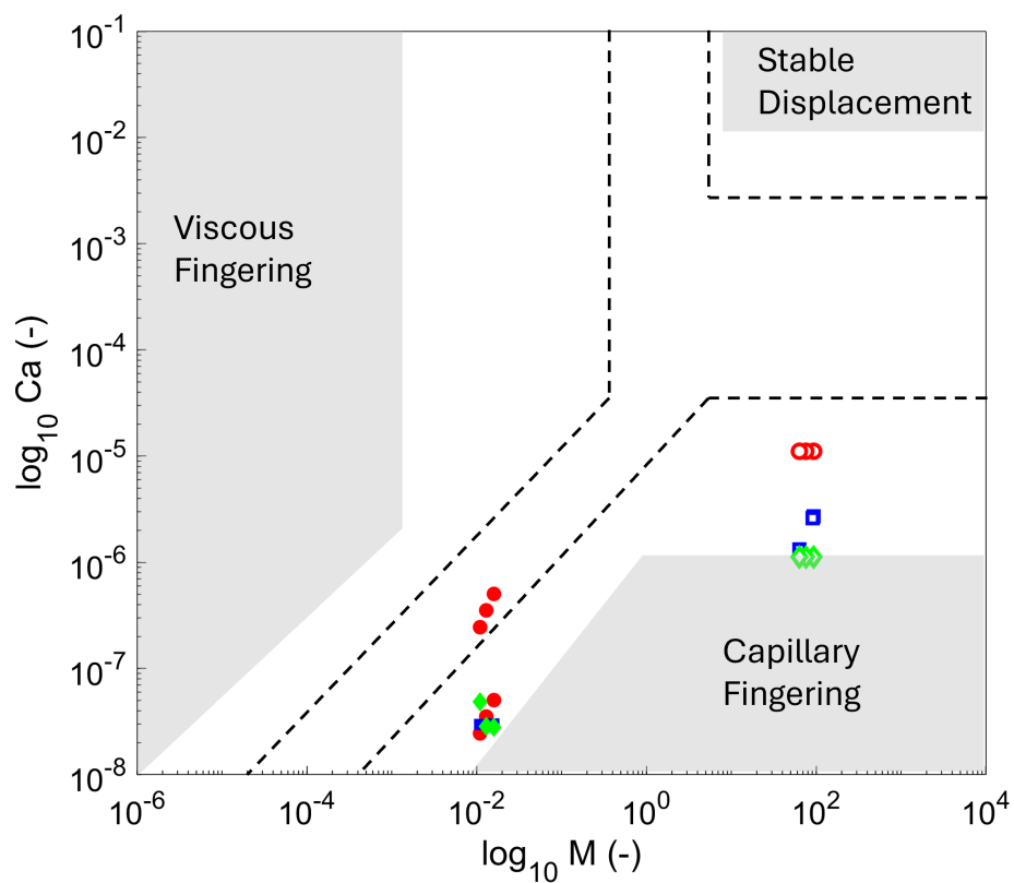
Figure S1: Capillary number (Ca) and viscosity ratio (M) for drainage studied in this paper overlaid on phase diagram for porous media [1]. The filled markers represent drainage experiments, while the empty markers correspond to imbibition experiments. Red circles indicate Exp 1, green diamonds represent Exp 2, and blue squares denote Exp 3.
