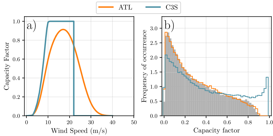
Fig. 3. (a) Power curves of the Enercon E112.4500 with a 0.3w smoothing filter used by the ATL dataset (orange) and the Vestas V136/3450 used by the two C3S datasets (blue) (b) Histograms of wind CF for Ireland for the ATL dataset (orange), the C3S datasets (blue) and Observed (shaded).
