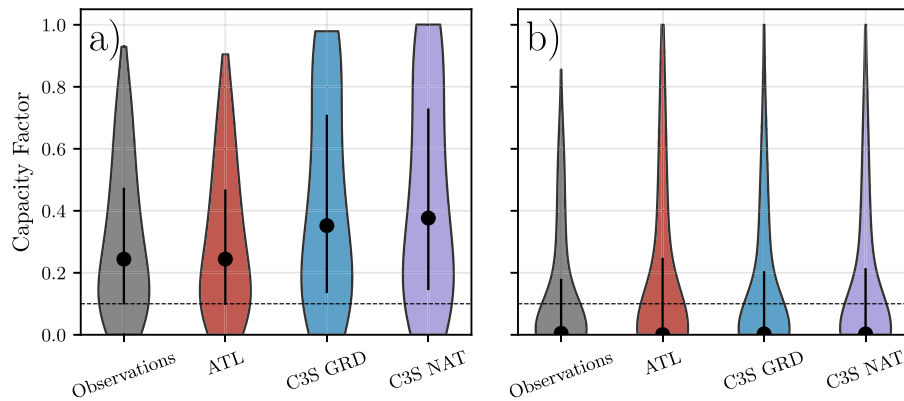
Fig. 2. Violin plots of CF distributions for (a) wind and (b) solar PV for the Observations (grey) and the three datasets: ATL (red), C3S GRD (blue), and C3S NAT (purple). The black dot shows the median values, while the black vertical lines represent the first and third quartiles. The black dashed line indicates the threshold of 0.1 used in the study to identify RES droughts.
