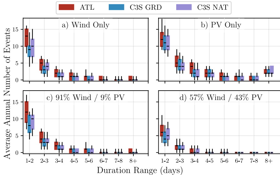
Fig. 8. Average annual number of RES droughts (from 1979 to 2023) for (a) Wind, (b) solar PV, (c) 91W-9PV and (d) 57W-43PV for ATL (red), C3S GRD (blue), and C3S NAT (purple). The x-axis represents duration ranges in days (lower bound included), while the y-axis indicates the annual number of events. The boxes display the first and third quartiles and the median is marked by a black line. The whiskers indicate the 5th and 95th percentiles.
