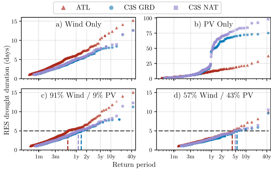
Fig. 9. Return periods of the duration of RES droughts (from 1979 to 2023) for (a) Wind, (b) Solar PV, (c) 91W-9PV and (d) 57W-43PV for ATL (red triangle), C3S GRD (blue circle), and C3S NAT (purple square). The x-axis represents the return period time in a log-scale and the y-axis indicates the duration of RES drought associated with it. The horizontal dashed line marks the 5-day return period, with coloured vertical dashed marking its return period for each dataset.
