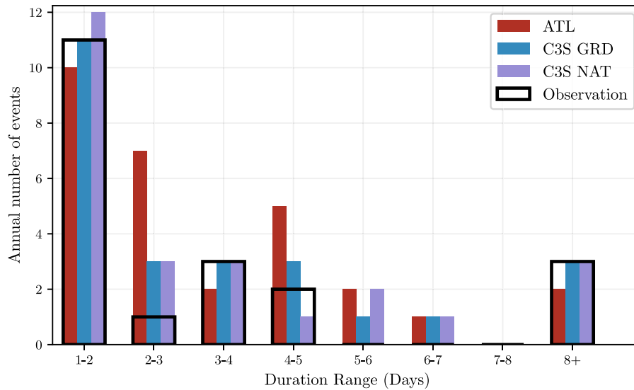
Fig. 7. Number of solar PV drought events for ATL (red), C3S GRD (blue), and C3S NAT (purple) and the observed data (black outline). The solar PV droughts are identified for 2023, considering the actual capacity of the system at any given time.
