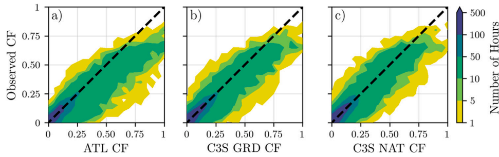
Fig. 6. Solar PV CF density plot of the observed (vertical axes) and modelled (horizontal axes) CF series for the (a) ATL, (b) C3S GRD and (c) C3S NAT datasets.
