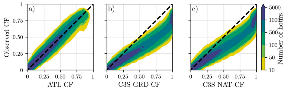
Fig. 4. Wind CF density plot of the observed CF (vertical axes) and modelled (horizontal axes) CF data for the (a) ATL, (b) C3S GRD and (c) C3S NAT datasets.
