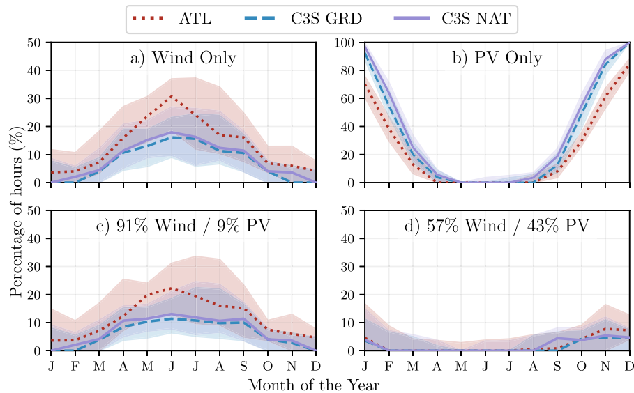
Fig. 10. Percentage of hours in a month which are part of a RES drought (from 1979 to 2023) for (a) Wind, (b) Solar PV, (c) 91W-9PV and (d) 57W-43PV for ATL (red dotted), C3S GRD (blue dashed), and C3S NAT (purple solid). The x-axis represents the month of the year, and the y-axis indicates the percentage of hours. Lines correspond to the median values and the area between the first and third quartiles is shaded. Note the different y-axis scale for (b).
