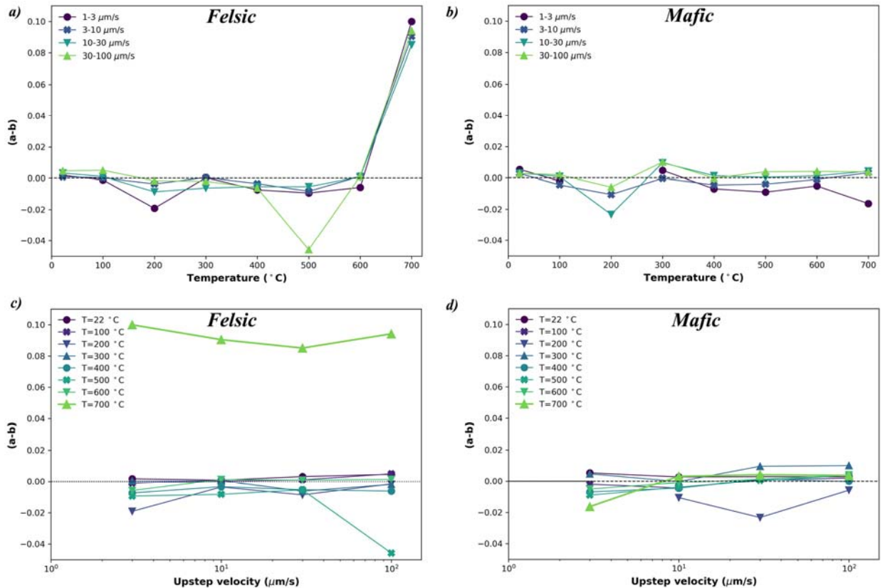
Figure 6: Plots of (a-b) as a function of temperature (a,b) as well as sliding velocity (c,d) for all experiments performed at 100 MPa effective normal stress (see Tables 2, 3 and 4). a, c) Felsic sample b, d) Mafic sample
