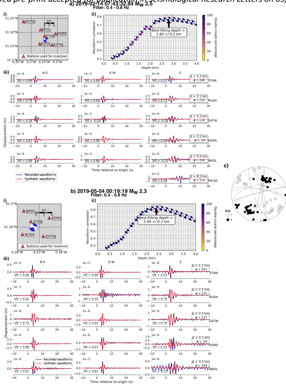
Figure 5: a) and b) Representative moment tensor solutions for two earthquakes recorded by all five local stations. i) Map showing stations and best-fitting focal mechanism; ii) waveform correlation as a function of centroid depth; iii) waveform fits. “VR” = variance reduction. c) Observed first-motion P-wave polarities from all events in the catalogue represent a composite faulting mechanism compared to fault planes from the best-fitting focal mechanisms from moment tensors a) and b).
