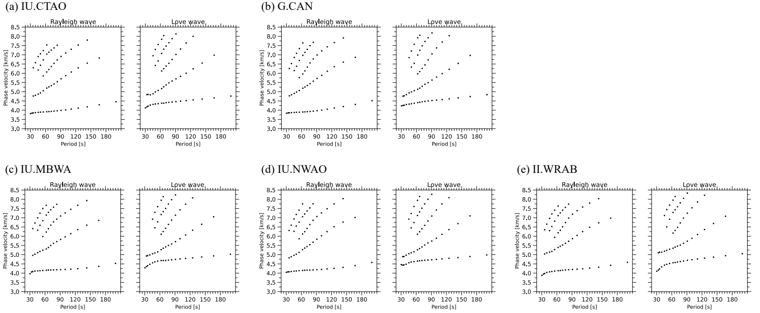
Figure S2: Phase speed dispersion data of multimode Rayleigh and Love waves for five
