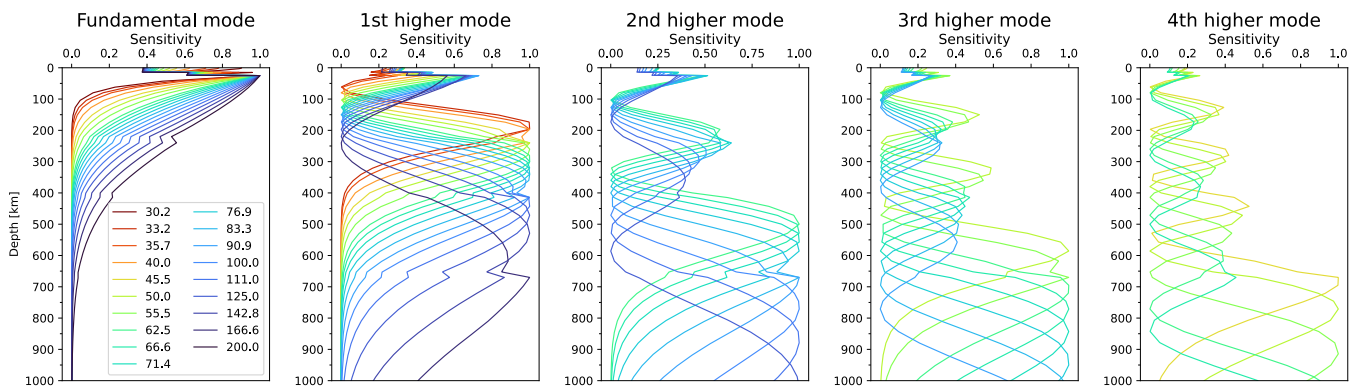
15 Figure S1. Normalized sensitivity kernels of surface waves for anisotropic PREM
