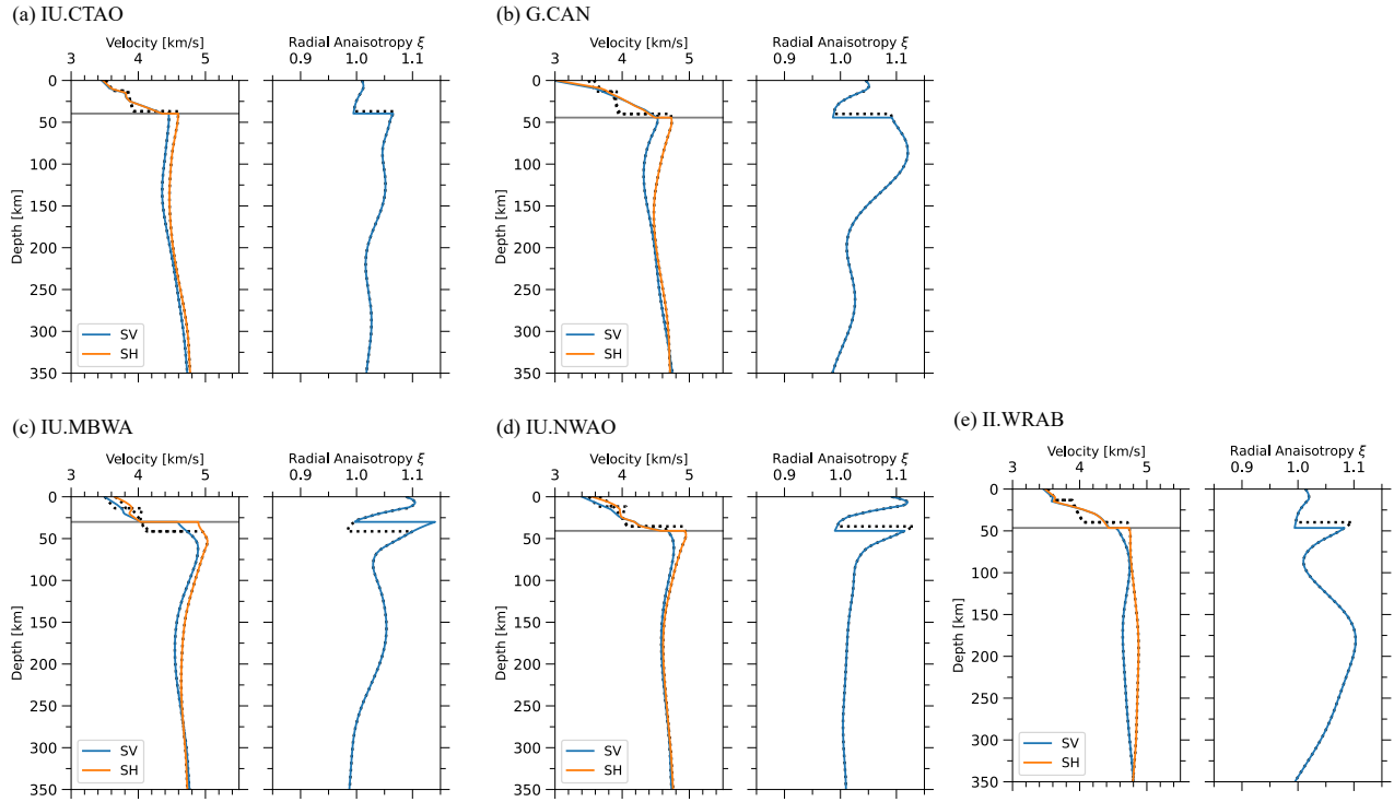
30 Figure S6: Local reference structural models (SV and SH velocities and radial anisotropy) for each station. Solid colored lines represent the reference SV and SH wave models used in this study taken from the 3-D radially anisotropic tomographic model (Yoshizawa, 2014), replacing the crust with AuSREM (Kennett et al. , 2013; Salmon, Kennett and Saygin, 2013) and AusMoho (Kennett et al. , 2011, 2023).
