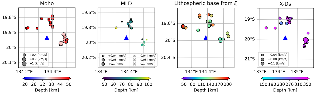
Figure 11: Same as Figure 9, but for three cratonic stations where MLDs have been observed: (a) IU.MBWA, (b) IU.NWAO, and (c) II.WRAB. CP maps for MLDs are added to the mid-left panel in all stations. Note that the mid-right panel for (c) II.WRAB represents the lithospheric base derived from an increase of radial anisotropy \xi , for which the circle sizes are constant, unlike other panels. The mid-left panel displays the CPs for MLDs, with circles and crosses indicating negative and positive changes in shear velocity, respectively.
