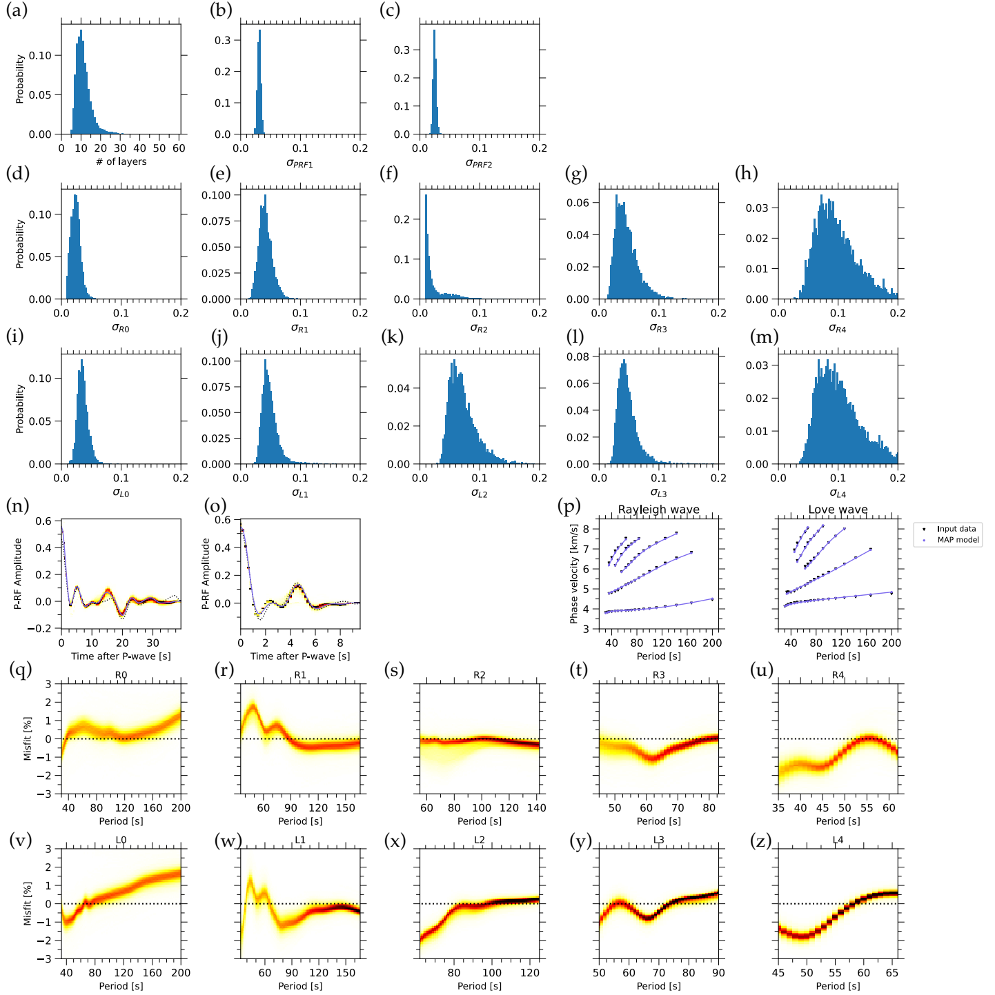
50 Figure S8: Same as Figure S7, but for the western event group (Figure 5 (c) in the main text).
