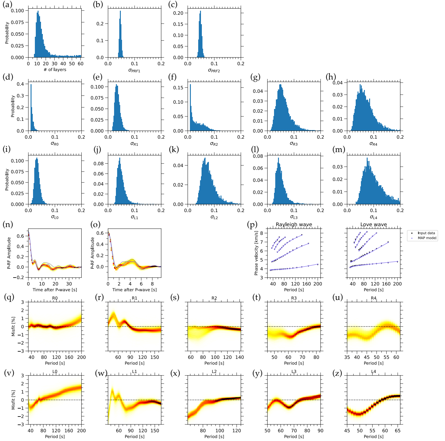
35 Figure S7: Posterior distributions of hyperparameters and marginal distributions of data misfit for IU.CTAO results using the eastern event group (Figure 5 (b)). (a) The number of layers. (b, c) Data noises for the low-frequency P-RF ( \sigma_{PRF1} ) and the high-frequency P-RF
