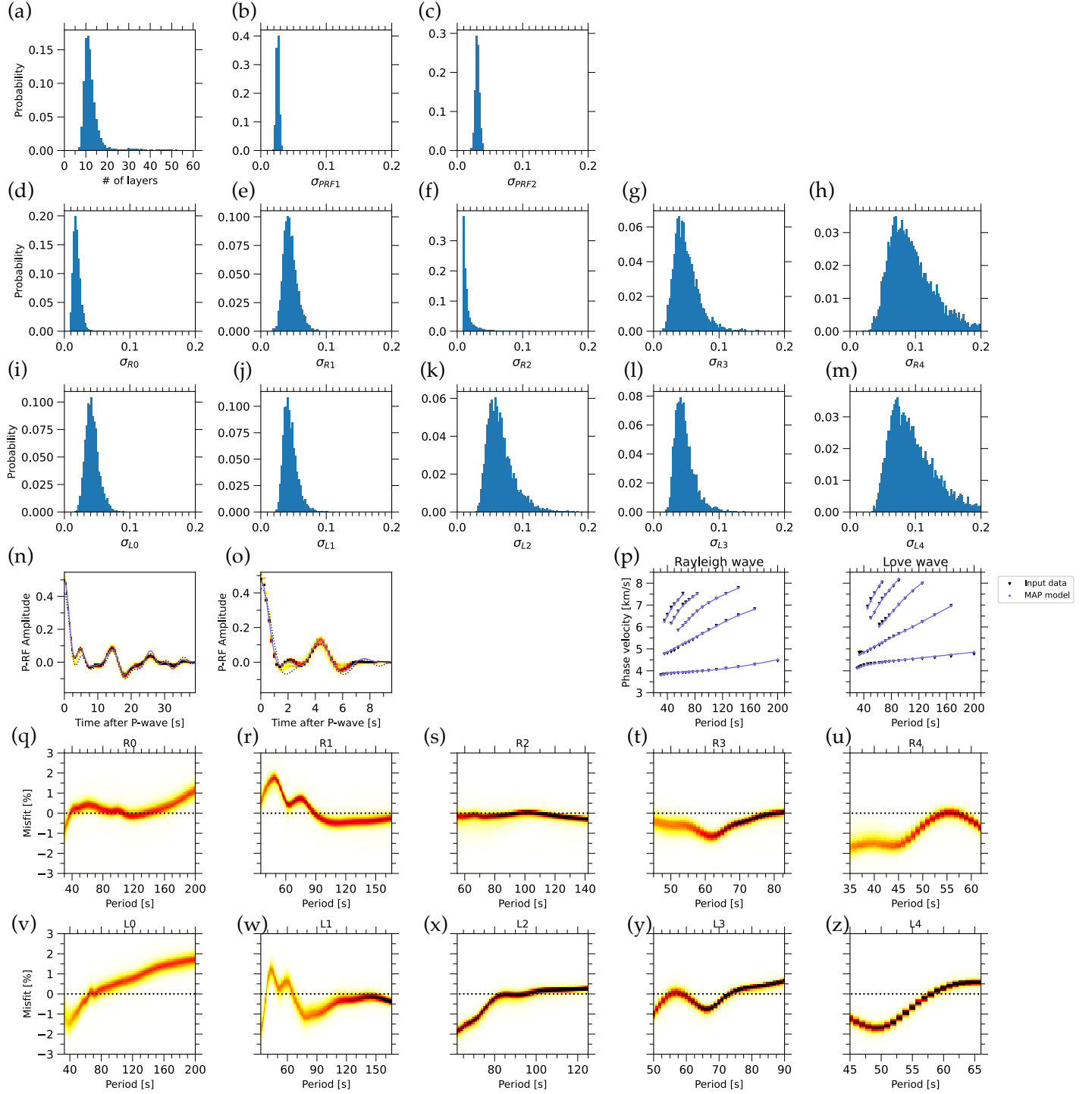
Figure S9: Same as Figure S7, but for the northern event group (Figure 5 (d) in the main text).
