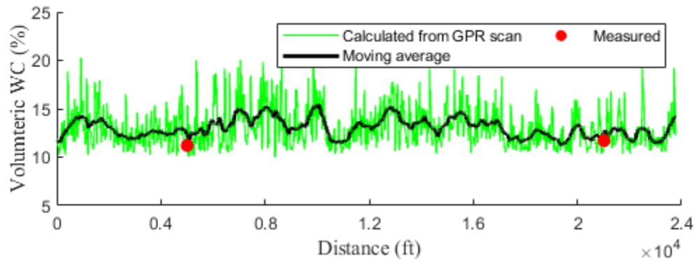
(b) Volumetric water content profile of the SH-24 test site
