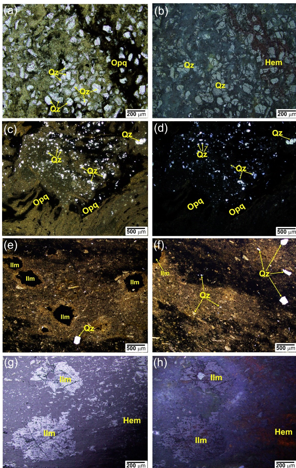
665 Figure 3. Photomicrographs of Ernestite thin sections: (a) sample from Dholavira in plane- 666 polarized transmitted light showing the presence of quartz (Qz) and opaques (Opq); (b) same 667 as in (a) with hematite (Hem) displaying characteristic red internal reflection under reflected 668 lights; (c-d) sample from Bhagatrav in plane-polarized and cross-polarized transmitted lights; 669 (e-f) sample from Kanmer showing detrital ilmenite (Ilm) and quartz (Qz) in plane-polarized 670 transmitted light; (g-h) sand-sized ilmenite (Ilm) grains and hematite (Hem) patches in the 671 same sample as in (e) in plane and crossed polarized reflected lights, respectively.
