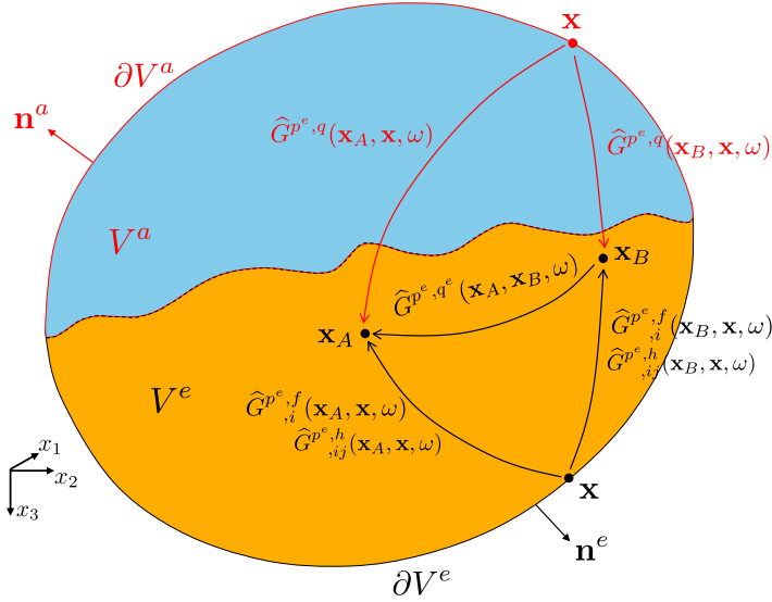
Figure 4. Pressure-type Green's function representation through interferometry when both the receivers are in V^e . According to eq. (60), the Green's function \widehat{G}^{p^e, q^e}(\mathbf{x}_A, \mathbf{x}_B, \omega) can be obtained by cross-correlating the observations at \mathbf{x}_A and \mathbf{x}_B , and integrating along the source coordinate \mathbf{x} at \partial V^a and \partial V^e . The wavefields observed at \mathbf{x}_A and \mathbf{x}_B , along with the corresponding sources required at \mathbf{x} on \partial V^a and \partial V^e for Green's function \widehat{G}^{p^e, q^e}(\mathbf{x}_A, \mathbf{x}_B, \omega) retrieval, are shown. Note that the rays in this figure represent the full responses between the source and receiver points, including primary and multiple scattering, as well as mode conversion due to inhomogeneities inside and outside the region \partial V^a \cup \partial V^e .
