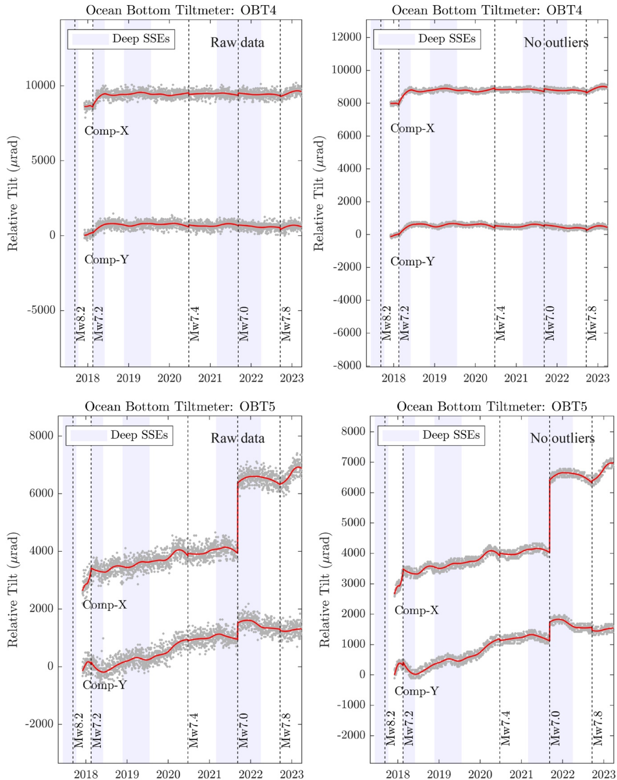
Fig. S12. Two-component raw tilt data (left column) with 24 h sampling rate and tilt data after outlier removal (right column) at our four ocean bottom tiltmeters. Red curves are locally weighted regression functions (fLOESS) using a 2nd order polynomial with a window support of 250 samples. Regressions are performed independently for each earthquake bounded period, so that
