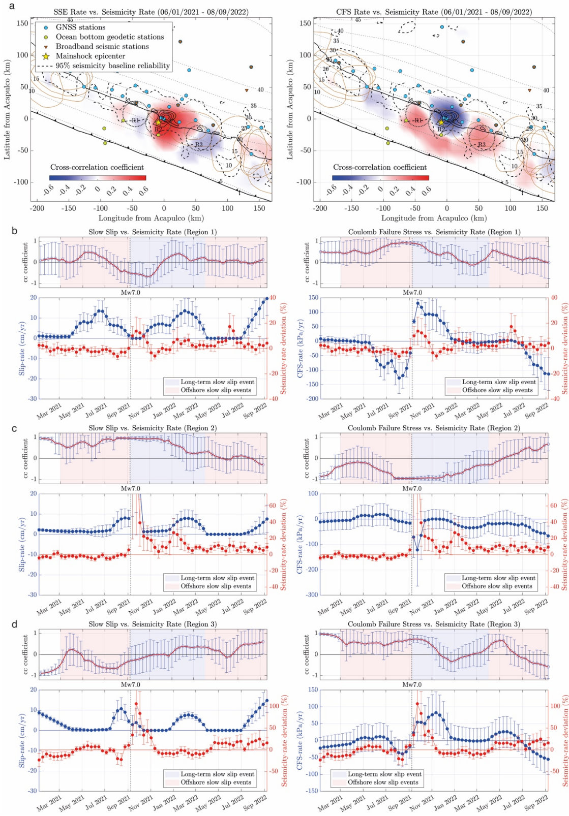
Fig. S24. Correlation analysis between the seismicity rate and both, slip rate (left column) and Coulomb failure stress (CFS, right column) at the plate interface. (a) Average over 1.3 years (see
