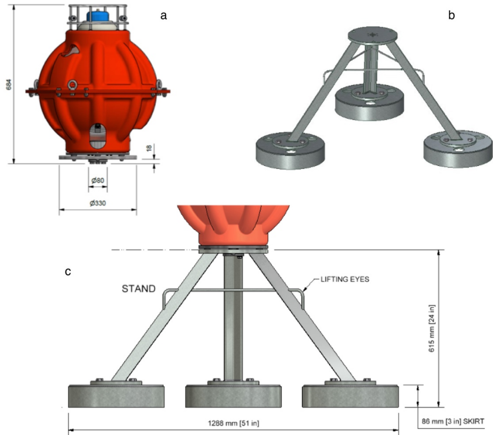
Fig. S10. Sonardyne Co Fetch unit dimensions and configuration. (a) Plastic covering (orange) of the glass sphere and transducer (blue). (b) and (c) show the steel tripod on which the glass sphere is mounted.
