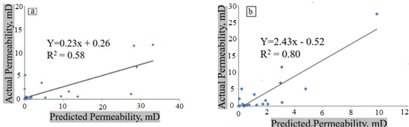
Figure 4. (a) Predicted permeability from the initial Winland model. (b) Predicted permeability from the calibrated Winland model.
