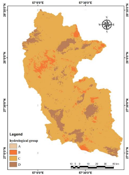
Figure3. Hydrological groups of the study area
