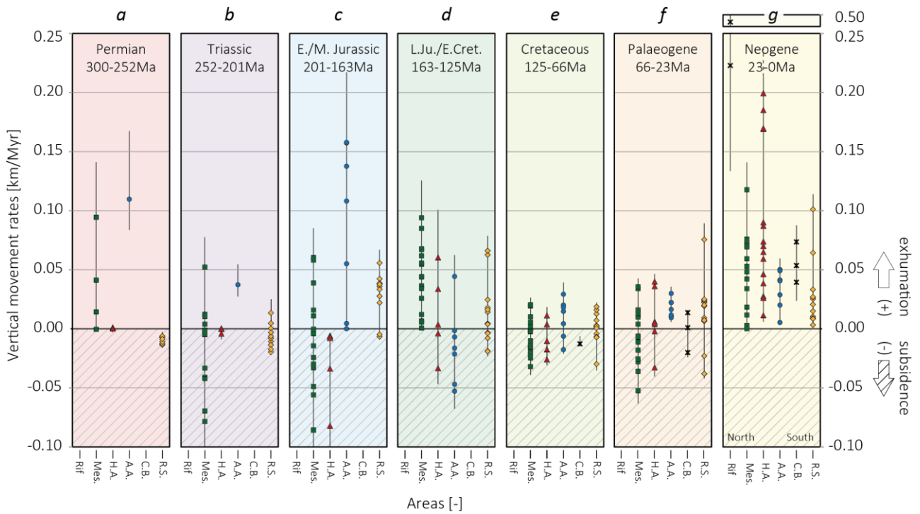
Figure 6. Exhumation and subsidence rates calculated from the 56 selected depth converted curves of figure 5 using the variable geotherms shown in figure A1. The seven defined periods a to g span between 300 and 0 Ma. The combined uncertainties are extracted from the results of rate calculations using constant geotherms. Mes : Meseta; HA : High Atlas; AA : Anti-Atlas; CB : Coastal Mesozoic basins; RS : Reguibat Shield. Areas, especially if substantially large, may have experienced both exhumation and subsidence, and must not necessarily be an error from the initial t-T models. North and South are only marked for period g because Morocco has been significantly rotated since the Permian (e.g. Scotese, 2012). Note that the x-axis is not time.
