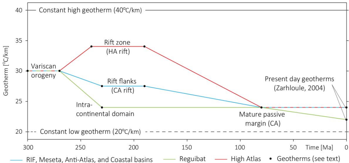
— RIF, Meseta, Anti-Atlas, and Coastal basins — Reguibat — High Atlas • Geotherms (see text) Figure A1. Geothermal gradients used for the depth conversion of the t - T curves. Geotherms: Geothermal gradients documented in literature, from present-day or recent settings similar to ones in Moroccan geological past. See description of the geotherms considered as analogues in the text of Appendix A.
