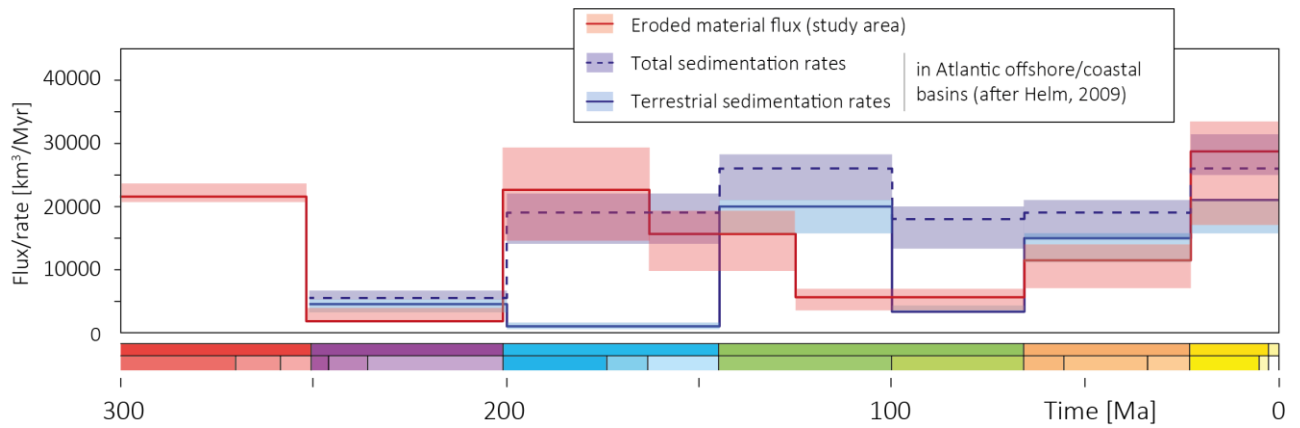
Figure 19. Comparison of the total eroded material flux to sedimentation rates in Moroccan offshore and coastal basins (after Helm, 2009). Note that it may be expected that the results should not match perfectly, as a proportion of the eroded material would be removed as dissolved carbonate or as fines that would have long transport distance into the deep oceanic basins (i.e. eroded material flux – red line v terrestrial sedimentation rates - blue).
