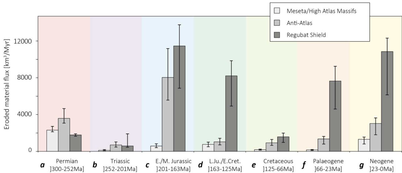
Figure 8. Estimated eroded material flux for the three main sediment sources (Meseta/High Atlas, Anti-Atlas, and Reguibat Shield) for the seven defined periods ( a-g ). The eroded material flux is obtained with variable geotherms (Appendix A), while the ranges are given by calculations done with two constant geotherms of 20 and 40°C/km.
