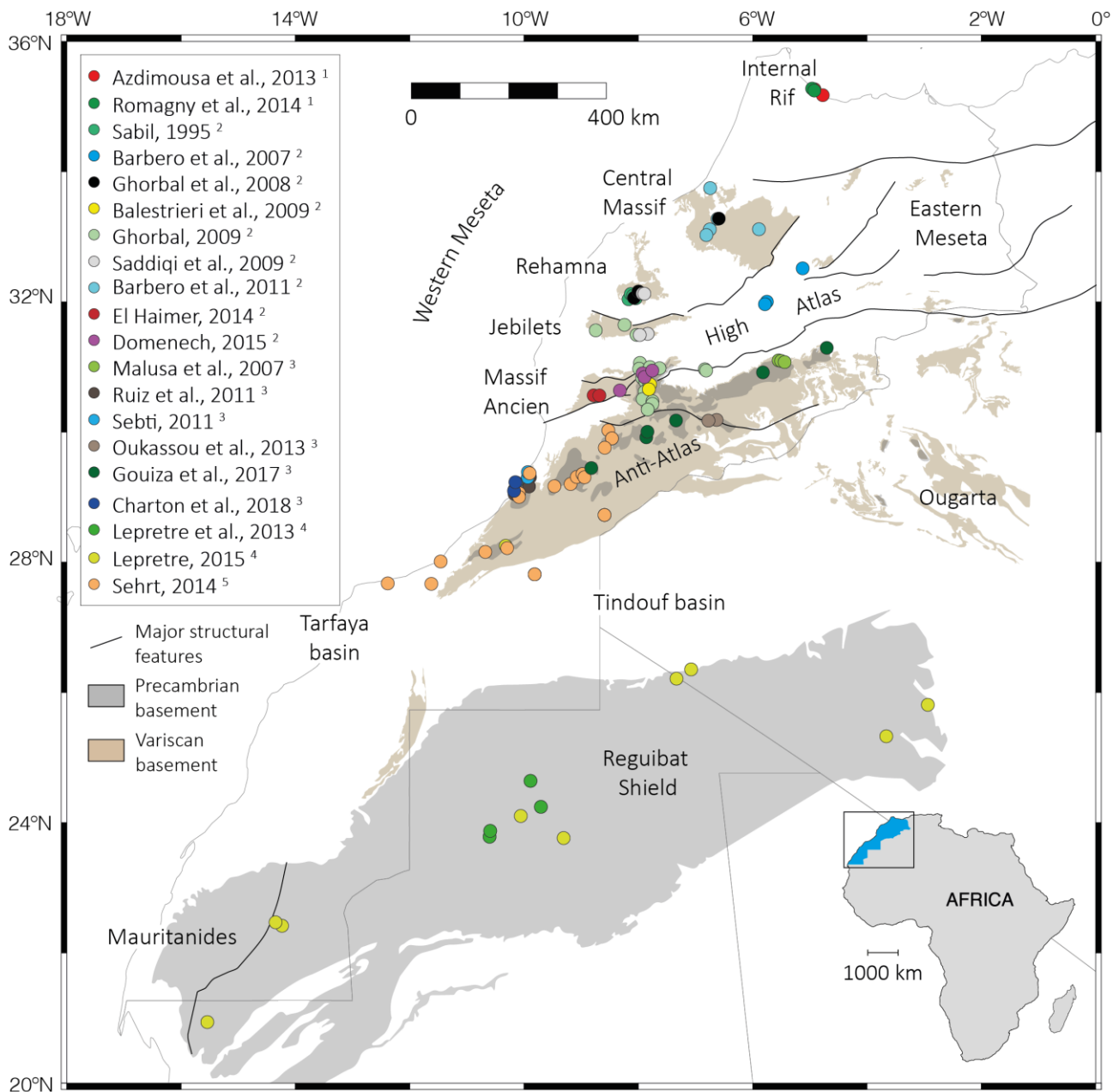
Figure 3. Location of samples used for t-T modelling, located in the Rif 1 , the Meseta and High Atlas 2 , the Anti-Atlas 3 , the Reguibat Shield 4 , and the western Anti-Atlas and north Tarfaya Basin 5 (see reference details in table A).
