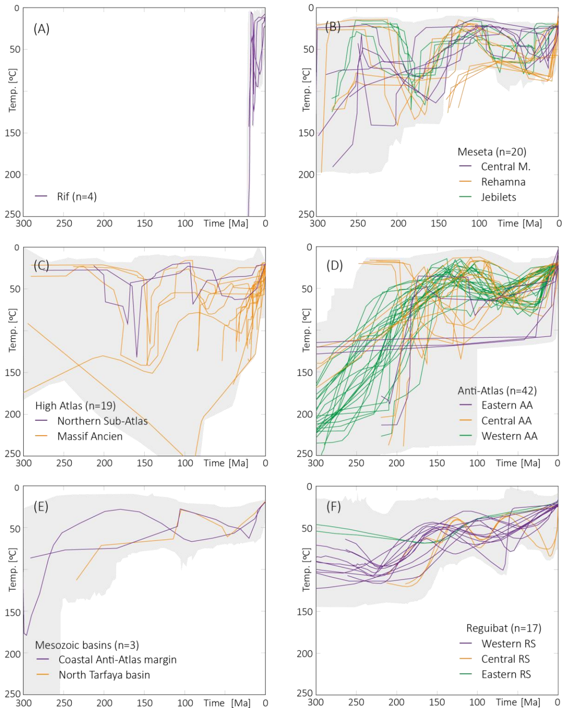
Figure 4. Digitized t-T modelling weighted averages, best-fit curves, and acceptable envelopes (grey area) for HeFTy results or expected curves, maximum likelihood curves and limits of 2\sigma confidence level (grey area) for QTQt results (see references in Appendix A). t-T results for borehole samples from Sehart (2014), as well as results from El Haimer (2014) and Barbero et al. (2007), for which only envelopes were published, were not included.
