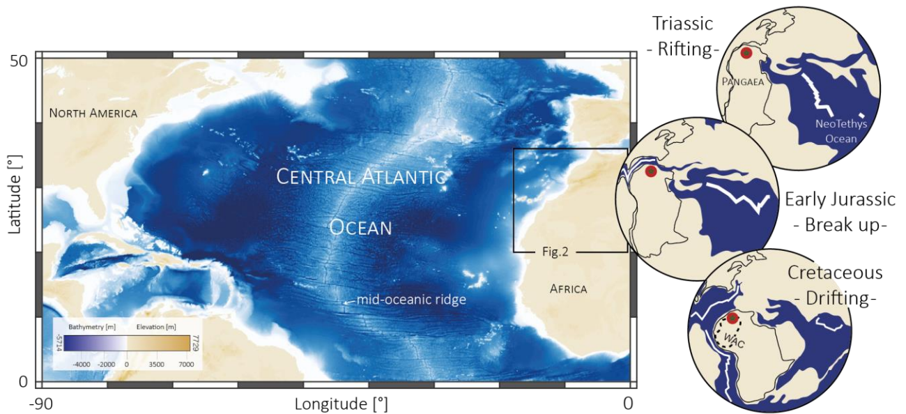
Figure 1. Morphology of the Central Atlantic seafloor and conjugate margins (data: GEBCO_2014_1D).
