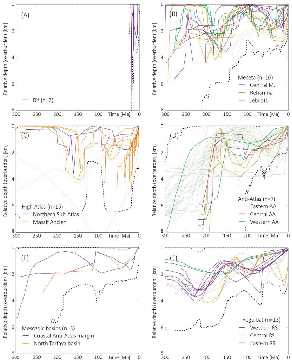
Figure 5. Time-depth curves converted from t-T curves shown in figure 4, assuming geothermal gradients evolving as illustrated in appendix A and assuming a surface temperature of 20°C. The thicker lines display vertical movement rate calculations; non-selected thinner curves, in the backgrounds, were also converted to depth but were not used in the later study; conditions for result selection are detailed in appendix A. The upper and lower limits (thick dashed lines) are calculated with geothermal gradients of 40 and 20°C/km, respectively.
