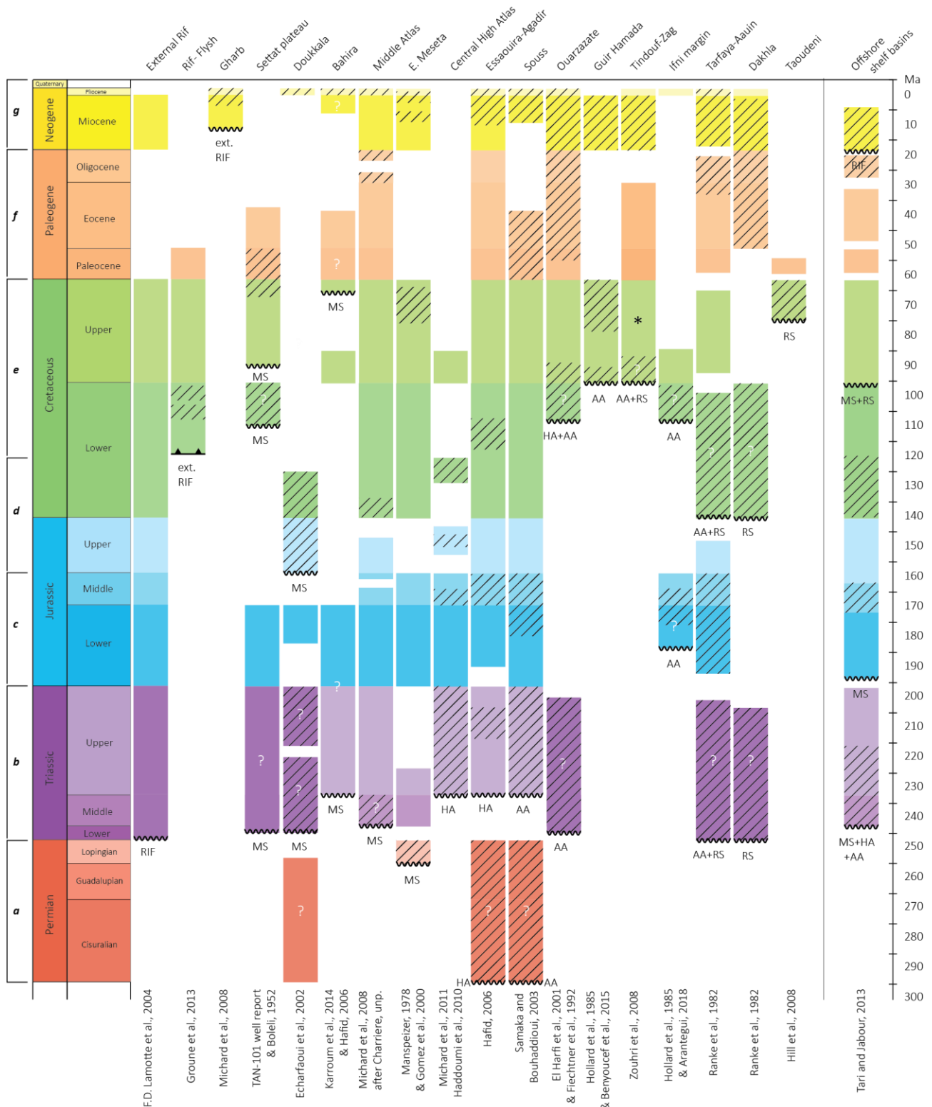
Figure A2. Simplified stratigraphic columns. The hatched parts highlight continental facies and/or coarse to very coarse clastic deposits. The name of the corresponding Variscan/Precambrian basement is shown below the unconformity surfaces (MS: Meseta, HA: High Atlas, AA: Anti-Atlas, and RS: Reguibat shield basements). The seven selected periods (a to g) are shown on the left. *Late Cretaceous in the Tindouf basin is present in the eastern and western parts, but not in its central part (Hollard et al., 1985).
