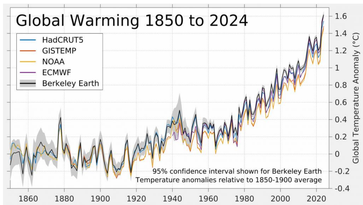
Figure 1. © Berkeley Earth, 2025.
