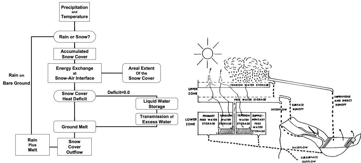
FIGURE 3 SNOW-17 diagram (left) from National Weather Service (2006) and SAC-SMA diagram (right) from National Weather Service (2002a).
