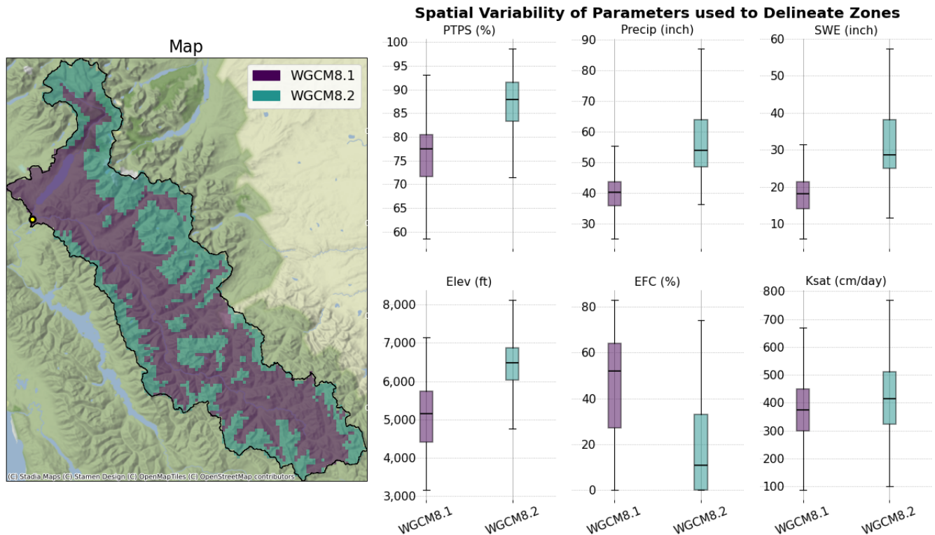
FIGURE 5 Example basin delineation using k-means clustering for the Middle Fork of the Flathead River near West Glacier, Montana. WGCM8.1 and WGCM8.2 indicate the two zones where zone 1 typically corresponds to lower elevations with the shortest travel time to the outlet. The yellow dot indicates the basin outlet.
