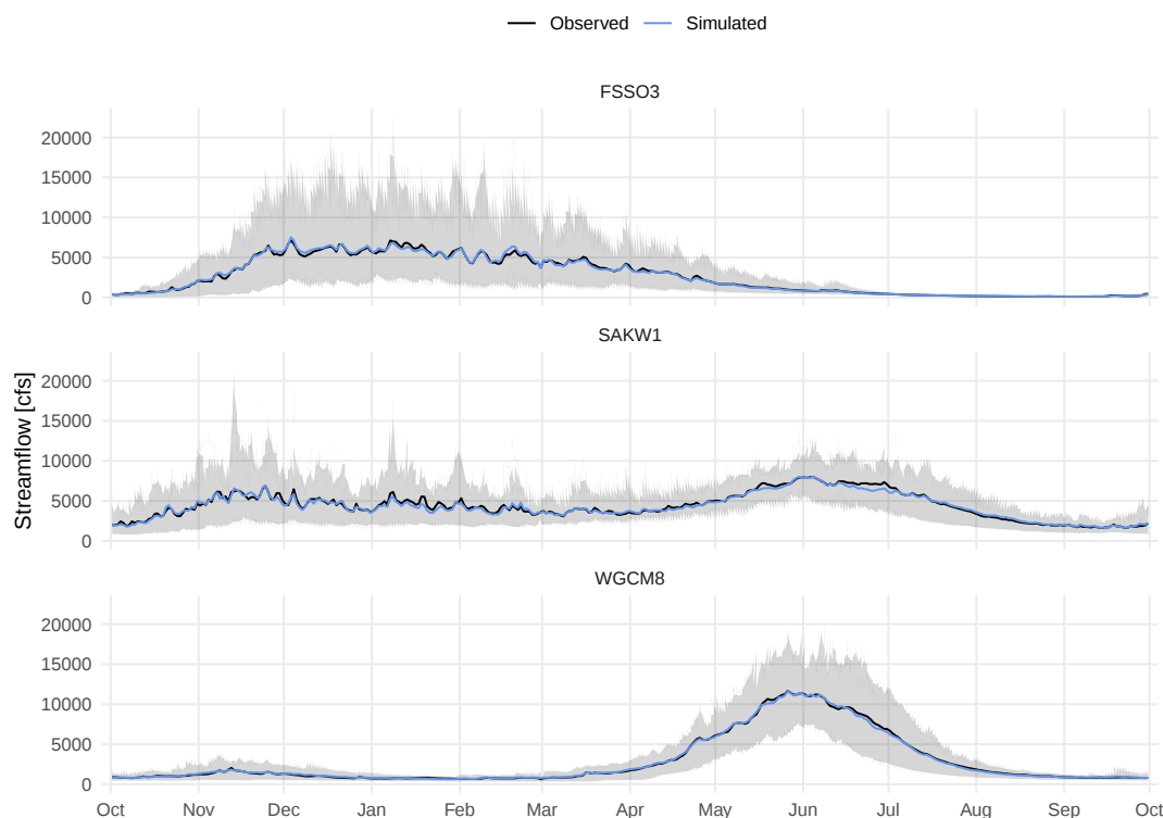
FIGURE 10 Cyclical streamflow plots showing the daily hydrologic regime from 1980 to 2022. The black line represents the median observed streamflow, while the blue line represents the median simulated streamflow. The grey shaded area indicates the 10th to 90th percentile range of the simulations.
