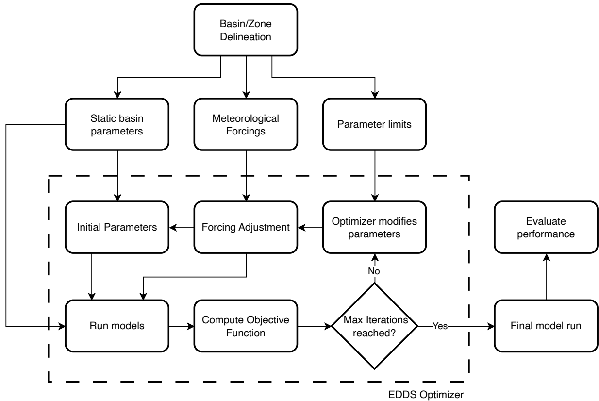
FIGURE 4 Flowchart of the NWRFC auto-calibration processes for utilization of the EDDS optimizer.
