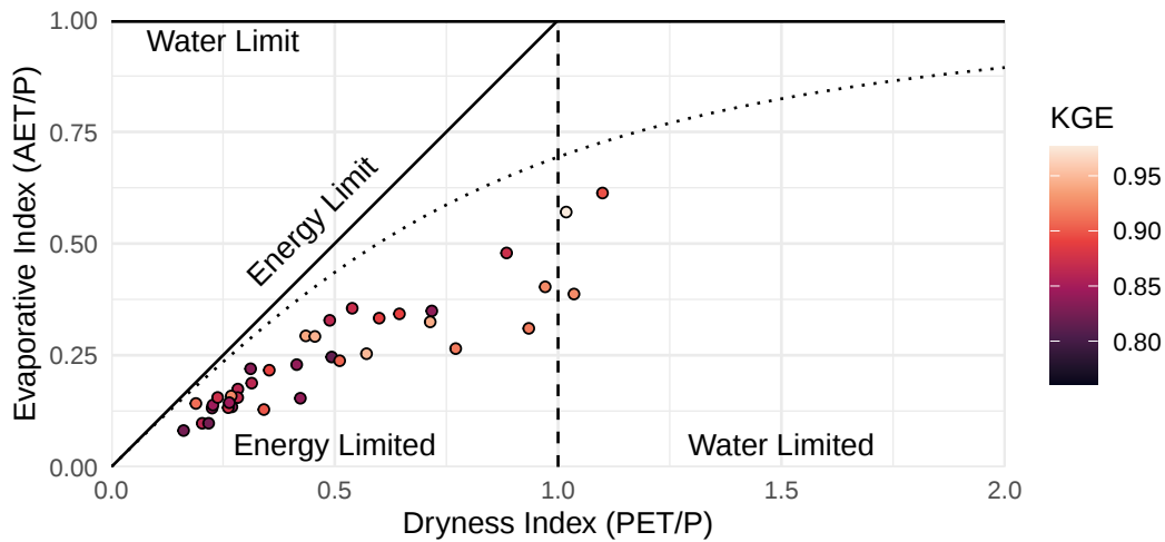
FIGURE 8 Budyko diagram showing long term behavior of the calibrated simulations for each zone of the three test basins. AET = Actual Evapotranspiration, P=Precipitation, PET=Potential Evapotranspiration, where all values represent long term annual averages, typically 10 years or more.
