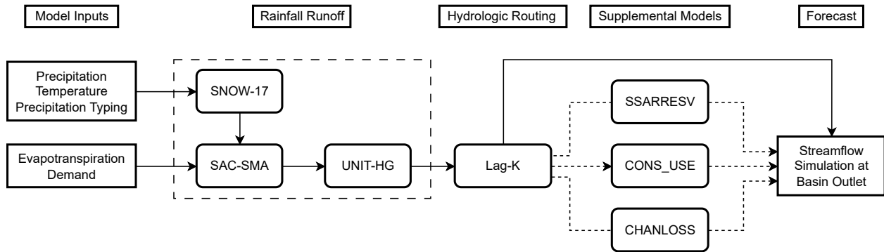
FIGURE 2 The operational models used by the NWRFC for forecasting. See Section 2 for complete details on each model.
