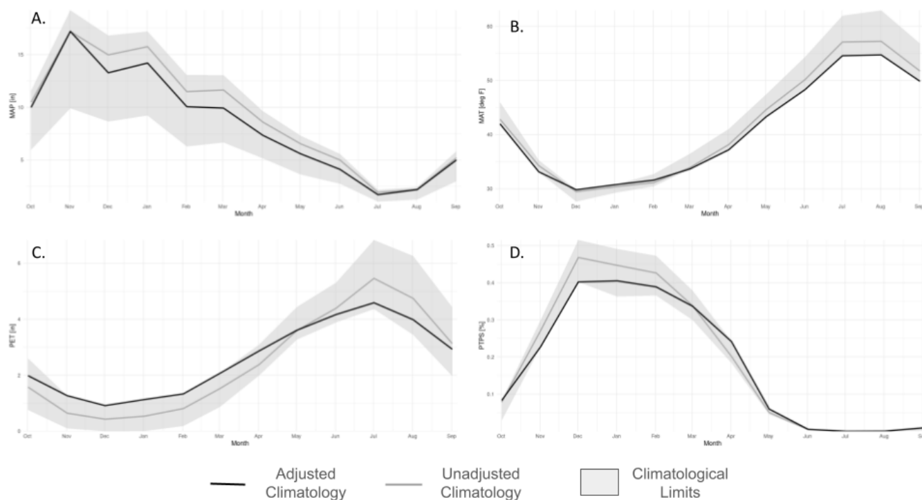
FIGURE 6 Examples of climatological monthly forcings before (grey line) and after adjustments (black line) applied through optimization during the auto-calibration routine. Imposed climatological limits used during optimization are also displayed (shaded area). A. precipitation (MAP), B. air temperature (MAT), C. evapotranspiration (PET), and D. precipitation typing (PTPS)
