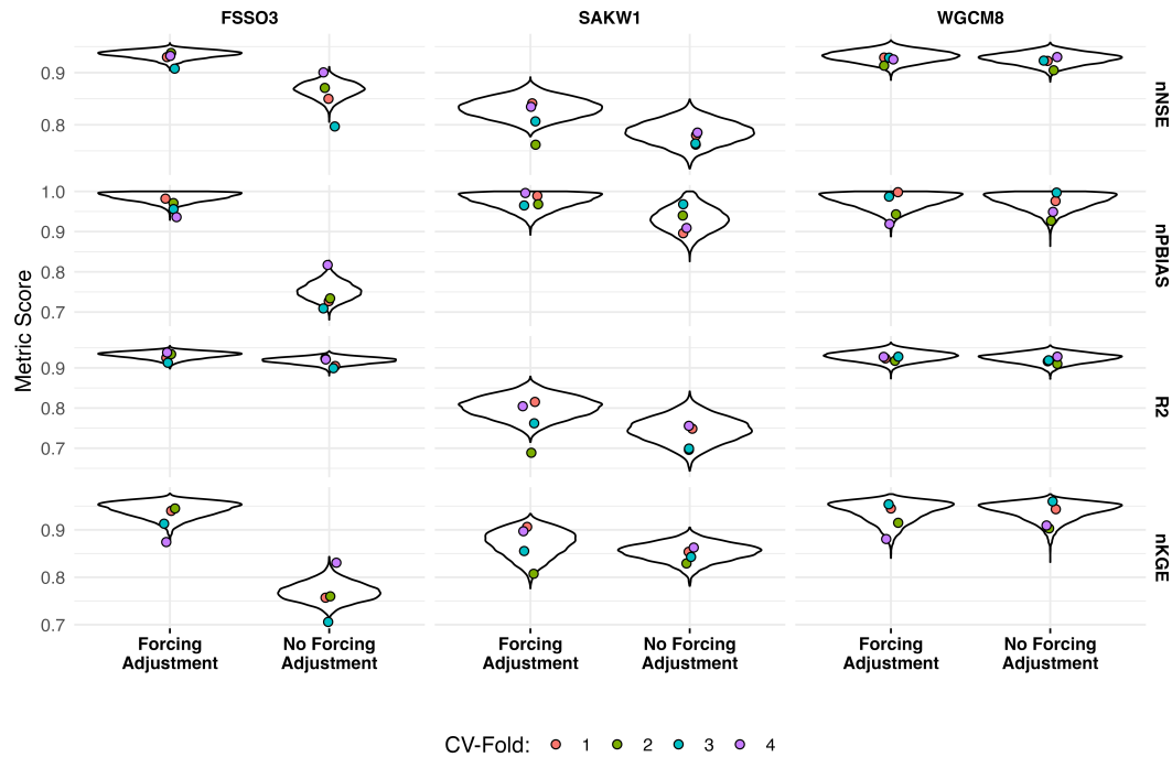
FIGURE 11 Cross validation (points) and POR bootstrapping (violin plots) metric scores with and without using climatological forcing adjustments
