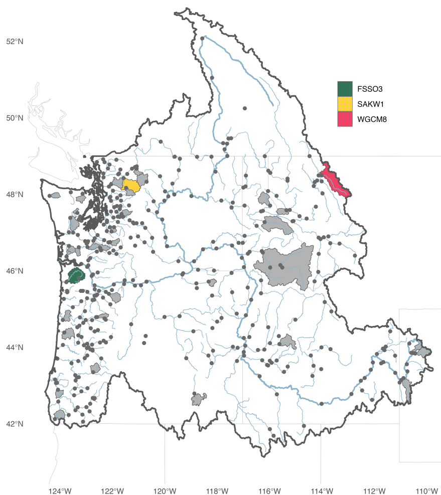
FIGURE 1 Map of the NWRFC domain (thick black outline), forecast points (black dots), and primary river reaches (blue lines). The mainstems of the Columbia and Snake Rivers are highlighted with increased line weight. CAMELS basins are shaded grey, while the three case-study basins are highlighted in color.
