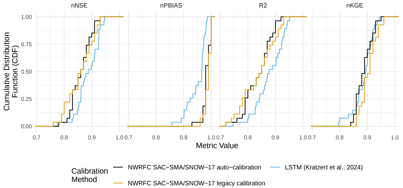
FIGURE 7 CDF of metrics scores from 27 basins in the NWRFC domain comparing NWRFC calibrations and metrics from a trained LSTM model from Kratzert et al. (2024). All basins are part of the CAMELS dataset. See Appendix A for definitions of the normalized metrics as well as tables of metrics for each basin.
