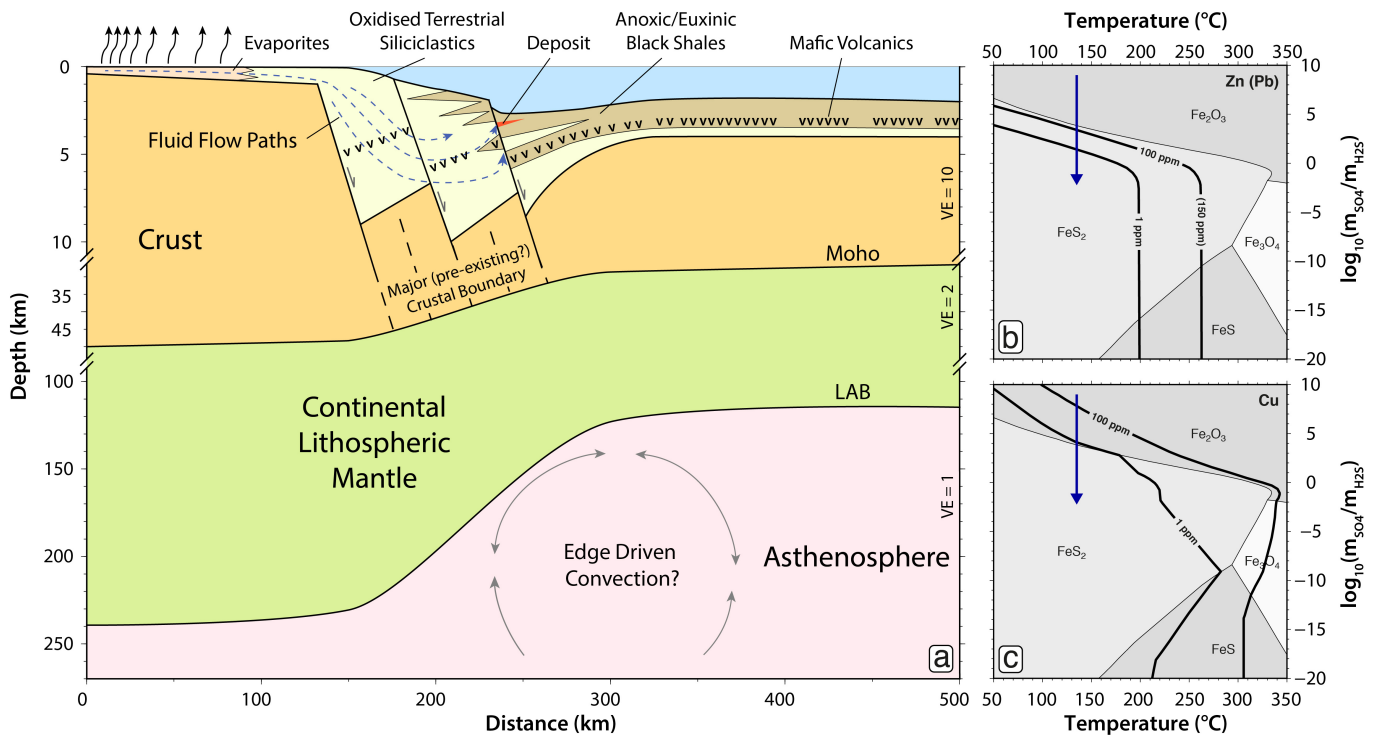
Figure 1: Mineralisation system for genesis of sediment-hosted base metal deposits. (a) Schematic illustration of deposit location in extensional rift settings. Basinal brines sourced from evaporites scavenge metals from oxidised terrestrial sediments and volcanics (v) on route to metal deposition sites in black shales. 23 Notice variable vertical exaggeration (VE) and prominence of the lithosphere-asthenosphere boundary edge illustrated at 1:1 scale. Schematic based on architectural constraints from the Australian Carpentaria Zinc Belt and Polish Fore-Sudetic Block. (b) Stability field of Fe-S-O minerals as a function of temperature and redox conditions; m_{SO_4} = molarity of sulphate; m_{H_2S} = molarity of sulphide; thick black lines = solubility of zinc (and lead) in brine, 24 calculated for fluid salinity = 10 wt.% NaCl, total concentration of sulphur species = 10^{2.5} M, and pH = 4.5; blue arrow = fluid path for metal precipitation by oxidation-reduction deposition mechanism. (c) Same for copper solubility.
