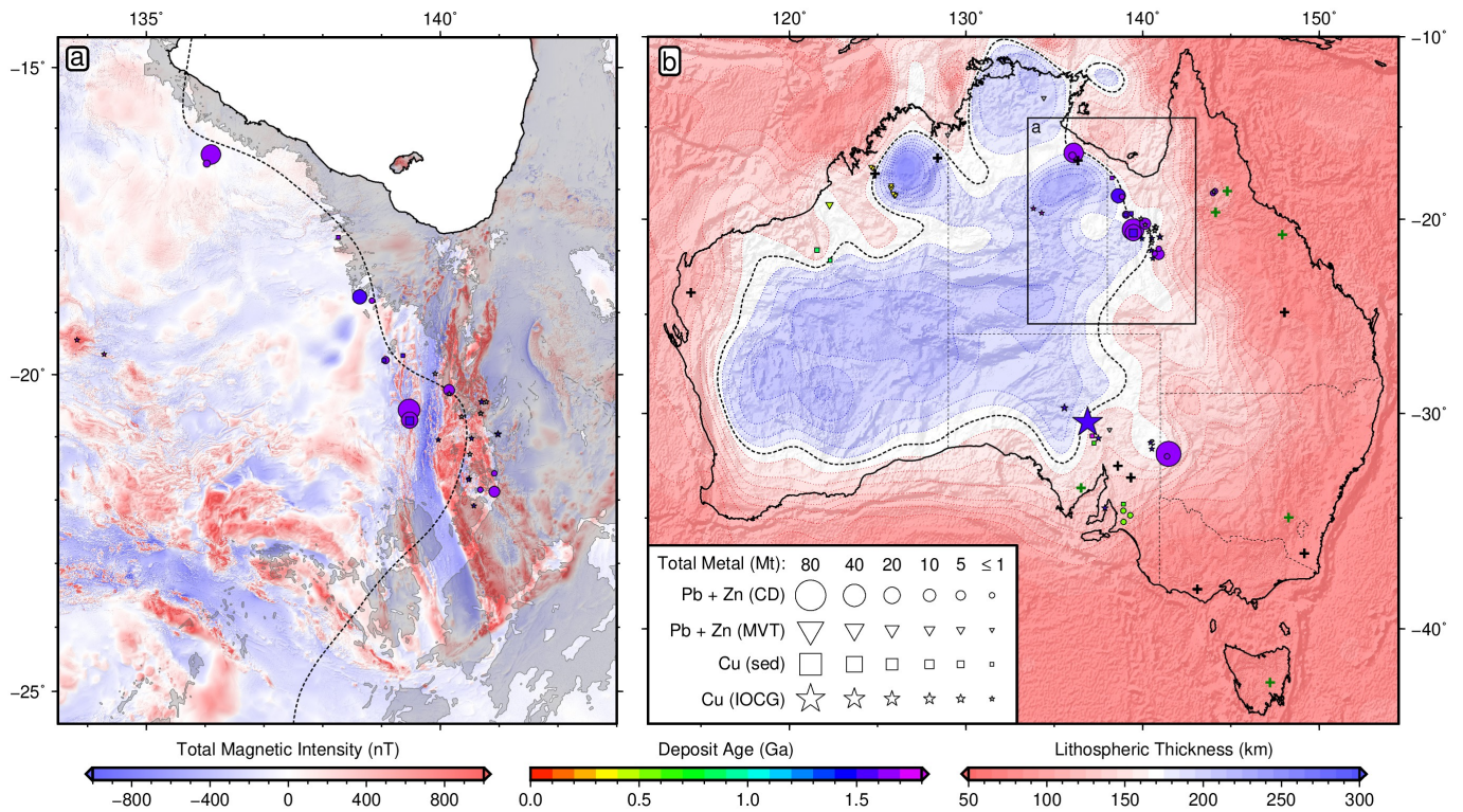
Figure 2: Distribution of sediment-hosted and iron-oxide-copper-gold base metal deposits as a function of lithospheric thickness in Australia. (a) Carpentaria Zinc Belt; red/blue = variably reduced to pole aeromagnetic intensity data 26 ; grey polygons = generalised outcrop of Cretaceous marine sediments in Eromanga and Carpentaria Basins; 128 black dashed contour = 170 km LAB thickness; symbols = deposit locations; area proportional to estimate of total contained mass of metal (Mt = megatonnes); unknown deposit size given 1 Mt symbol; colour = ore body formation age (billion years); unknown age plotted in grey; circles = clastic-dominated lead-zinc (PbZn-CD); triangles = Mississippi Valley type lead-zinc (PbZn-MVT); squares = sedimentary copper (Cu-sed); stars = iron-oxide-copper-gold (IOCG). Large star in South Australia shows location of the Olympic Dam deposit. (b) Australian LAB mapped by converting FR12 tomography 29 to temperature using an anelasticity parameterisation 28 calibrated on local paleogeotherms (Methods) and illuminated by free-air gravity anomalies 26 ; black/green crosses = geotherms used as constraints/tests in anelasticity calibration (Supplementary Information); box = location of panel (a).
