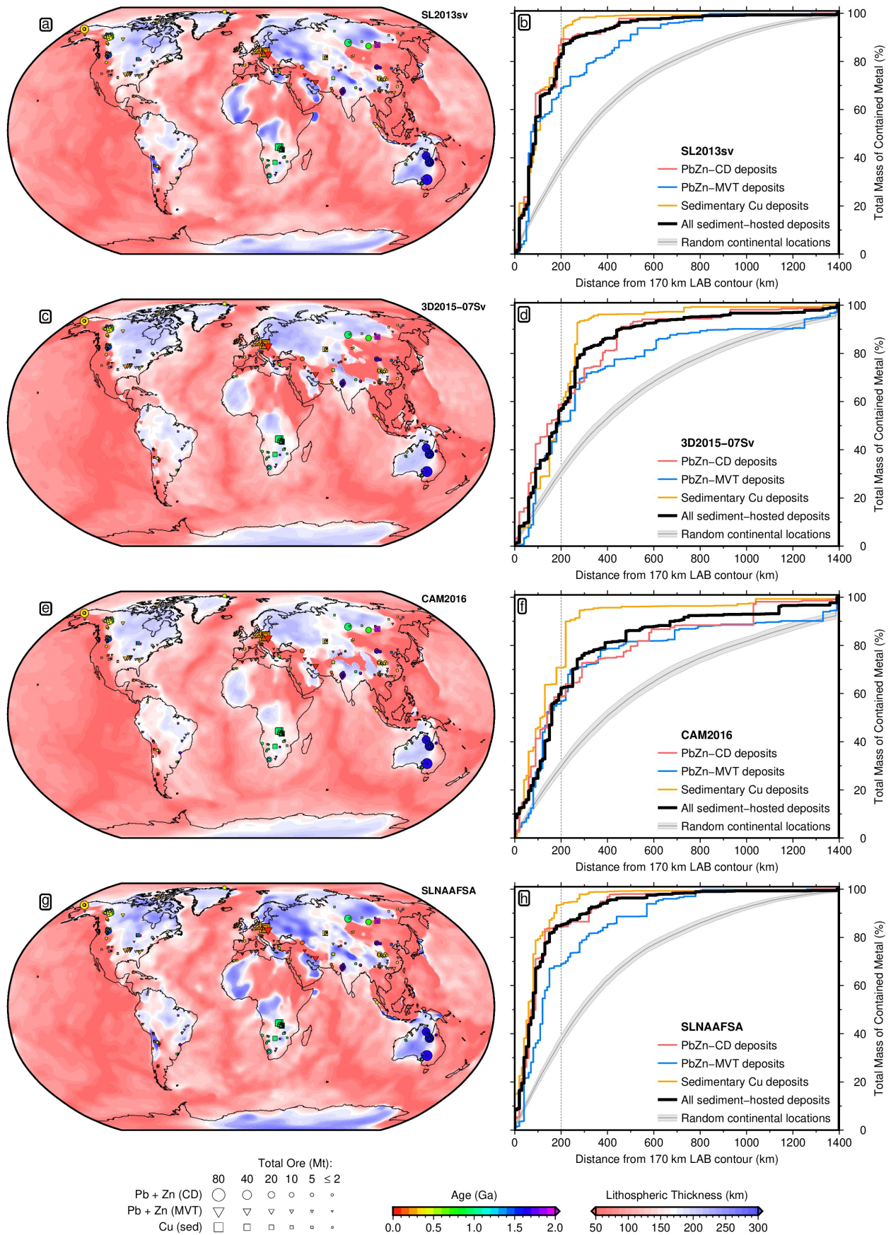
Figure Extended Data Figure 1: Global lithospheric thickness maps obtained from calibration of four upper mantle surface wave tomography models. (a) SL2013sv model. 30 Symbols = deposit locations; area proportional to estimate of total contained mass of metal (Mt = megatonnes); unknown deposit size given 2 Mt symbol; colour = ore body formation age (billion years); unknown age plotted in grey; circles = clastic-dominated lead-zinc (PbZn-CD); triangles = Mississippi Valley type lead-zinc (PbZn-MVT); squares = sedimentary copper (Cu-sed). (b) Associated CDFs for sediment-hosted deposits and random continental locations. (c-d) Same for the 3D2015-07Sv model. 70 (e-f) Same for the CAM2016 model. 71,72 (g-h) Same for the SLNAAFSA model, generated by blending regional updates from North America (SL2013NA 73 ), Africa (AF2019 74 ), and South America (SA2019 75 ) into the global SL2013sv model. 30 Note that CDFs for all tomography models show a significant difference from the distribution of random continental locations.
