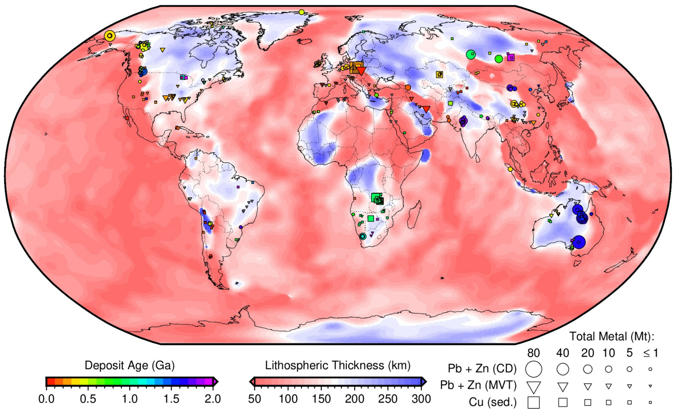
Figure 3: Global distribution of sediment-hosted base metal deposits as a function of lithospheric thickness. LAB derived from SL2013sv tomography model 30 using a calibrated anelasticity parameterisation 28 (Methods). Symbols = deposit locations; area proportional to estimate of total contained mass of metal (Mt = megatonnes); unknown deposit size given 1 Mt symbol; colour = ore body formation age (billion years); unknown age plotted in grey; circles = clastic-dominated lead-zinc (PbZn-CD); triangles = Mississippi Valley type lead-zinc (PbZn-MVT); squares = sedimentary copper (Cu-sed).
