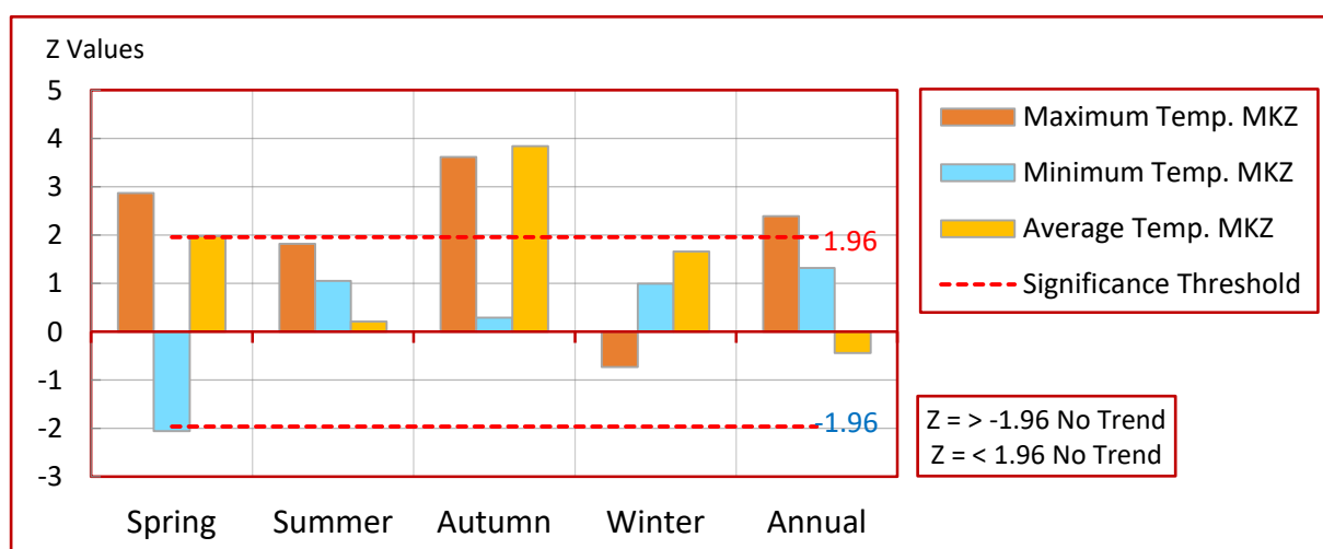
Figure 3. Z-values of the Mann-Kendall Test for maximum, minimum, and average temperatures in the Al-Berdi region during the period 1985–2022.
