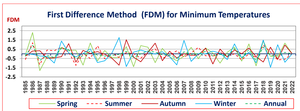
Figure 7. Seasonal and annual Minimum temperatures in the Al-Berdi region analyzed using the Finite Difference Method (FDM).
