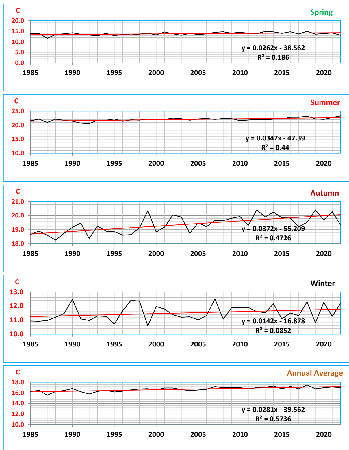
Figure 5. Seasonal trend analysis of minimum temperatures in the Al-Berdi region based on the simple linear regression method.
