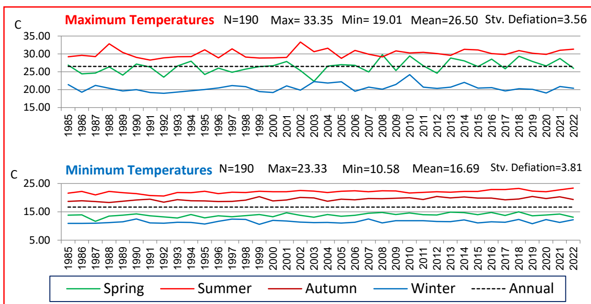
Figure 2. Seasonal and Annual Maximum and Minimum Temperatures in the Al-Berdi region.
