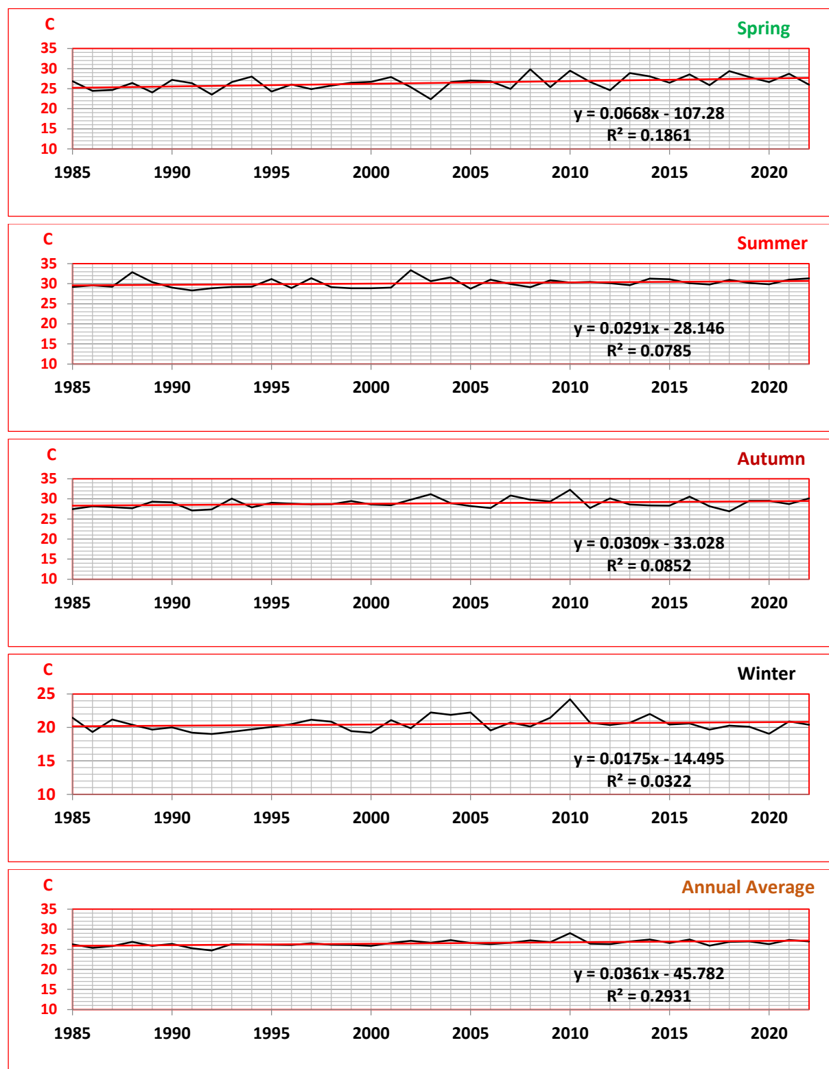
Figure 4. Seasonal trend analysis of maximum temperatures in the Al-Berdi region based on the simple linear regression method.
