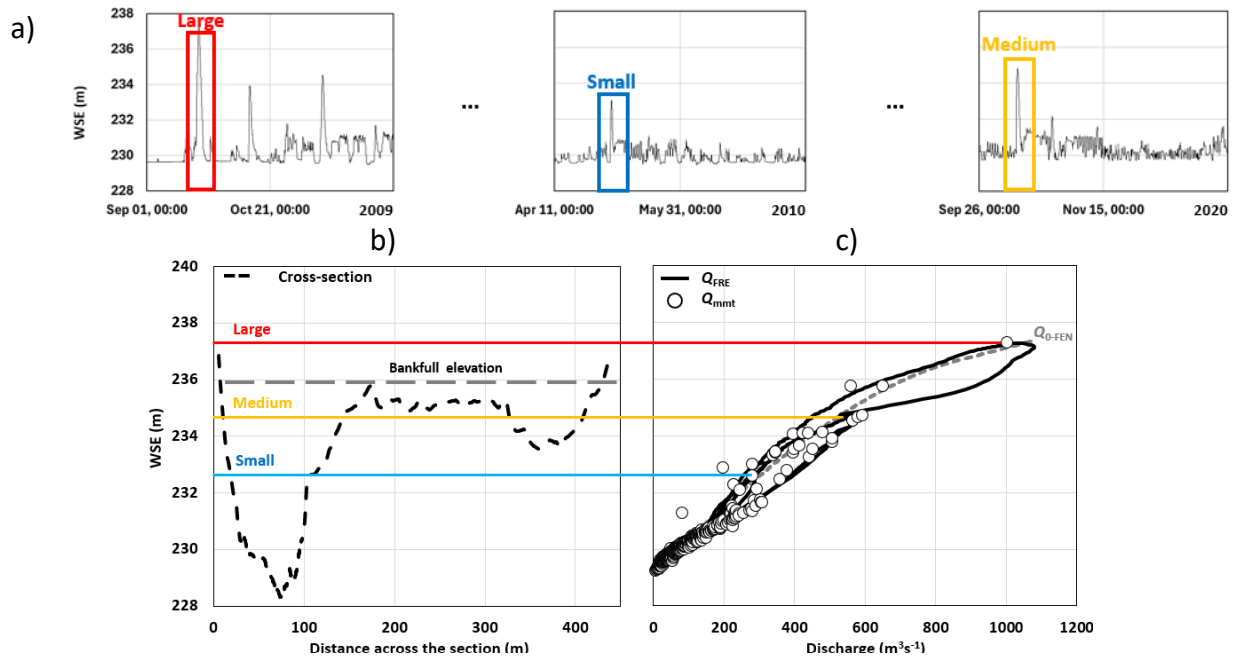
Figure 3. Key analysis elements for the Atlanta station: (a) selected storm events; (b) maximum event stages superposed on the channel cross-section; and (c) reference HQRC ( Q_{0-FEN} ) and Fread-corrected discharge ( Q_{FRE} ).
