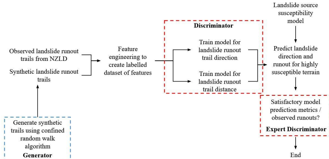
Figure 3: GAN inspired model architecture for landslide debris trail prediction
