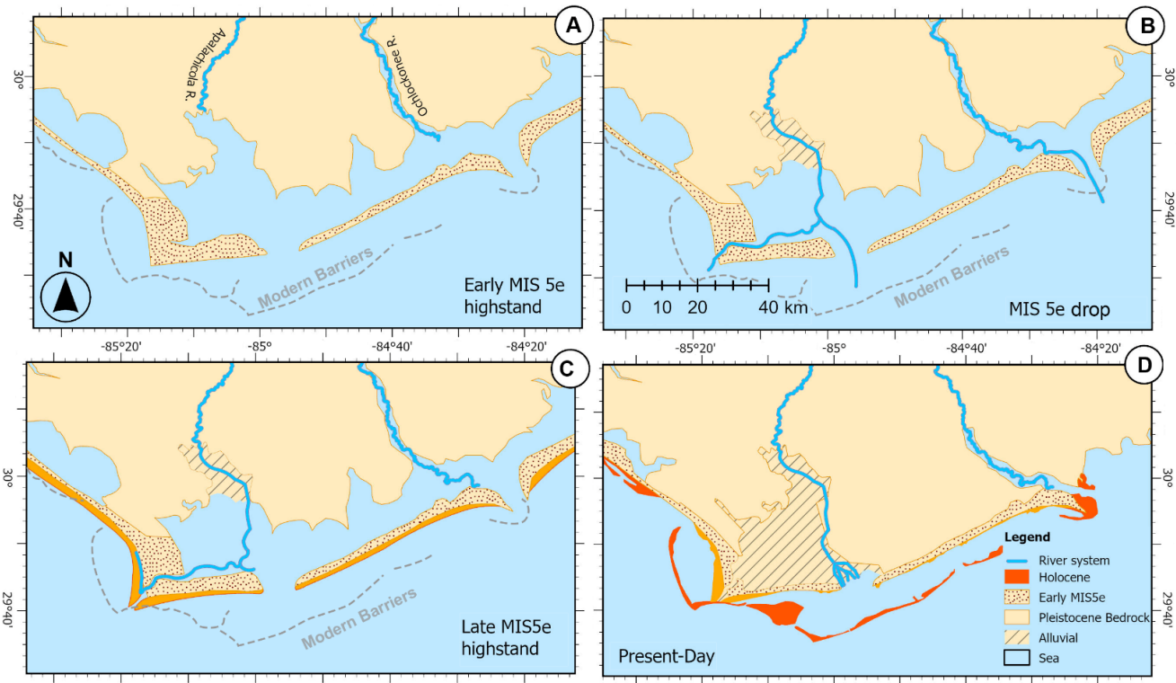
Figure 9. Evolution of the Apalachicola coastal barrier system since the Last Interglacial (MIS5e). A) Early MIS 5e highstand; B). MIS5e drop, C) Late MIS5e highstand, D) Present-day coastal morphology.
