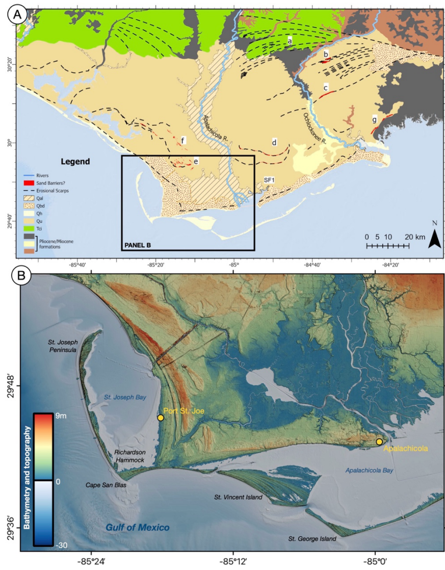
210 Figure 3. A) Geologic map of the Apalachicola barrier system (from Scott et al., 2001). Red polygons mark sand barriers; dashed black line marks distinct geomorphological features based on the results of former studies. Labels a-g correspond to locations of geomorphological features shown in Figure 4. Label SF1 marks the location of the geomorphological feature represented in Supplementary Figure 1. Legend of geological formations: Qh = Quaternary Holocene Sediments; Qbd = Quaternary Beach Ridge and Dune; Qal = Quaternary Alluvium; Qu = unconsolidated and undifferentiated sediments; Tci = Citronelle Formation. 215 B). Digital elevation model of the study area (NOAA National Centers for Environmental Information, 2023; US Geological Survey, 2011) with toponyms mentioned in the text and main towns.
