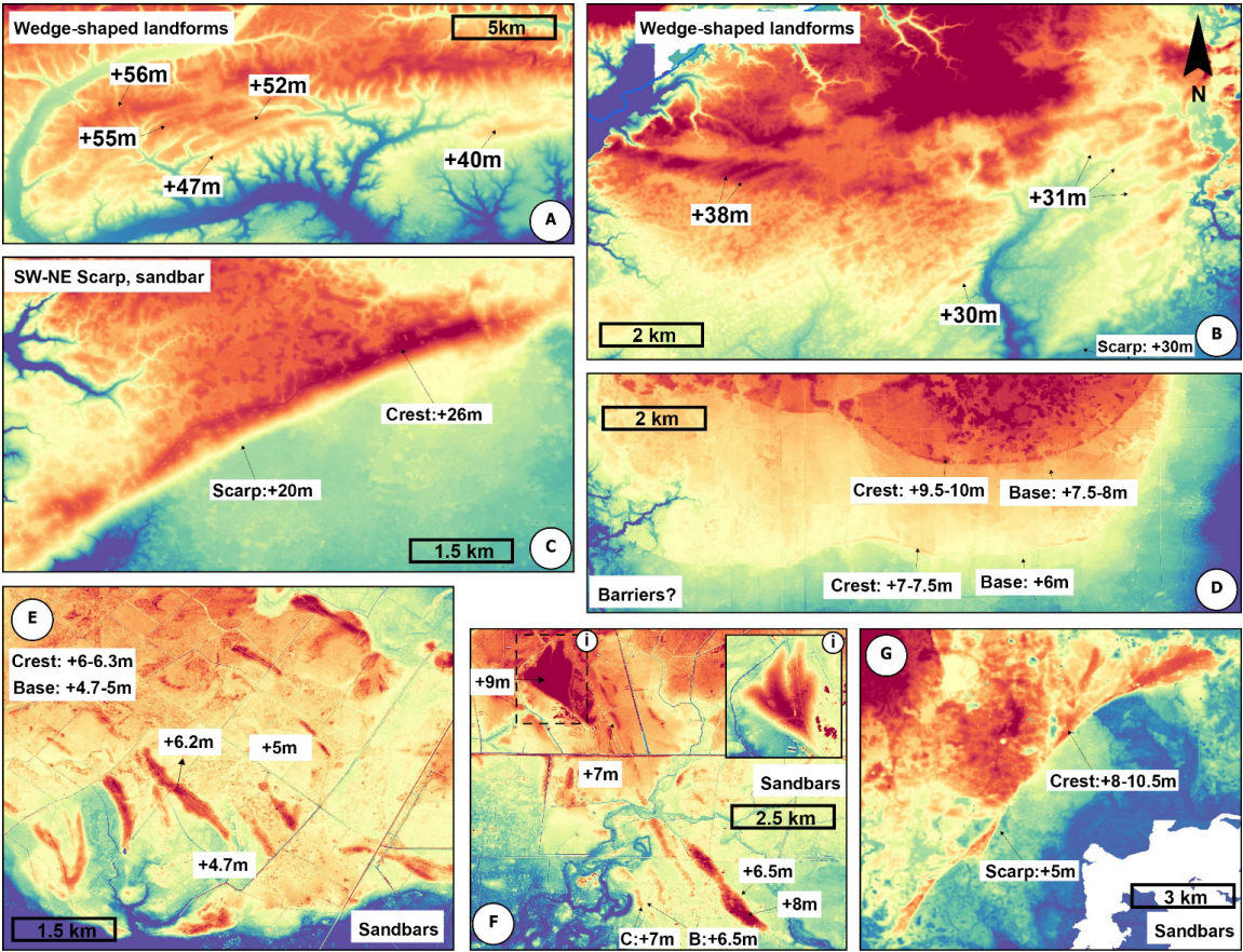
Figure 4. Distinct geomorphological features related to coastal depositional/erosional features. The location of each panel is shown in Figure 3A. Elevation data from 1-meter DEMs (US Geological Survey, 2022).
