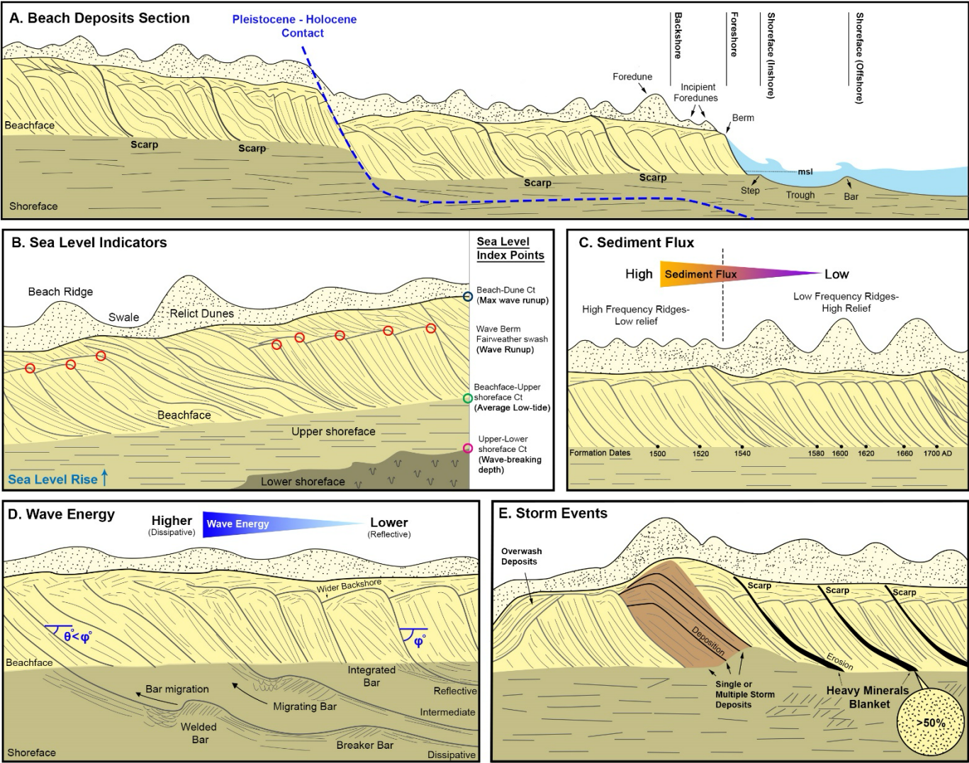
130 Figure 2. Idealized stratigraphic profiles showing common vertical plane geometries and the impact of varying climatic forcings on foreshore and shoreface deposits. A) Composite Holocene-Pleistocene beach deposit section, after Dougherty, 2018. MSL is mean sea level. B) Sea level rise, after Costas et al., 2016. Ct is contact. C) Sediment flux. D) Wave energy. E) Storm events.
