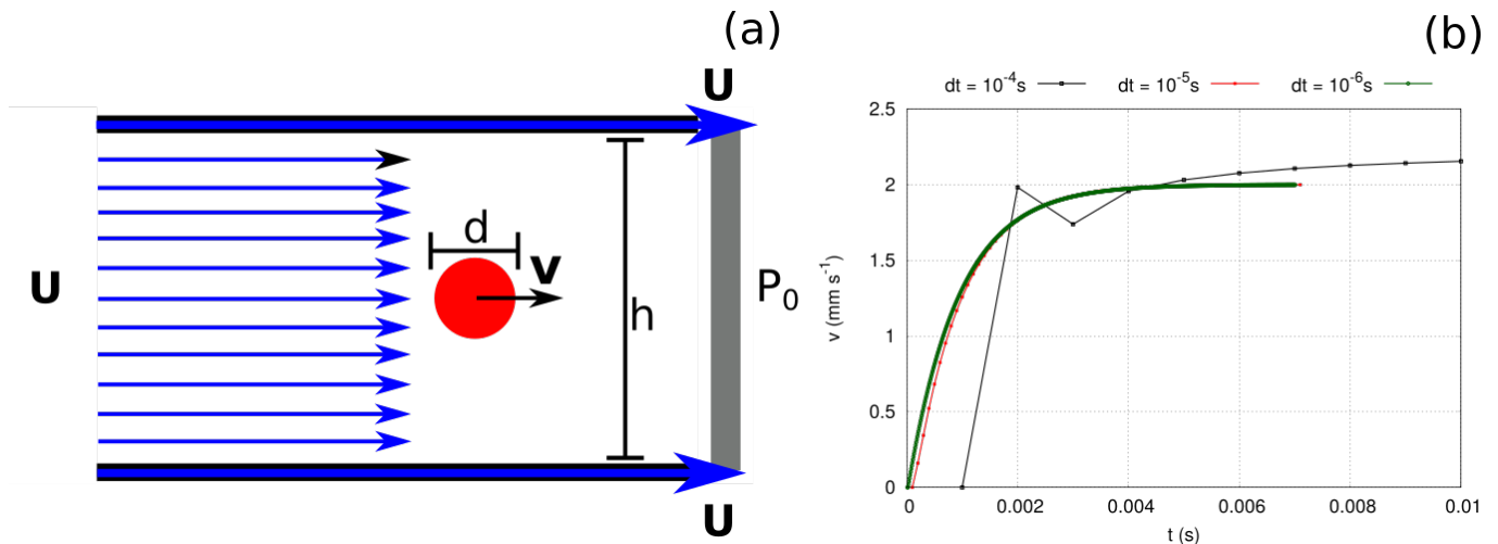
FIG. 6. (a) Lateral view of the system used to characterise particle movement due to fluid flow: a rectangular ( 3D ) cell with a fluid inlet velocity U = 2\text{mm s}^{-1} and h = 10\text{mm} . The lateral wall velocity is set equal to U to avoid changes in U due to finite size effects. A particle of d = 1\text{mm} is placed in the centre of the cell and its velocity, v , is recorded as a function of time. (b) Particle velocity v as a function of time for three different time-steps values. The CFD mesh has a resolution of 6 blocks per particle diameter.
