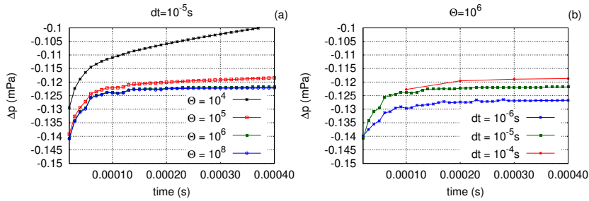
Fig. 4 Pressure drop through the porous material of Fig. 3 as a function of time for (a) different values of the parameter \Theta (Eq. (6)) and (b) different time steps dt .
