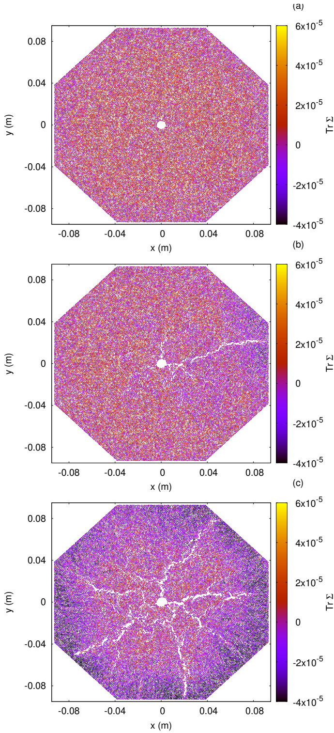
Fig. 8 (a) Numerical setup: N = 50000 spherical particles with sizes dispersed in the range of 1.8 - 0.9\text{mm} and a mean diameter \langle d_m \rangle = 1.35\text{mm} contained in an octagonal Hele-Shaw cell. Initial granular pack was created by compressing a loose granular material confined between two parallel plates (upper and lower plates) separated by a distance of about 2.5 times the mean particle diameter, confined by 8 piston like walls at a constant pressure until reach a mechanically stable static condition. Fluid is injected from the central hole at different pressures, (a) P_i = 8\text{kPa} (b) P_i = 22\text{kPa} (c) P_i = 28\text{kPa} . External pressure was set constant and a zero velocity boundary condition was set in the upper and lower plates. A low inter-particle cohesion interaction was simulated using a simplified Johnson-Kendall-Roberts model [19, 20] (with a cohesion energy density 300000\text{J/m}^3 ). Fluid density \rho = 1000\text{Kg/m}^3 , fluid viscosity \nu = 10\text{cp} .
