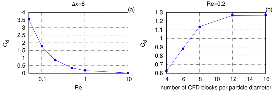
Fig. 7 Drag coefficient (for the setup represented in Fig. 6) for a particle forced to remain static (by external means) as a function of (a) Reynolds number ( Re ) and (b) mesh refinement.
