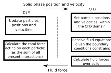
Fig. 1 CFDEM coupling procedure. In each time-step the DEM engine determines grains positions and velocities and send this information to the CFD engine. The CFD engine solves the fluid equations compatible with the given boundary conditions. Velocity and a pressure fields are obtained and forces F_g on each grain due to the fluid are calculated. F_g is sent to the DEM engine which adds it to the contact forces and any other grain interaction forces set within the DEM model and updates particle positions and velocities.
