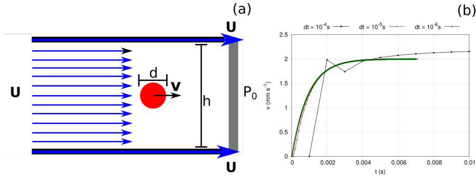
Fig. 6 (a) Lateral view of the system used to characterise particle movement due to fluid flow: a rectangular ( 3D ) cell with a fluid inlet velocity U = 2\text{mm s}^{-1} and h = 10\text{mm} . The lateral wall velocity is set equal to U to avoid changes in U due to finite size effects. A particle of d = 1\text{mm} is placed in the centre of the cell and its velocity, v , is recorded as a function of time. (b) Particle velocity v as a function of time for three different time-steps values. The CFD mesh has a resolution of 6 blocks per particle diameter.
