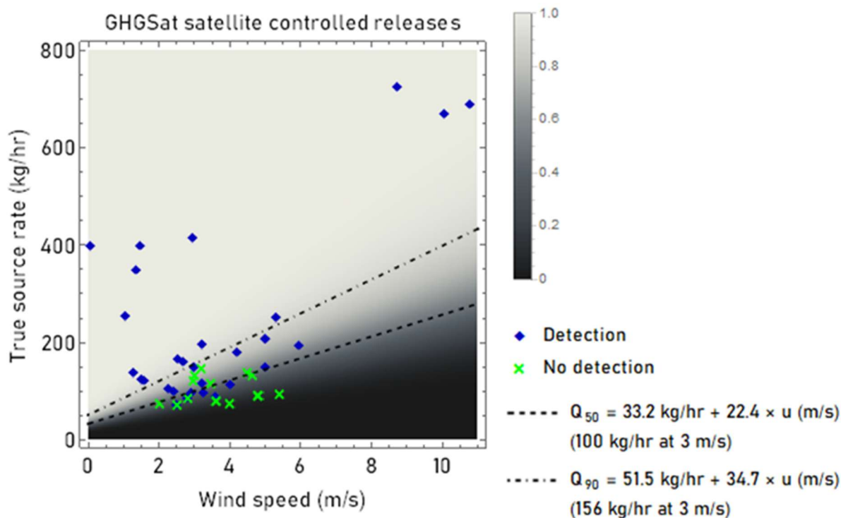
Figure 3: Regression analysis of detection limit from controlled releases measured by GHGSat's satellites (2020 - Aug 2023). The gray scale represents the probability of detection (colour bar). The lines give the best-fit thresholds Q_{50} and Q_{90} at each value of u .
