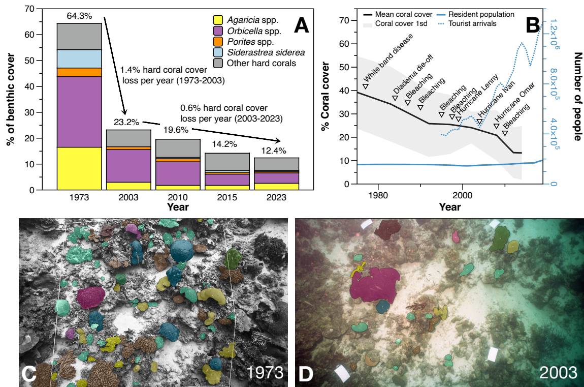
Figure 2. A) Changes in hard coral cover (%) and trends in hard coral cover loss (% year -1 ) from 1973 to 2023 at 10m depth on the shallow reefs of Curaçao. B) Time series of hard coral cover (%) from 1973 to 2014 based on permanent quadrats on the leeward coast of Curaçao (data from De Bakker et al., 2016(38)). The black line indicates the average % coral cover from four depths (10 m, 20 m, 30 m, and 40 m) each sampled at four sites and the gray band indicates 1 standard deviation of the mean; triangles above the line show major events affecting the Curaçao reefs. Blue lines show the number of tourist visits(34) (dotted line) and the resident population in Curaçao(33) (continuous line). C) and D) visual examples of hard coral cover in 1973 and 2003 of the same photo quadrat on Curaçao. Colors indicate different coral genera identifiable in the quadrats.
