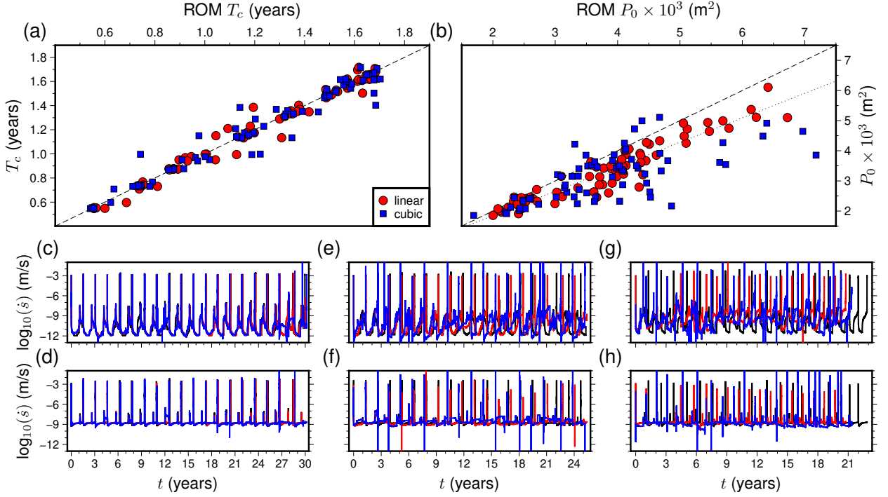
Figure S1. Comparison of the LOOCV results with linear (red) and cubic (blue) RBF interpolation kernels. (a) Comparison of FOM results versus ROM-predicted calculated recurrence time ( T_c ). The dashed line indicates a 1:1 ratio. (b) Comparison of FOM results versus ROM-predicted potency ( P_0 ). The dashed line indicates a 1:1 ratio and the dotted line shows the best linear fit between the linear-RBFs ROM and FOM datasets. (c)-(h) shows the same results as from Figure 9 (c)-(h) with FOM shown in black, ROM reconstruction using a linear RBF kernel (red) and ROM reconstruction using a cubic RBF kernel (blue).
