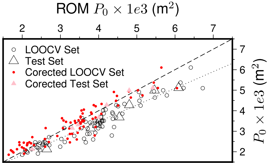
Figure S4. Effect of the linear post-processing correction on ROM-predicted SSEs potency ( P_0 ) when compared against Full Order Model (FOM) values. Results are shown for both the LOOCV dataset (circles), which were used to calculate the linear correction, and the independent test set (triangles). Dashed line indicates a 1:1 correspondence and dotted line best linear fit for the LOOCV not-corrected set.
