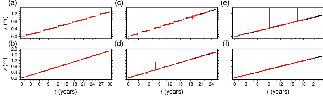
Figure S2. LOOCV comparison of cumulative slip predictions from the ROM (red curves) versus those from the FOM (black curves). Results are displayed for three different parameter sets at two along-dip observation points: 195 km (panels a, c, e) and 220 km (panels b, d, f). The parameter sets are: Panels (a,b): \mathbf{P}_1 using W = 37.375 km and \sigma_W = 5 MPa. Panels (c,d): \mathbf{P}_2 using W = 60.5 km and \sigma_W = 4 MPa. Panels (e,f): \mathbf{P}_3 using W = 43.0 km and \sigma_W = 3 MPa.
