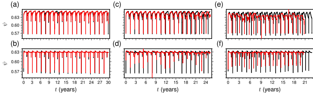
Figure S3. LOOCV comparison of state variable predictions from the ROM (red curves) versus those from the FOM (black curves). Results are displayed for three different parameter sets at two along-dip observation points: 195 km (panels a, c, e) and 220 km (panels b, d, f). The parameter sets are: Panels (a,b): \mathbf{P}_1 using W = 47.375 km and \sigma_W = 5 MPa. Panels (c,d): \mathbf{P}_2 using W = 60.5 km and \sigma_W = 4 MPa. Panels (e,f): \mathbf{P}_3 using W = 43.0 km and \sigma_W = 3 MPa.
