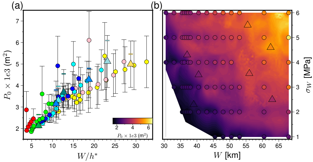
Figure S5. ROM predictions for uncorrected SSEs potency ( P_0 ). (a) Uncorrected SSE potency ( P_0 ) as a function of the normalized fault width ( W/h^* ). (b) Uncorrected SSE potency ( P_0 ) as a function of the width ( W , x-axis) and magnitude ( \sigma_W , y-axis) of the low effective normal stress zone. These are the raw ROM potency predictions before the linear correction detailed in Section 4.3 and shown in Figure 11.
