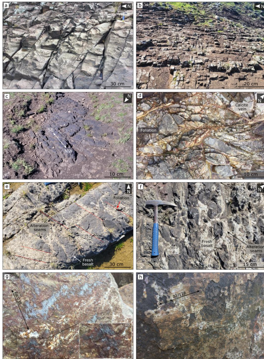
Figure 10. Deformational features in the field. (a) Irregular, nearly-vertical E-W striking structures (Fig. 3a). (b) Closely-spaced vertical E-W striking structures. (c) Closely-spaced NW-SE striking fractures along the Sarandí de Yí lineament (Fig. 4a). (d) Crackle basaltic breccia and fault gouge with apparent sinistral kinematics along bedrock exposure in the Lunarejo Valley (Fig. 3b). (e) Mosaic basaltic breccia and fault gouge along bedrock exposure along the Sarandí de Yí lineament (Fig. 4a). (f) Detailed features of fault gouge observed in (e), featuring alteration seams and fresh basaltic clasts (Fig. 4a). (g) High-plunging lineations in NW-SE-striking plane. (h) Nearly horizontal lineations in NW-SE-striking plane filled with calcite.
