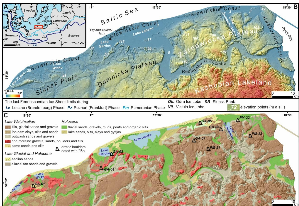
Fig. 1. Study area and location of large erratic boulders used in this study. (A) Location of the study area against the main limits of the last Fennoscandian Ice Sheet (FIS) and the main phases of the last deglaciation in north-central Europe. (B) Digital elevation model (DEM) of the study area with the main physiographic regions and selected elevation points. (C) Surface lithology of the study area based on Geological Map of Poland, 1:500 000 (Marks et al., 2006). Erratic boulders sampled for ^{10}\text{Be} surface exposure dating are also indicated.
