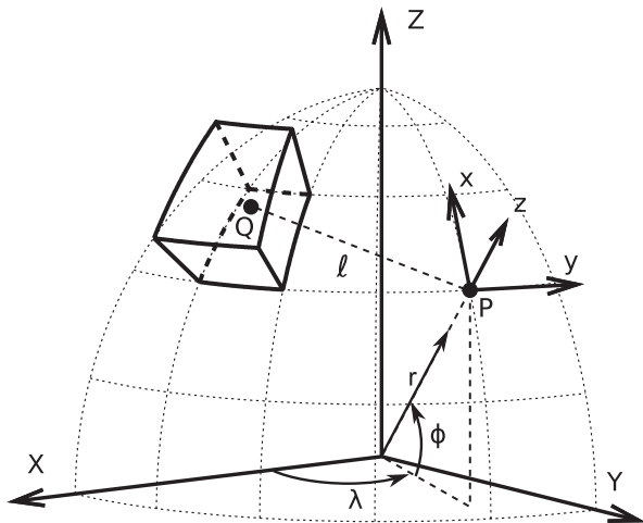
Figure 2. Sketch of a tesseroïd (spherical prism) in a geocentric coordinate system ( X, Y, Z ). Observations are made at point P with respect to its local north-oriented coordinate system ( x, y, z ). After Uieda (2015).
