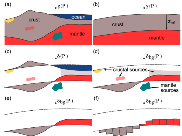
Figure 1. Sketch of the stages in gravity data correction and the discretization of the anomalous Moho relief using tesseroids. (a) The Earth and the measured gravity at point P ( g(P) ). (b) The Normal Earth and the calculated normal gravity at point P ( \gamma(P) ). z_{ref} is the depth of the Normal Earth Moho. (c) The gravity disturbance ( \delta(P) ) and the corresponding density anomalies after removal of the normal gravity: topography, oceans, crustal and mantle heterogeneities, and the anomalous Moho. (d) The Bouguer disturbance ( \delta_{bg}(P) ) after topographic correction and the remaining density anomalies. (e) All density anomalies save the anomalous Moho are assumed to have been removed before inversion. (f) The discretization of the anomalous Moho in tesseroids. Grey tesseroids will have a negative density contrast while red tesseroids will have a positive one.
