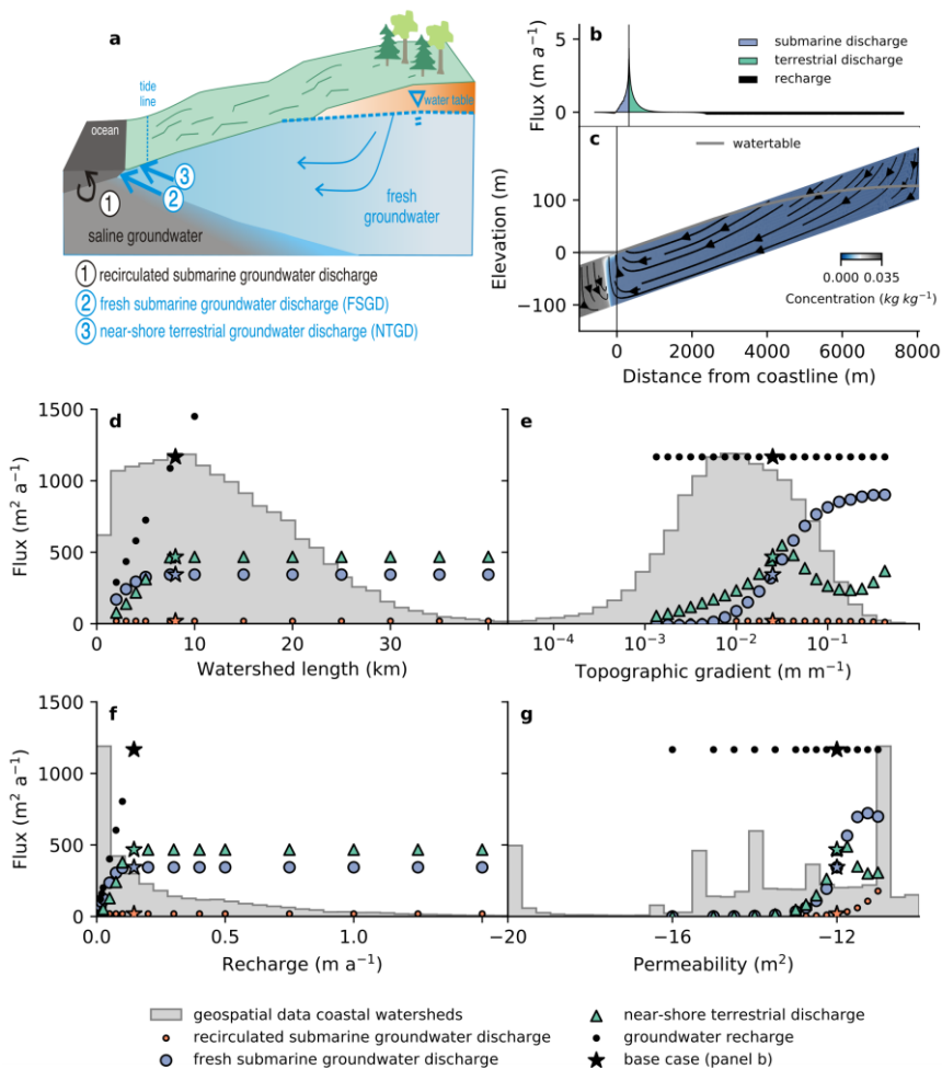
Fig. 1. Sensitivity analysis (d-g) of numerical models of coastal groundwater discharge (a-b) demonstrates that the flux of groundwater to the ocean is controlled primarily by topographic gradient (e) and aquifer permeability (g) and is relatively insensitive to watershed length (d) and groundwater recharge (f). The histograms in panels d-f show the distribution of the controlling parameters in all 40,082 global coastal watersheds. Panel b and c show modeled groundwater fluxes over the land surface and seabed (b), flowlines and salinity (c) for a base-case model coastal watershed with global median values for groundwater recharge ( 0.143 \text{ m a}^{-1} ), but with relatively high permeability ( 10^{-12} \text{ m}^2 ) and topographic gradient (2.5%).
