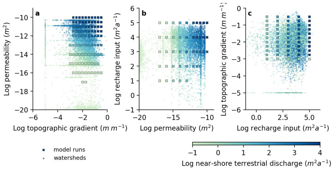
Fig. S9. Interpolation of near-shore terrestrial groundwater discharge (NGD) for each of the n=40082 coastal watersheds in our global database from n=351 model runs.
