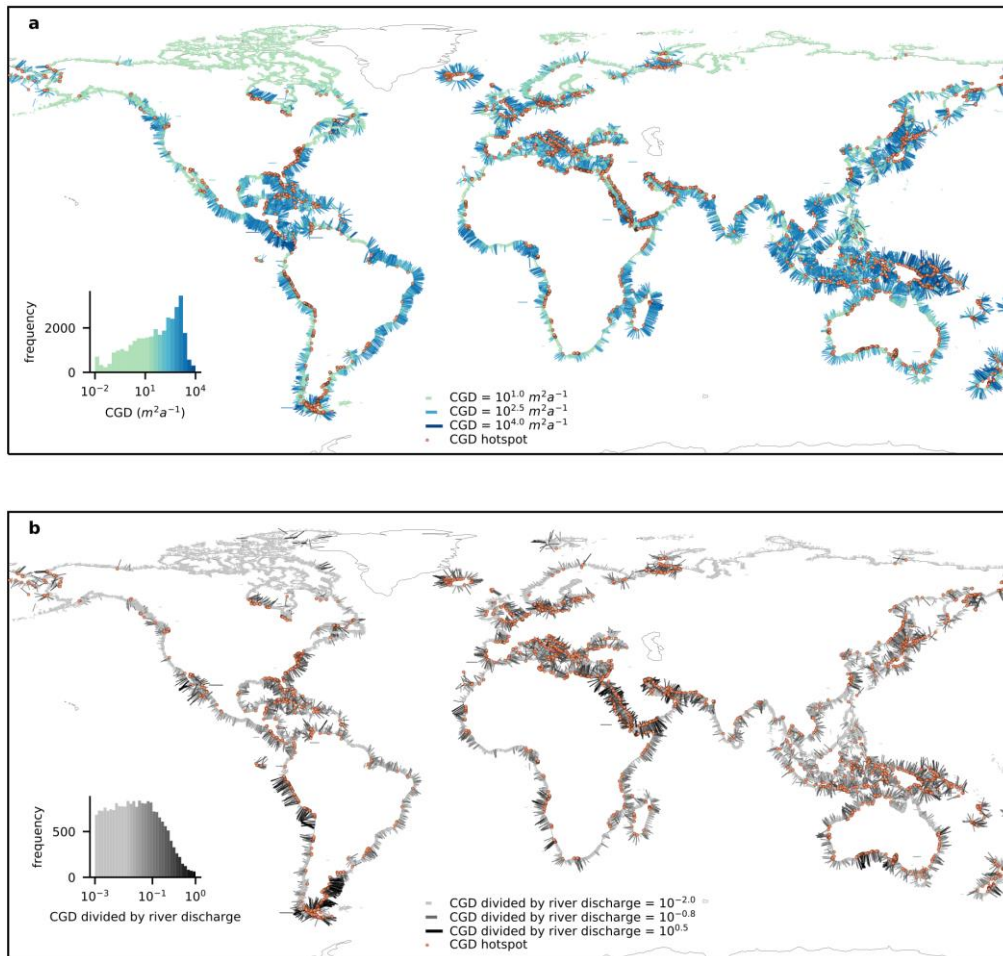
Fig. 3. The flow of groundwater to the oceans is highly variable, dominated by localized hotspots, and can locally be source of water that rivals surface water discharge. Global maps of a) coastal groundwater discharge (CGD) in m^2 a^{-1} and b) coastal groundwater discharge (CGD) divided by the surface water flux to the oceans.
