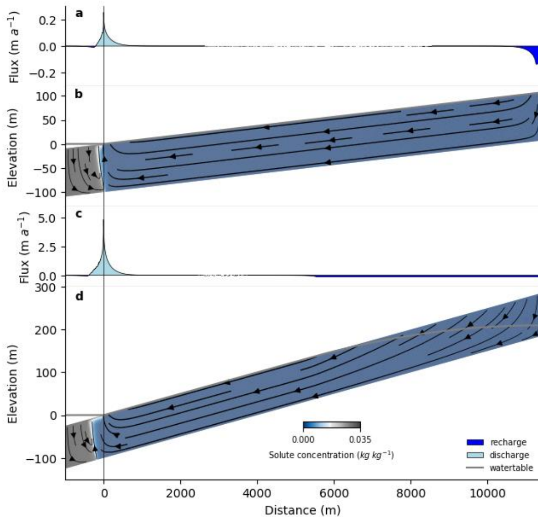
Fig. S13. Examples of modeled groundwater flow, salinity and distribution of terrestrial and submarine recharge and discharge for the median global watershed (panels a and b) and a model with a relatively high permeability ( 10^{-12} \text{ m}^2 ) and topographic gradient (2.5%) (c and d). The flux over the top surface (i.e., the land surface and the seabed) is shown in panel a and c, and shows the distribution of areas with groundwater recharge (dark blue), areas with zero or near-zero discharge where the applied recharge is balanced by discharge and a relatively small zone with significant terrestrial and marine groundwater discharge (light blue).
