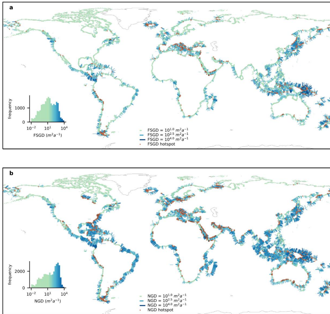
Fig. S14. Modeled fresh submarine groundwater discharge (a) and near-shore terrestrial groundwater discharge (b). Hotspots denote locations where the discharge flux exceeds 100 \text{ m}^2 \text{ a}^{-1} and 25% of the surface water flux to the oceans.
