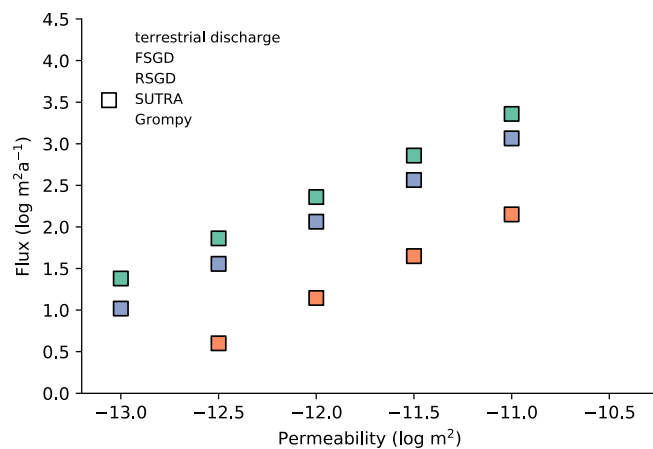
Fig. S5. Comparison of modeled fresh and recirculated submarine groundwater discharge and terrestrial discharge in a series of identical model experiments with the model codes GroMPy-couple and SUTRA. The model experiments used model domain size of 2.5 km onshore and 500 m offshore,
