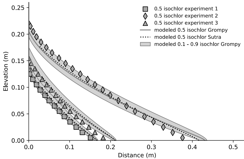
Fig. S2. Comparison of modeled position of a salt wedge by GroMPy-couple to the measured position in fresh and salt water flow experiments in porous media 37 . The modeled position of the fresh-salt water interface compares well to the measured values and is comparable to results for the widely used model code SUTRA 24 . The position of the salt wedge is equal to the location of the 50% salt water concentration contour line (0.5 isochlor).
