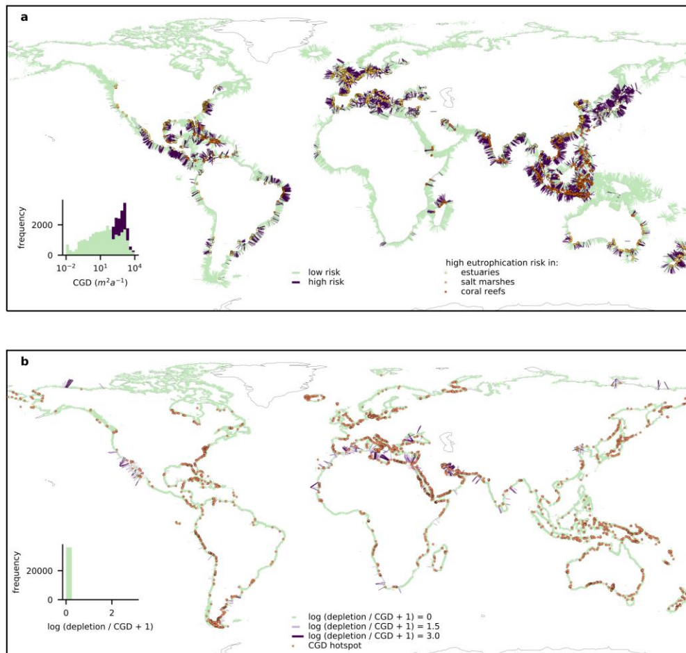
Fig. 4. Coastal groundwater discharge can locally pose a eutrophication and pollution risk to coastal ecosystems (panel a). Although the majority of coastal watersheds groundwater depletion is lower than coastal groundwater discharge, groundwater depletion locally exceeds coastal groundwater discharge in approximately 13% of the global coastline (panel b).
