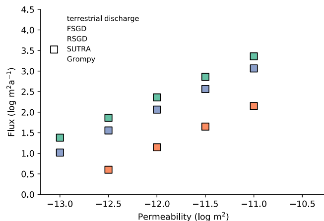
Fig. S5. Comparison of modeled fresh and recirculated submarine groundwater discharge and terrestrial discharge in a series of identical model experiments with the model codes GroMPy-couple and SUTRA. The model experiments used model domain size of 2.5 km onshore and 500 m offshore,
