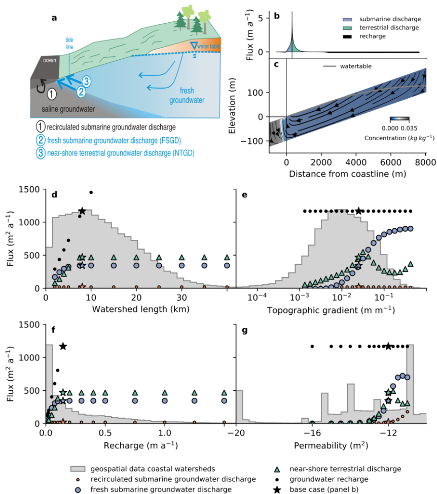
Fig. 1. Sensitivity analysis (d-g) of numerical models of coastal groundwater discharge (a-b) demonstrates that the flux of groundwater to the ocean is controlled primarily by topographic gradient (e) and aquifer permeability (g) and is relatively insensitive to watershed length (d) and groundwater recharge (f). The histograms in panels d-f show the distribution of the controlling parameters in all 40,082 global coastal watersheds. Panel b and c show modeled groundwater fluxes over the land surface and seabed (b), flowlines and salinity (c) for a base-case model coastal watershed with global median values for groundwater recharge ( 0.143 \text{ m a}^{-1} ), but with relatively high permeability ( 10^{-12} \text{ m}^2 ) and topographic gradient (2.5%).
